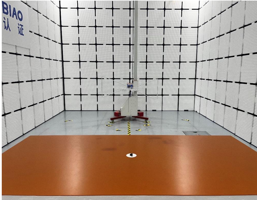
Radiated Emission Above 1GHz (Left ear)
