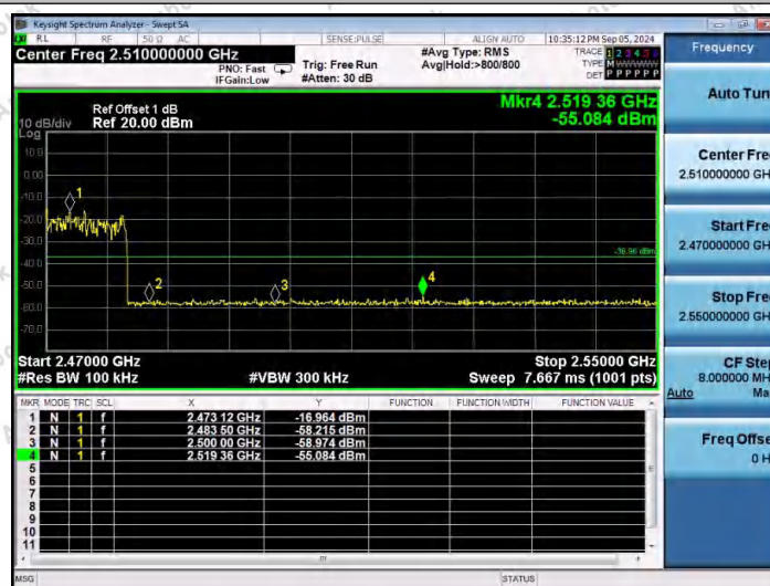
3DH5-Ant1-Hop_2480-PASS
