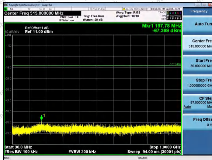
DH5-Ant1-2441-30~1000-PASS
