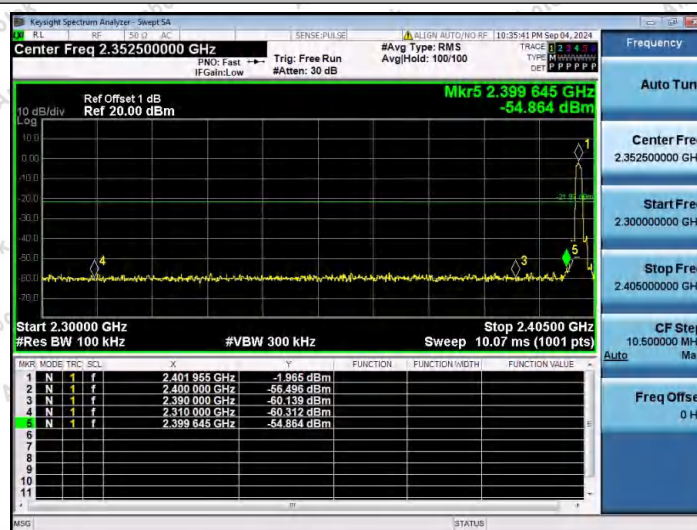
3DH5-Ant1-2402-PASS
