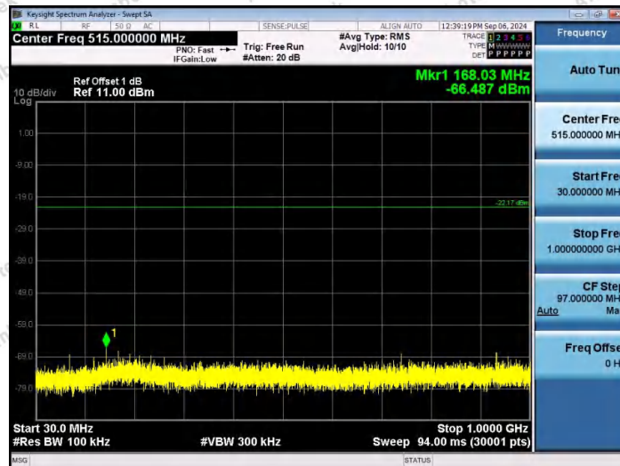
3DH5-Ant1-2402-30~1000-PASS
