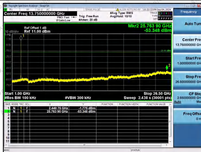
2DH5-Ant1-2441-1000~26500-PASS
