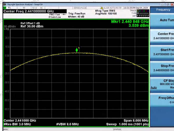
2DH5-Ant1-2441-PASS
