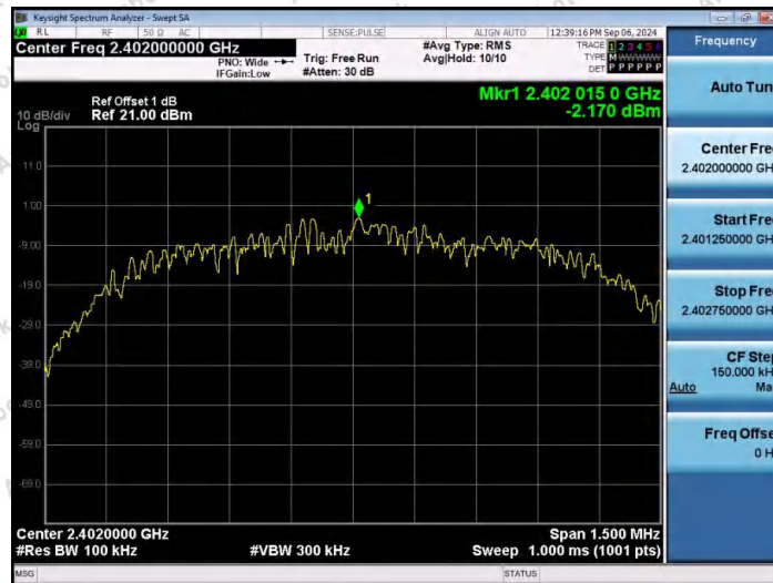
3DH5-Ant1-2402-0~Reference-PASS
