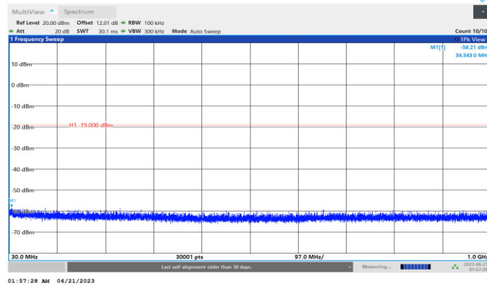
3DH5_Ant1_2480_30~1000
