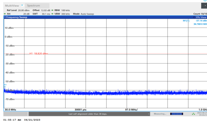
3DH5_Ant1_2402_30~1000
