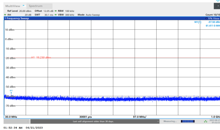
DH5_Ant1_2441_30-1000
