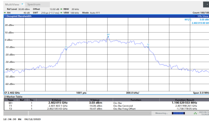
3DH5_Ant1_2402
