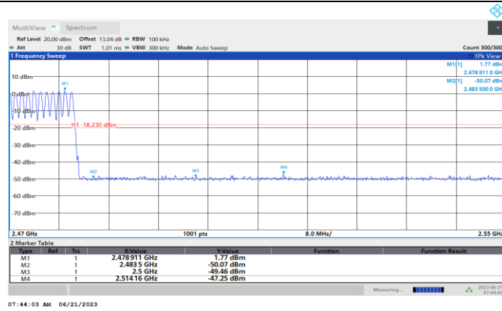
DH5_Ant1_High_Hop_2480
