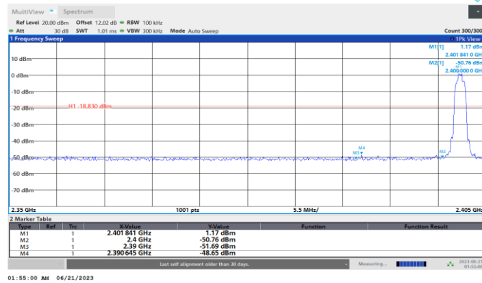
3DH5_Ant1_Low_2402
