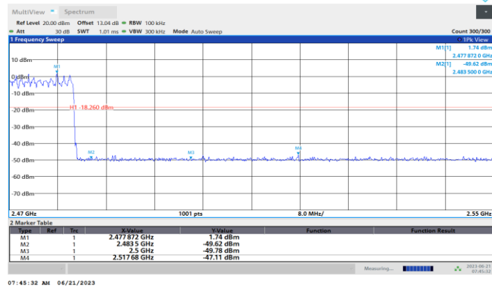
3DH5_Ant1_High_Hop_2480
