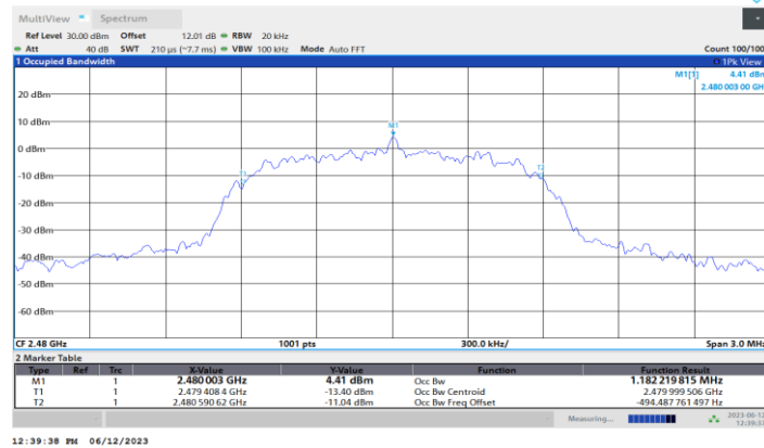
3DH5_Ant1_2480
