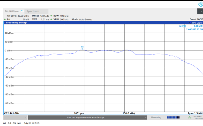
3DH5_Ant1_2441_0~Reference
