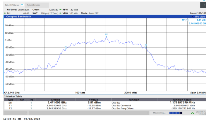
3DH5_Ant1_2441
