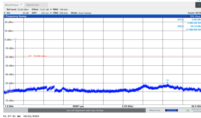
3DH5_Ant1_2480_1000~26500
