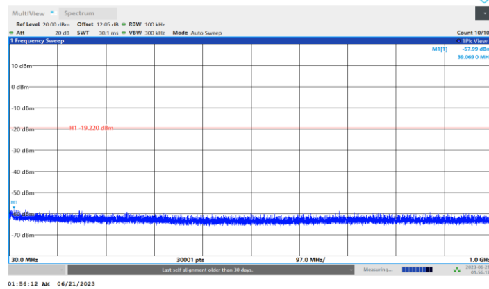
3DH5_Ant1_2441_30~1000
