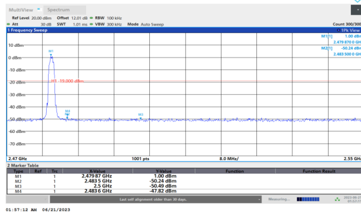
3DH5_Ant1_High_2480
