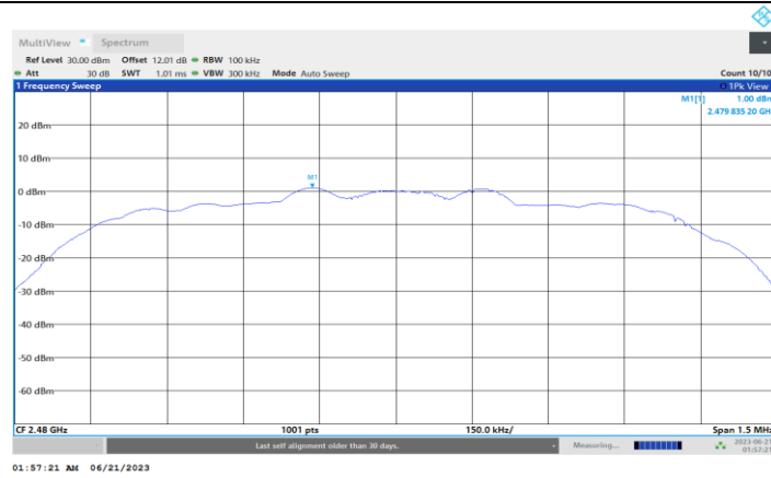
3DH5_Ant1_2480_0~Reference
