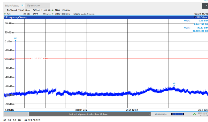
DH5_Ant1_2441_1000-26500
