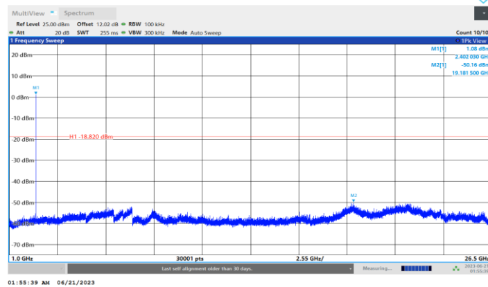
3DH5_Ant1_2402_1000~26500
