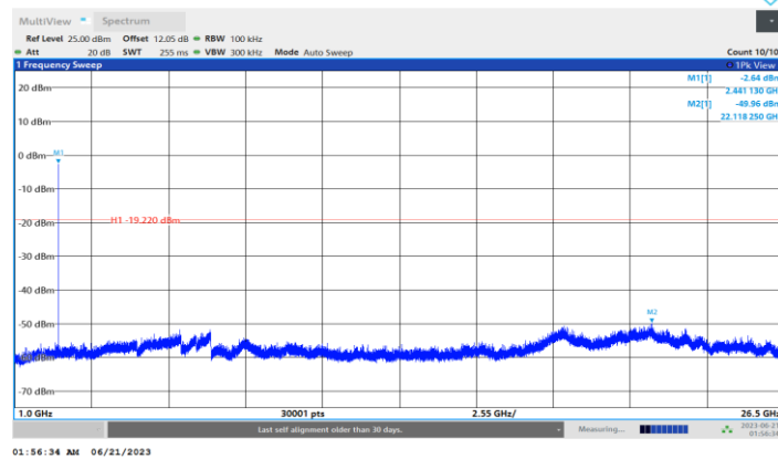
3DH5_Ant1_2441_1000~26500
