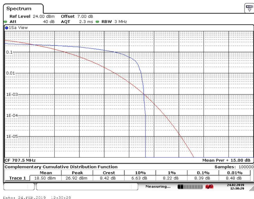
Peak-Average Ratio Plot(5MHz BW,16QAM,Band 12-mid Channel)
