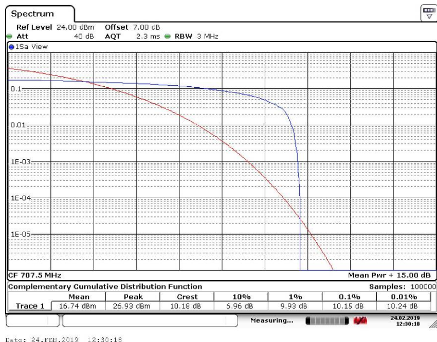
Peak-Average Ratio Plot(5MHz BW,QPSK,Band 12-mid Channel)
