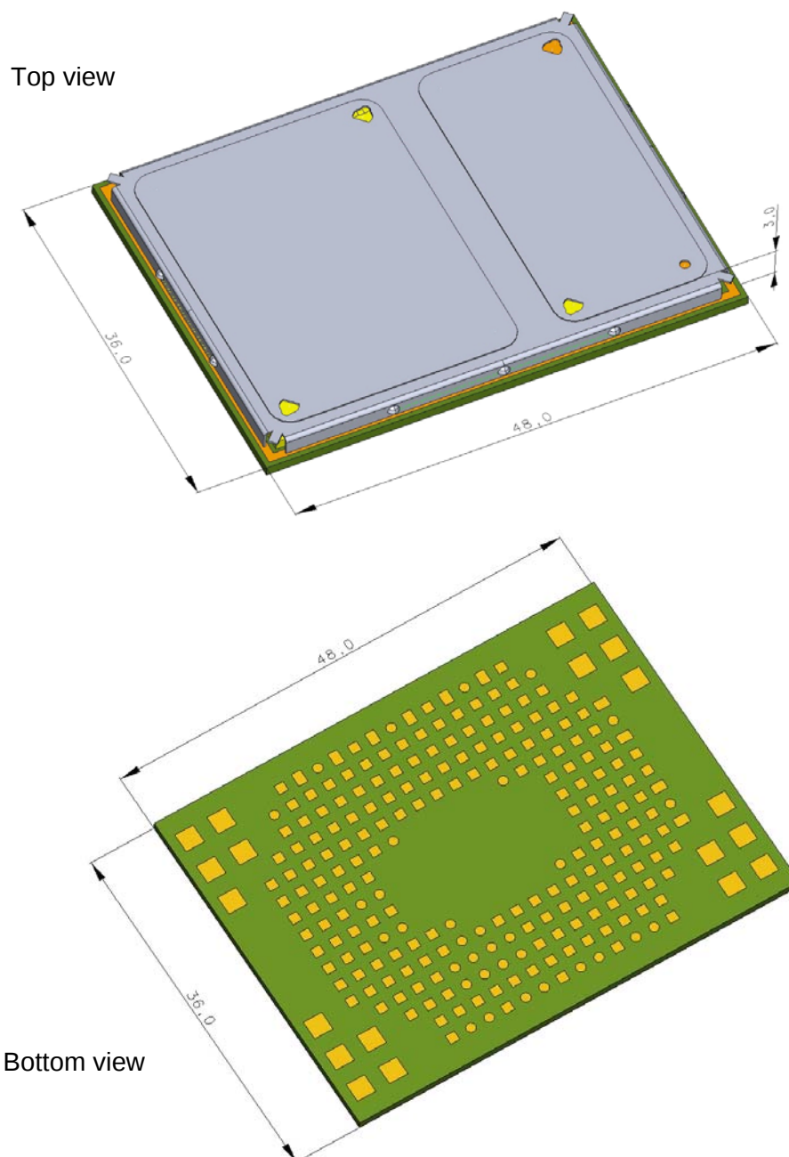
Figure 14: ALAS66A – top and bottom view
