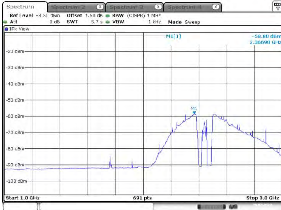
Plot on Configuration VHT40 / 2437 MHz / Average / Port 2 / 1GHz~3GHz
