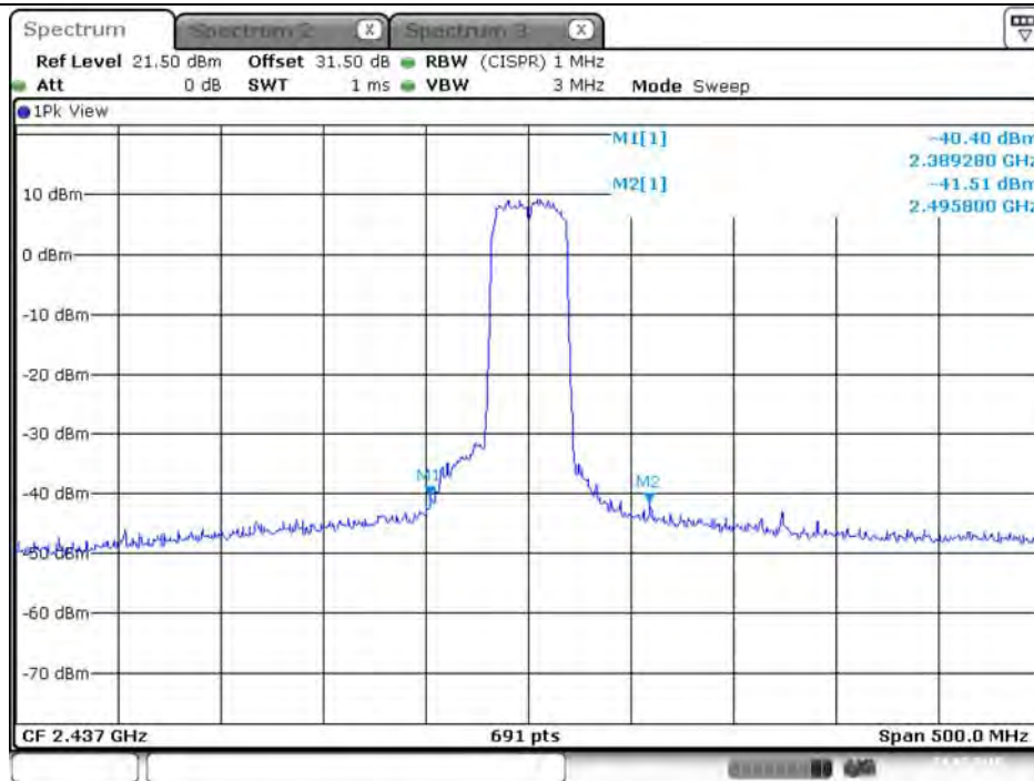
Plot on Configuration VHT40 / 2437 MHz / Peak / Port 1 (TX1)
