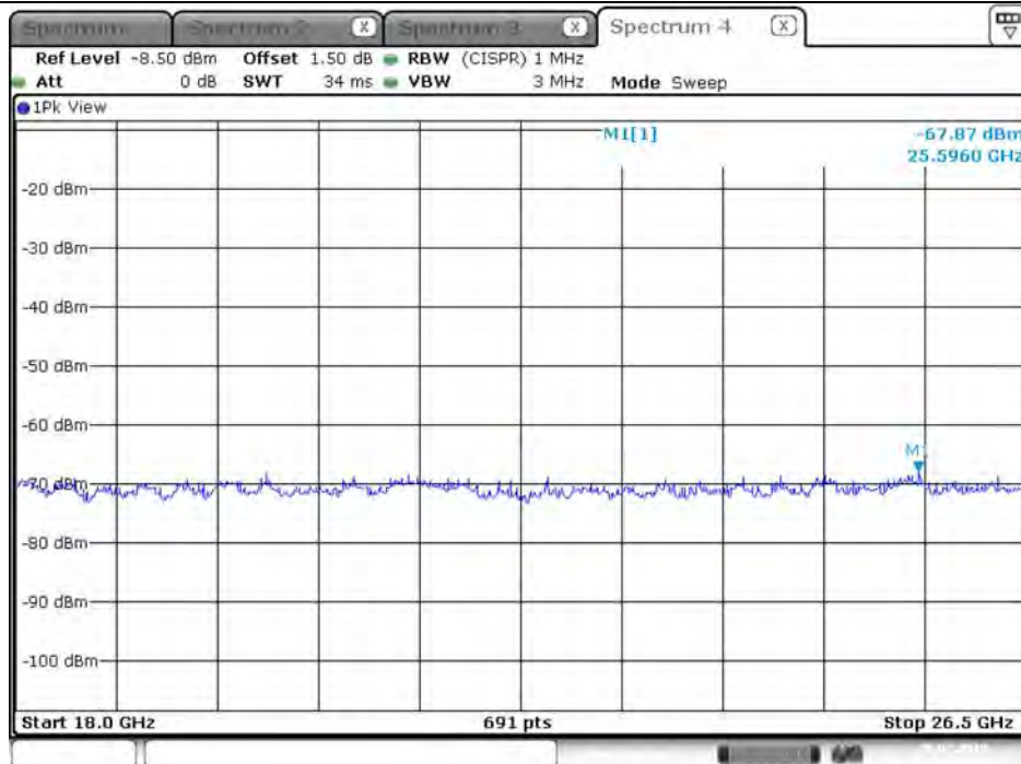
Plot on Configuration VHT20 / 2462 MHz / Peak / Port 1 / 18GHz~26.5GHz
