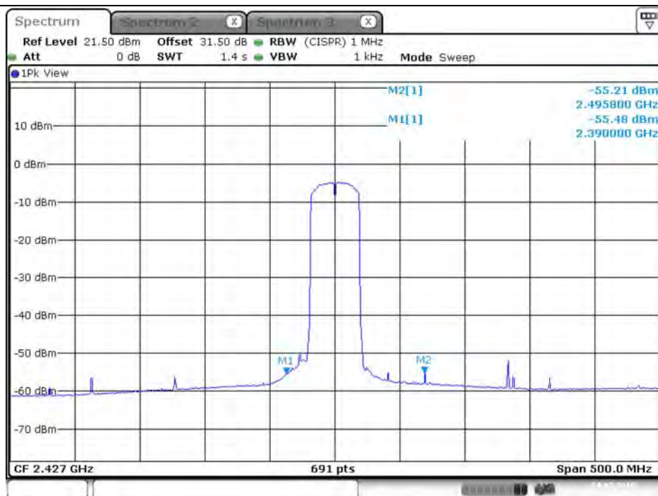
Plot on Configuration VHT40 / 2427 MHz / Average / Port 1 (TX1)
