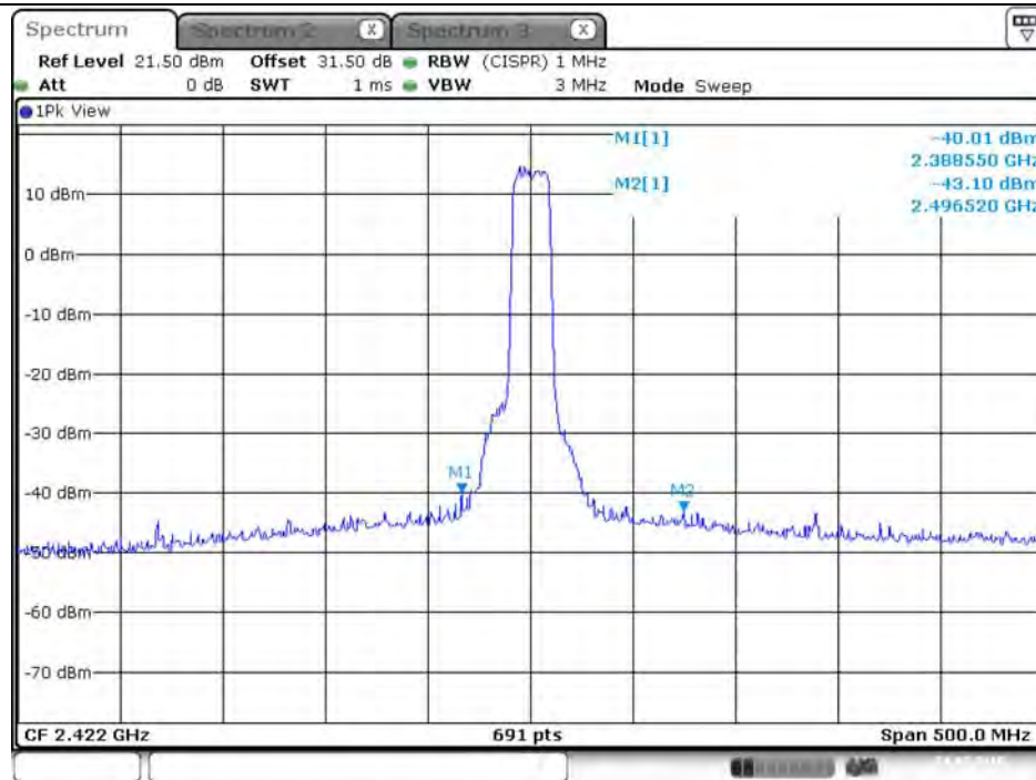
Plot on Configuration VHT20 / 2422 MHz / Peak / Port 1 (TX1)
