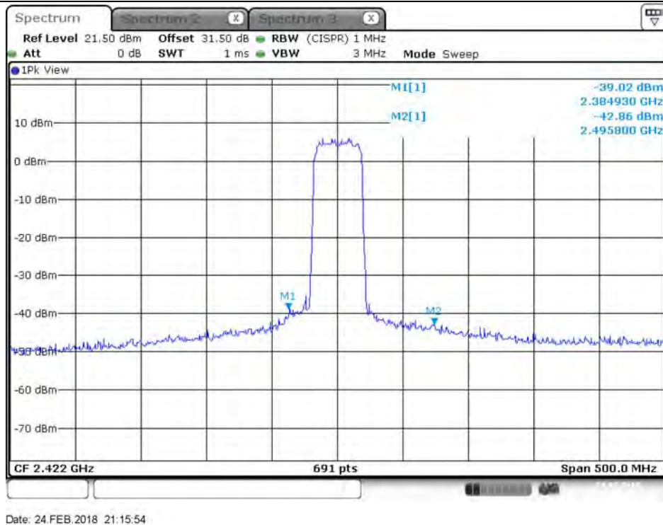
Plot on Configuration VHT40 / 2422 MHz / Peak / Port 2 (TX2)
