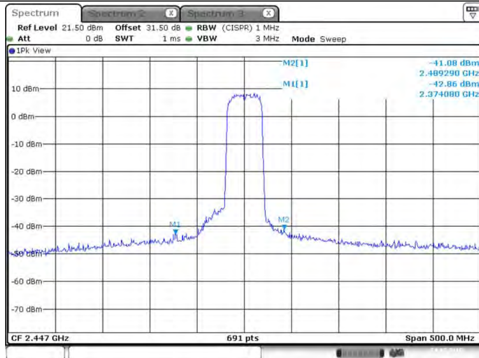
Plot on Configuration VHT40 / 2447 MHz / Peak / Port 2 (TX2)
