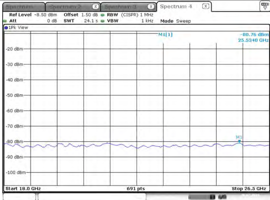
Plot on Configuration VHT20 / 2412 MHz / Average / Port 2 / 18GHz~26.5GHz
