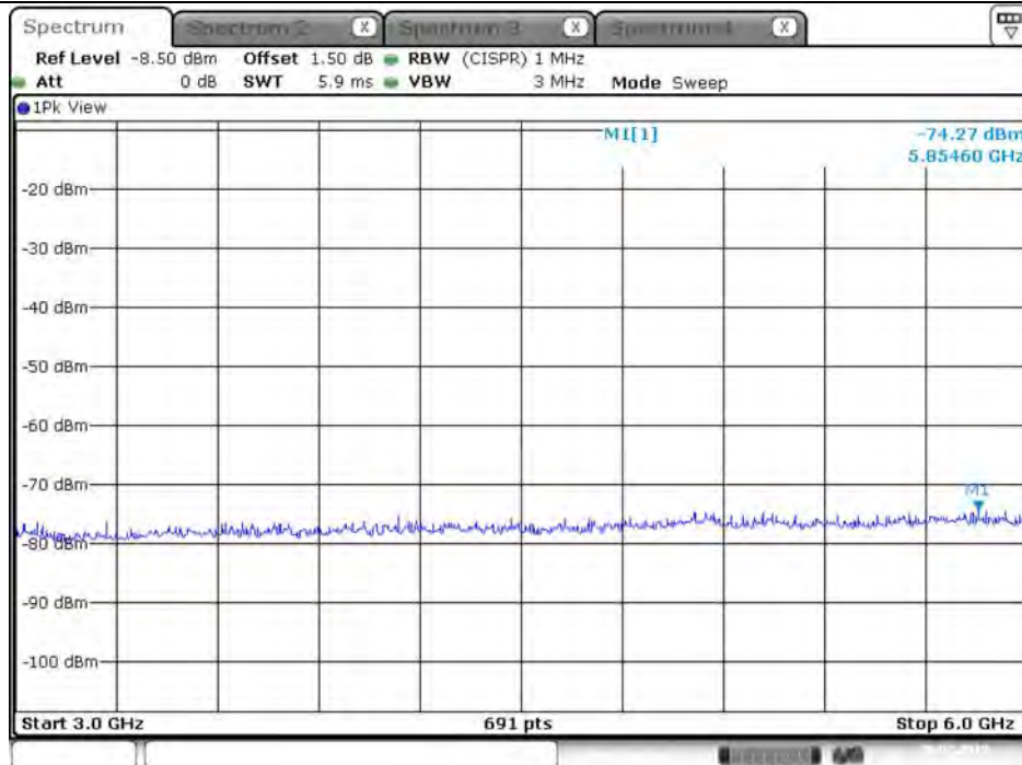
Plot on Configuration VHT40 / 2452 MHz / Peak / Port 1 / 3GHz~6GHz
