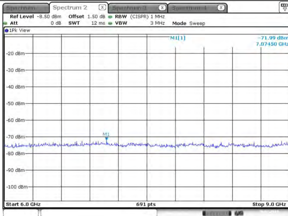
Plot on Configuration VHT20 / 2437 MHz / Peak / Port 1 / 6GHz~9GHz
