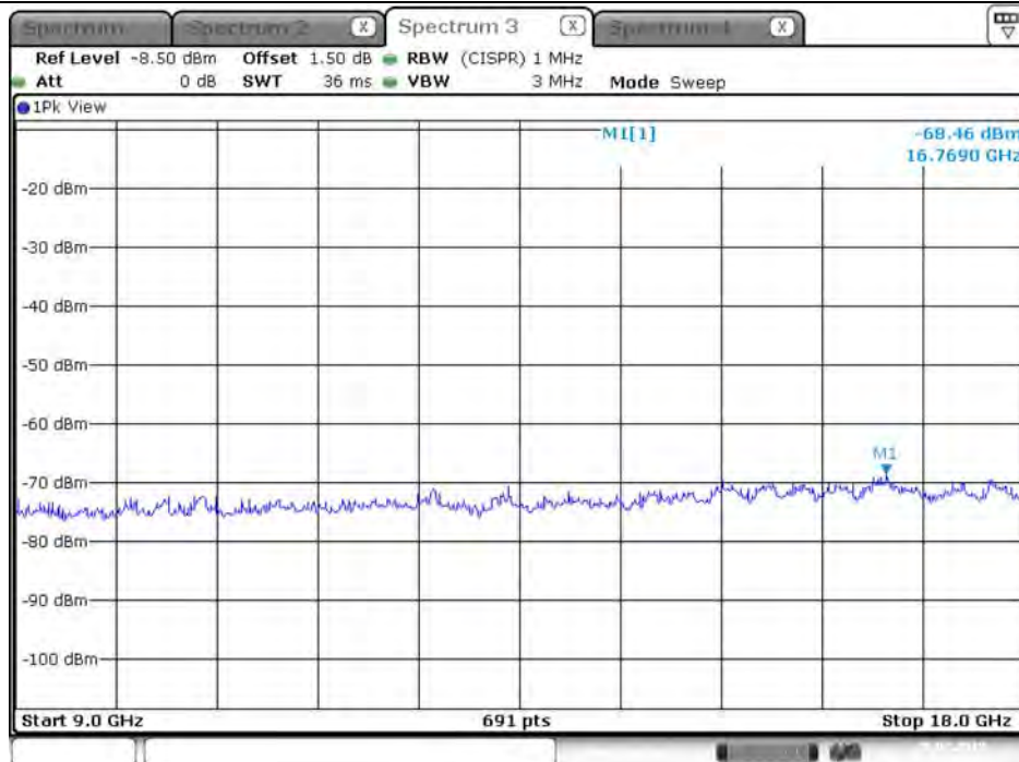
Plot on Configuration VHT40 / 2422 MHz / Peak / Port 1 / 9GHz~18GHz
