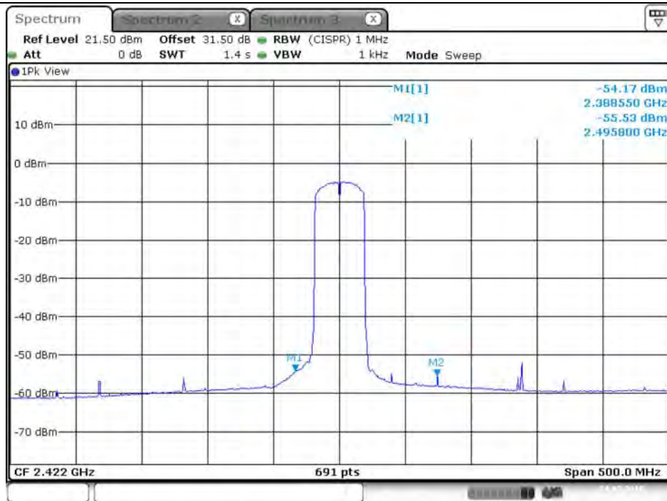
Plot on Configuration VHT40 / 2422 MHz / Average / Port 1 (TX1)
