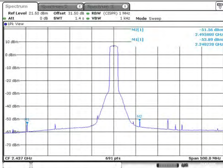
Plot on Configuration VHT20 / 2437 MHz / Average / Port 1 (TX1)
