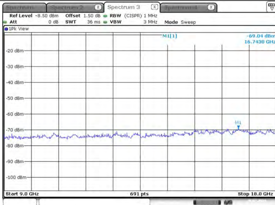
Plot on Configuration VHT20 / 2437 MHz / Peak / Port 1 / 9GHz~18GHz
