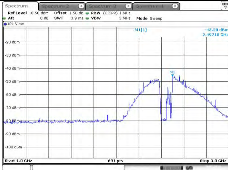
Plot on Configuration VHT40 / 2452 MHz / Peak / Port 1 / 1GHz~3GHz
