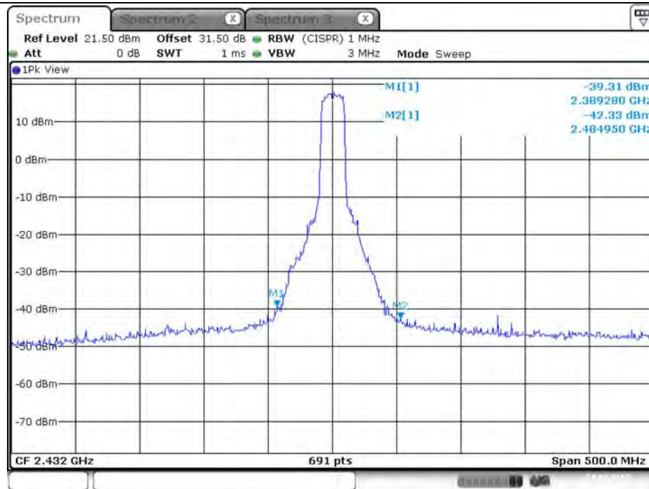
Plot on Configuration VHT20 / 2432 MHz / Peak / Port 1 (TX1)
