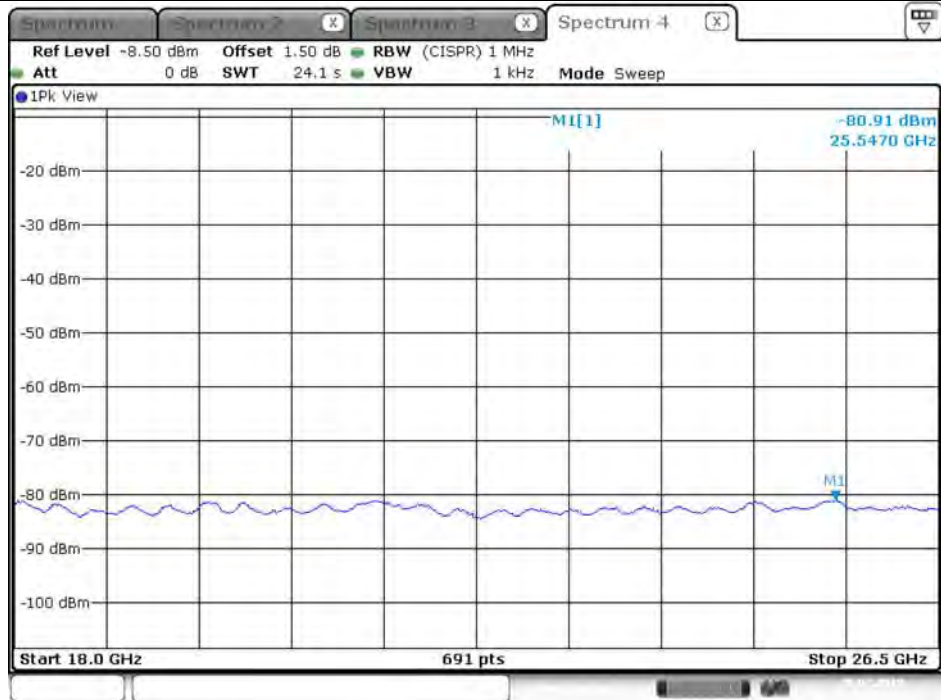
Plot on Configuration VHT20 / 2462 MHz / Average / Port 1 / 18GHz~26.5GHz
