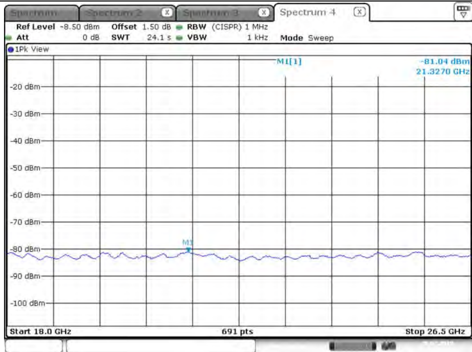
Plot on Configuration VHT20 / 2412 MHz / Average / Port 1 / 18GHz~26.5GHz
