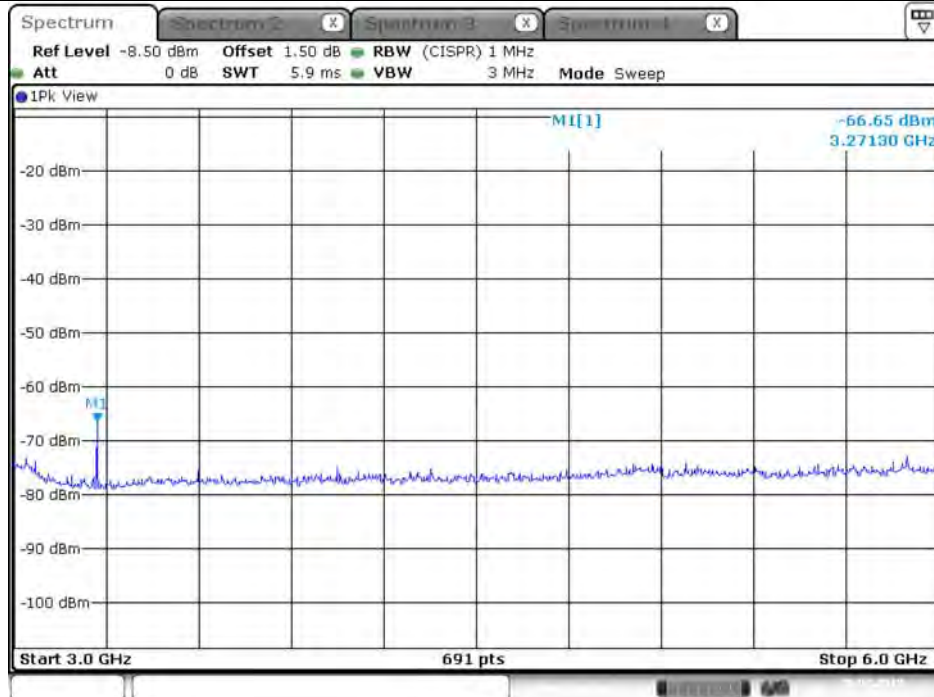
Plot on Configuration VHT40 / 2452 MHz / Peak / Port 2 / 3GHz~6GHz
