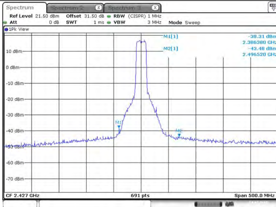
Plot on Configuration VHT20 / 2427 MHz / Peak / Port 2 (TX2)
