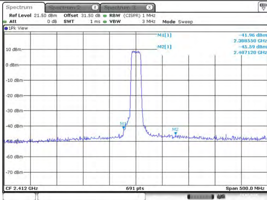
Plot on Configuration VHT20 / 2412 MHz / Peak / Port 2 (TX2)
