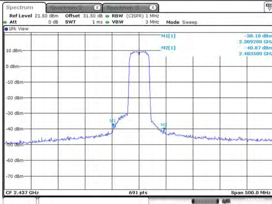
Plot on Configuration VHT40 / 2437 MHz / Peak / Port 2 (TX2)
