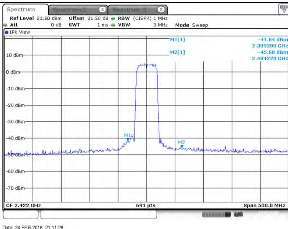
Plot on Configuration VHT40 / 2422 MHz / Peak / Port 1 (TX1)
