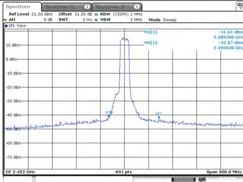
Plot on Configuration VHT20 / 2422 MHz / Peak / Port 2 (TX2)
