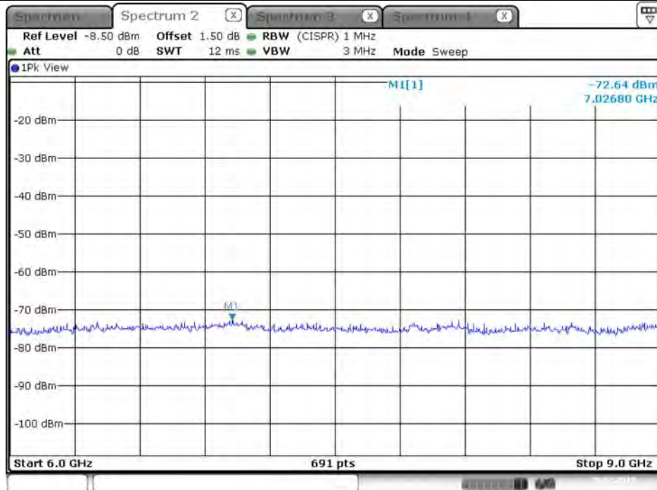
Plot on Configuration VHT40 / 2452 MHz / Peak / Port 2 / 6GHz~9GHz
