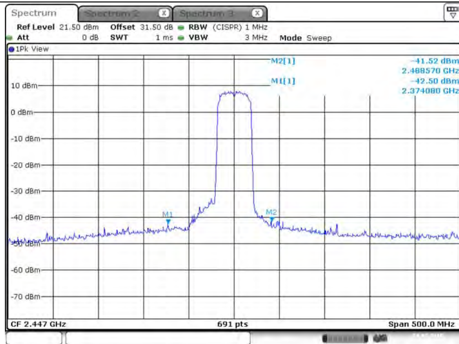
Plot on Configuration VHT40 / 2447 MHz / Peak / Port 1 (TX1)
