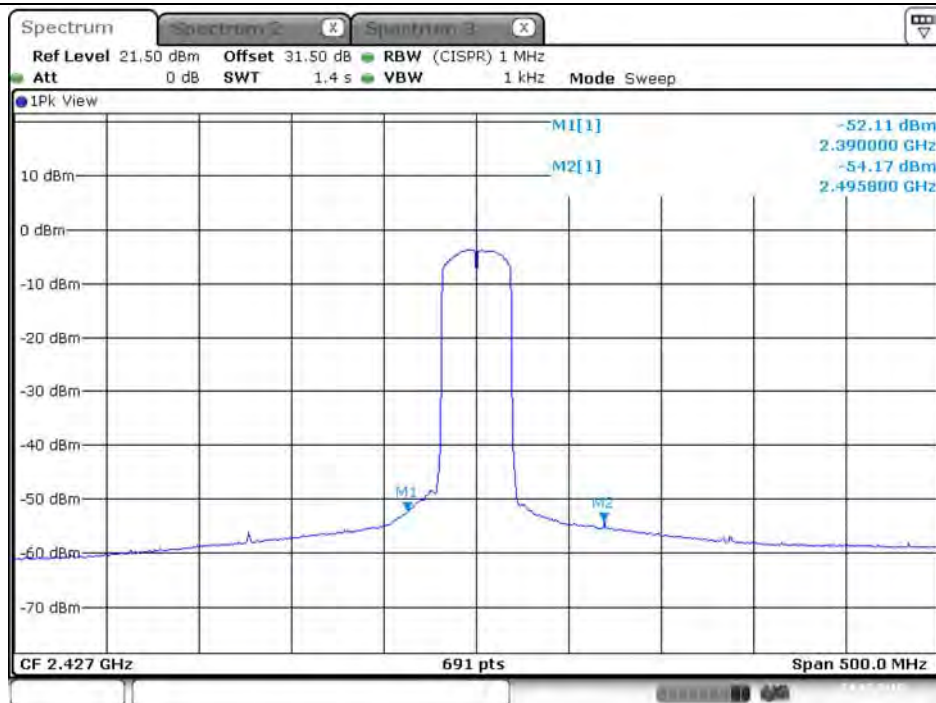
Plot on Configuration VHT40 / 2427 MHz / Average / Port 2 (TX2)
