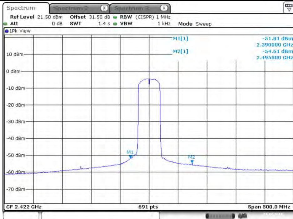
Plot on Configuration VHT40 / 2422 MHz / Average / Port 2 (TX2)
