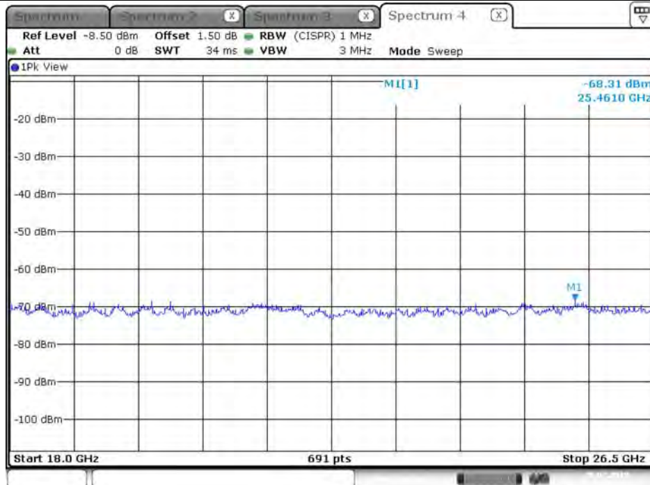
Plot on Configuration VHT20 / 2462 MHz / Peak / Port 2 / 18GHz~26.5GHz
