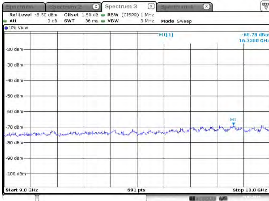
Plot on Configuration VHT40 / 2422 MHz / Peak / Port 2 / 9GHz~18GHz
