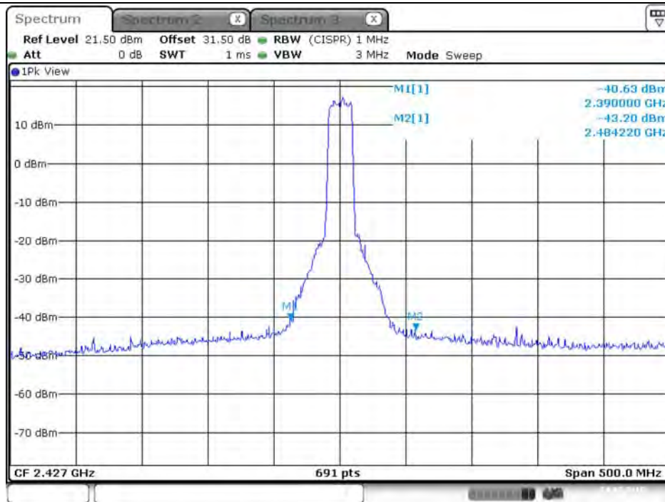
Plot on Configuration VHT20 / 2427 MHz / Peak / Port 1 (TX1)
