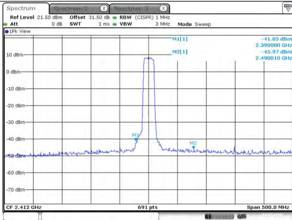
Plot on Configuration VHT20 / 2412 MHz / Peak / Port 1 (TX1)
