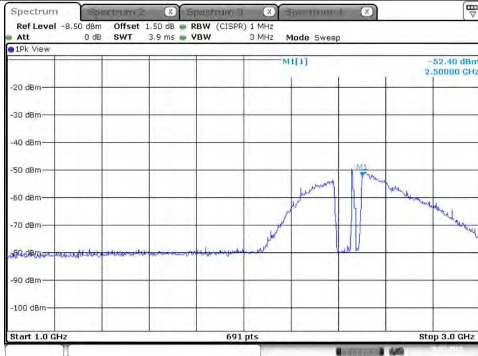
Plot on Configuration VHT20 / 2462 MHz / Peak / Port 2 / 1GHz~3GHz
