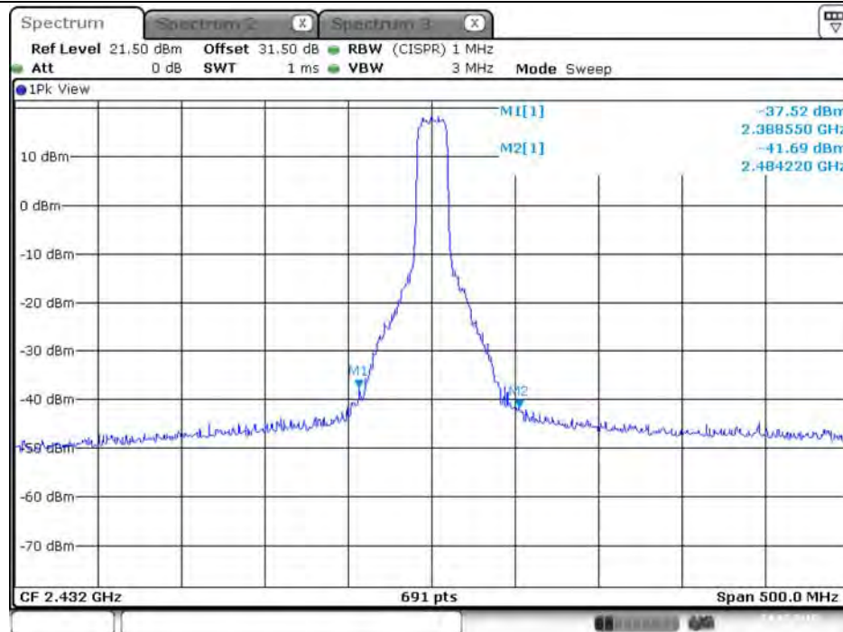
Plot on Configuration VHT20 / 2432 MHz / Peak / Port 2 (TX2)
