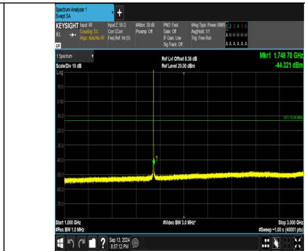
Band66_1.4MHz_QPSK_132322_1RB#5_1000~3000_1000~3000
