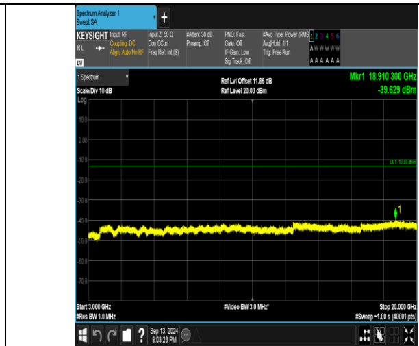
Band66_1.4MHz_16QAM_132665_1RB#5_3000~20000_3000~20000
