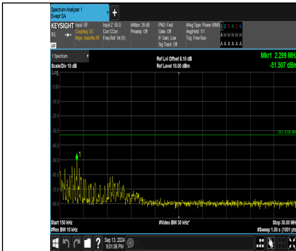
Band66_1.4MHz_16QAM_132665_1RB#0_0.15~30_0.15~30
