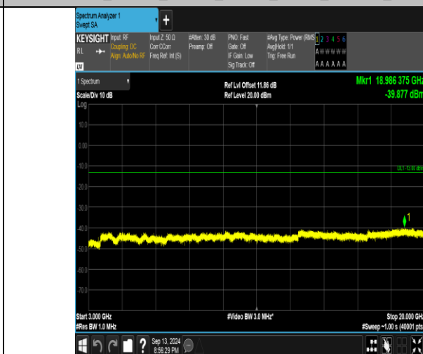
Band66_1.4MHz_16QAM_132322_1RB#0_3000~20000_3000~20000
