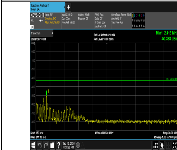
Band66_1.4MHz_16QAM_132322_6RB#0_0.15~30_0.15~30
