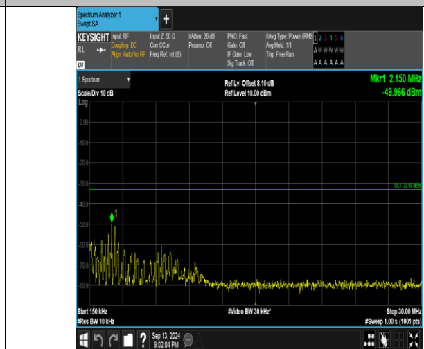
Band66_1.4MHz_QPSK_132665_1RB#5_0.15~30_0.15~30
