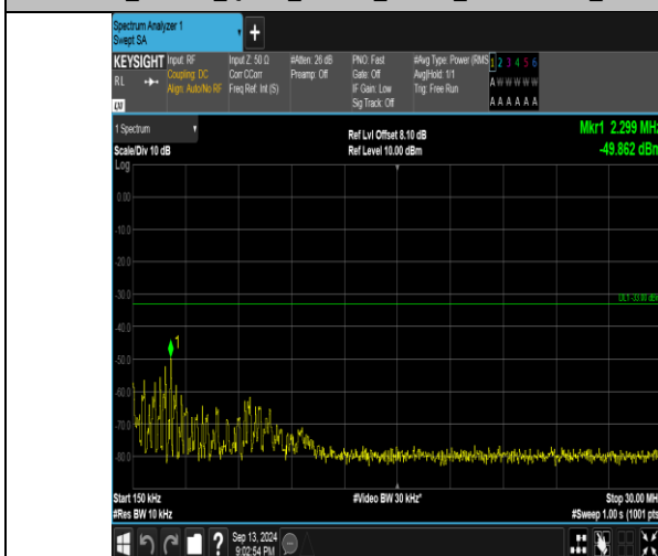
Band66_1.4MHz_16QAM_132665_1RB#5_0.15~30_0.15~30
