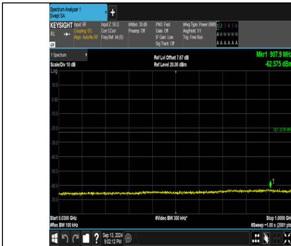
Band66_1.4MHz_QPSK_132665_1RB#5_30~1000_30~1000
