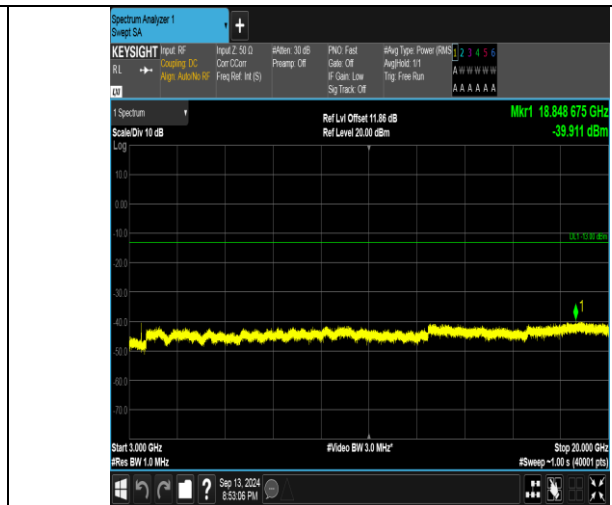
Band66_1.4MHz_16QAM_131979_1RB#5_3000~20000_3000~20000
