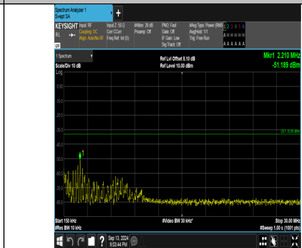
Band66_1.4MHz_QPSK_132665_6RB#0_0.15~30_0.15~30
