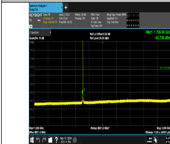
Band66_1.4MHz_16QAM_131979_1RB#0_1000~3000_1000~3000
