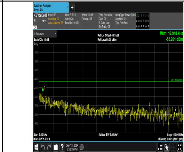
Band66_1.4MHz_16QAM_131979_1RB#5_0.009~0.15_0.009~0.15
