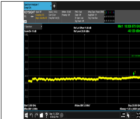
Band66_1.4MHz_QPSK_132322_6RB#0_3000~20000_3000~20000
