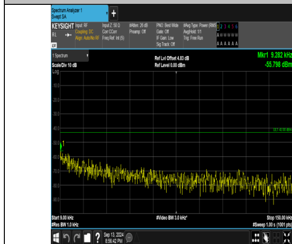
Band66_1.4MHz_QPSK_132322_1RB#5_0.009~0.15_0.009~0.15
