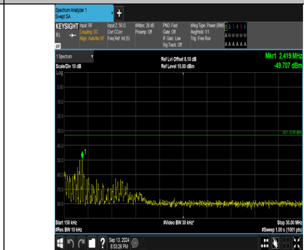
Band66_1.4MHz_QPSK_131979_6RB#0_0.15~30_0.15~30
