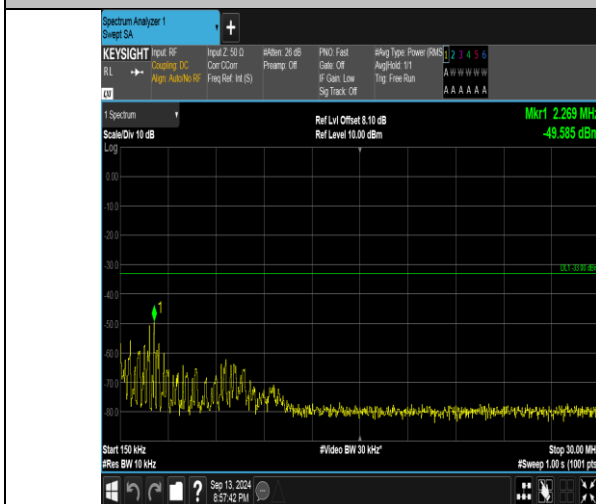
Band66_1.4MHz_16QAM_132322_1RB#5_0.15~30_0.15~30
