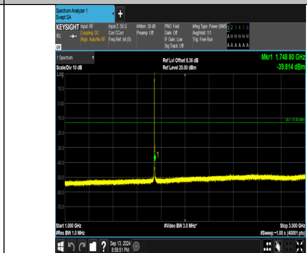
Band66_1.4MHz_QPSK_132322_6RB#0_1000~3000_1000~3000
