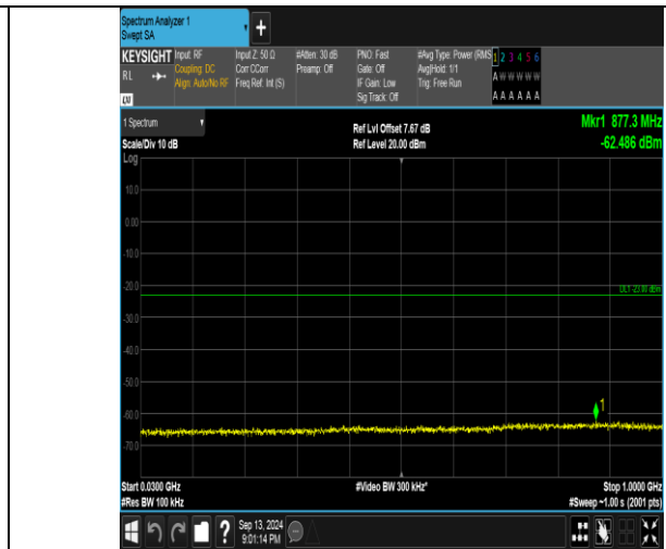
Band66_1.4MHz_16QAM_132665_1RB#0_30~1000_30~1000
