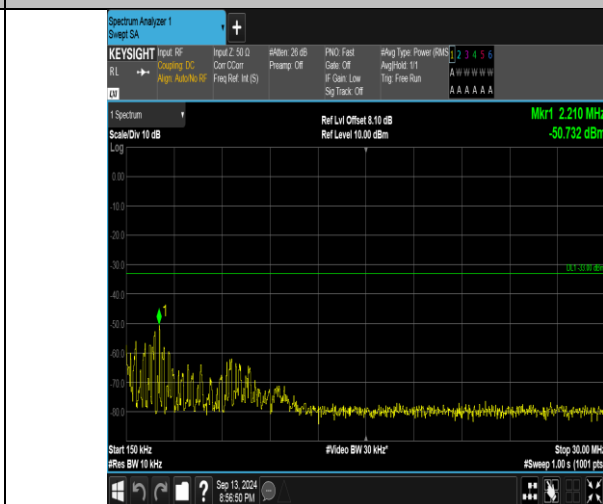
Band66_1.4MHz_QPSK_132322_1RB#5_0.15~30_0.15~30
