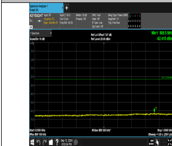
Band66_1.4MHz_QPSK_131979_6RB#0_30~1000_30~1000
