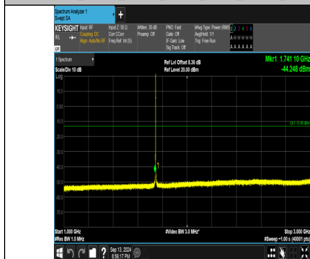
Band66_1.4MHz_16QAM_132322_1RB#0_1000~3000_1000~3000
