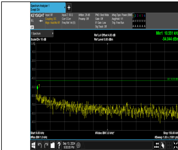
Band66_1.4MHz_QPSK_132665_1RB#0_0.009~0.15_0.009~0.15
