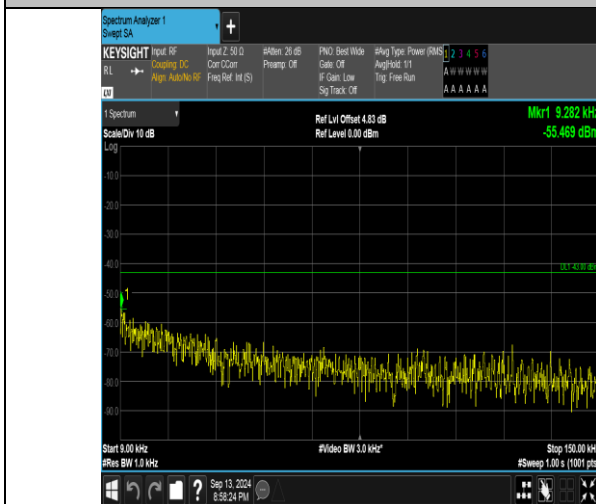
Band66_1.4MHz_QPSK_132322_6RB#0_0.009~0.15_0.009~0.15
