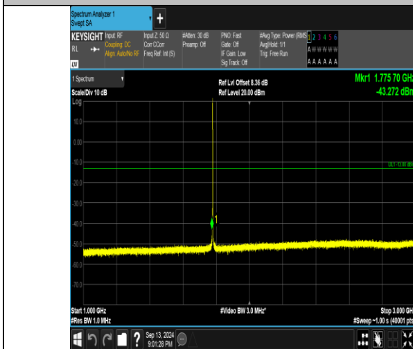
Band66_1.4MHz_16QAM_132665_1RB#0_1000~3000_1000~3000
