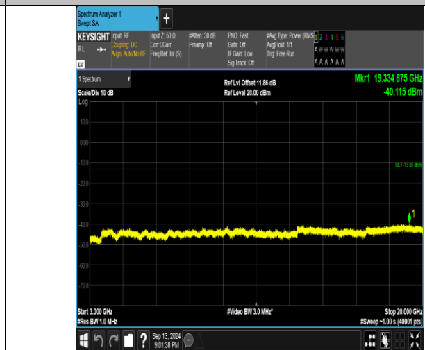
Band66_1.4MHz_16QAM_132665_1RB#0_3000~20000_3000~20000
