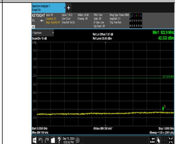
Band66_1.4MHz_16QAM_131979_1RB#5_30~1000_30~1000
