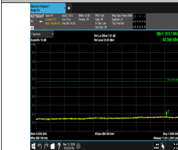
Band66_1.4MHz_QPSK_132665_6RB#0_30~1000_30~1000
