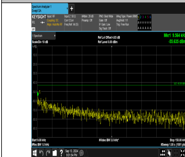
Band66_1.4MHz_QPSK_132665_1RB#5_0.009~0.15_0.009~0.15
