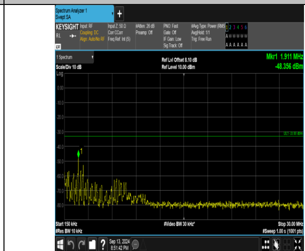
Band66_1.4MHz_QPSK_131979_1RB#5_0.15~30_0.15~30
