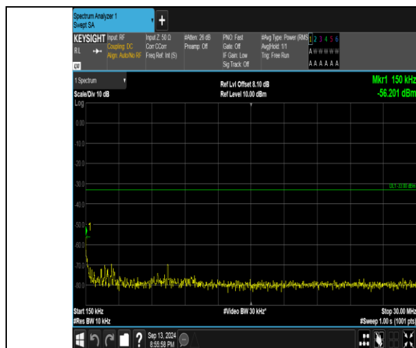
Band66_1.4MHz_16QAM_132322_1RB#0_0.15~30_0.15~30
