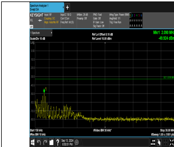
Band66_1.4MHz_16QAM_131979_1RB#0_0.15~30_0.15~30
