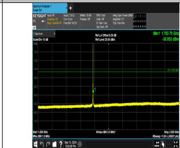
Band66_1.4MHz_QPSK_132665_6RB#0_1000~3000_1000~3000
