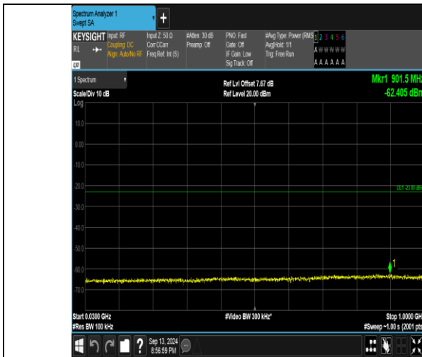
Band66_1.4MHz_QPSK_132322_1RB#5_30~1000_30~1000
