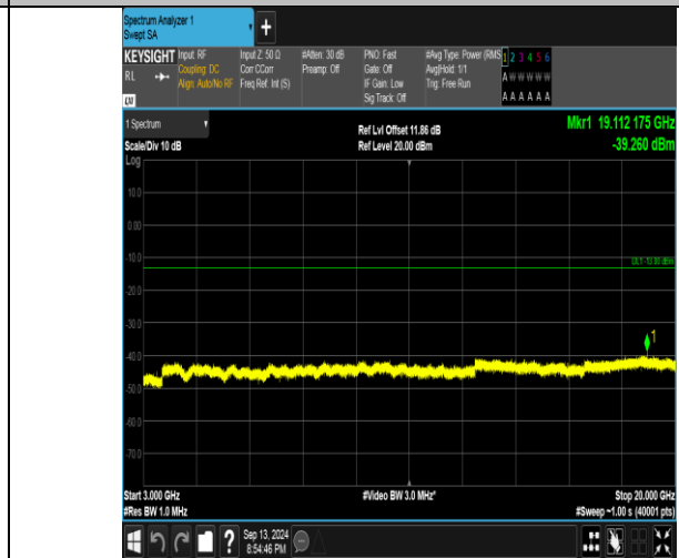
Band66_1.4MHz_16QAM_131979_6RB#0_3000~20000_3000~20000
