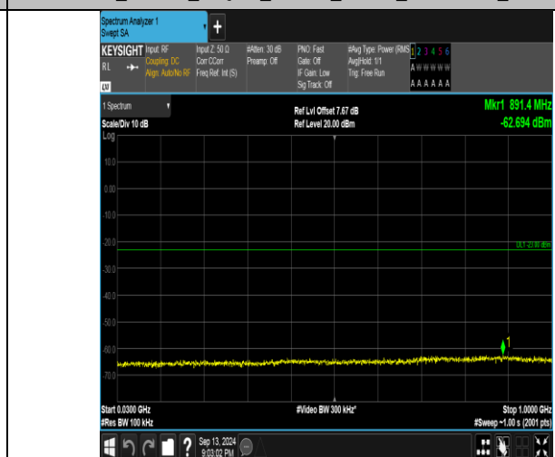
Band66_1.4MHz_16QAM_132665_1RB#5_30~1000_30~1000
