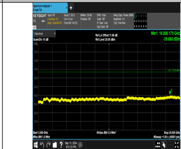
Band66_1.4MHz_16QAM_131979_1RB#0_3000~20000_3000~20000
