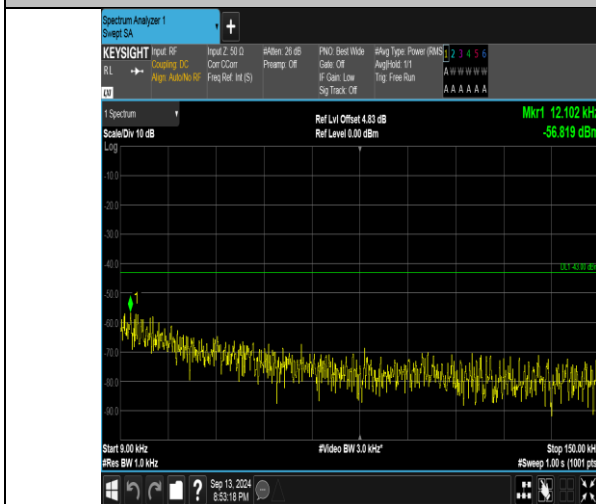
Band66_1.4MHz_QPSK_131979_6RB#0_0.009~0.15_0.009~0.15
