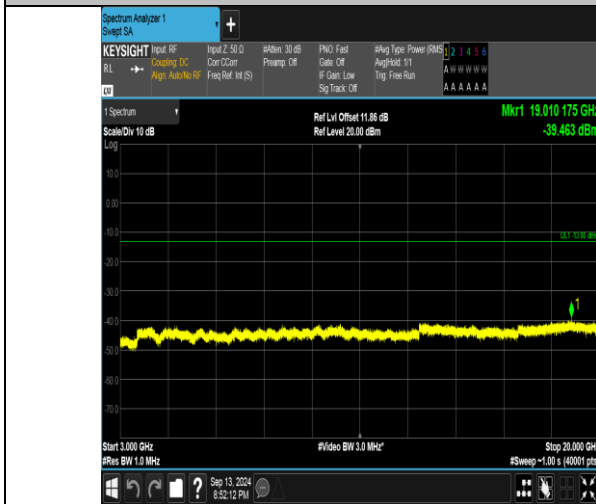
Band66_1.4MHz_QPSK_131979_1RB#5_3000~20000_3000~20000
