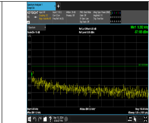
Band66_1.4MHz_16QAM_131979_6RB#0_0.009~0.15_0.009~0.15
