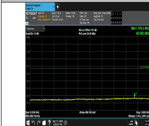
Band66_1.4MHz_QPSK_132322_6RB#0_30~1000_30~1000
