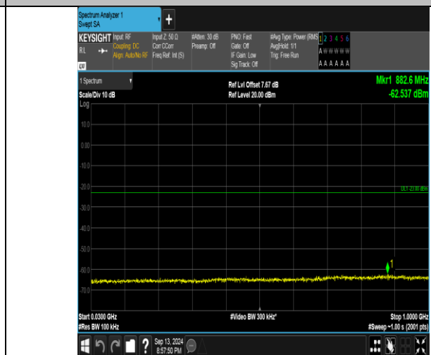
Band66_1.4MHz_16QAM_132322_1RB#5_30~1000_30~1000
