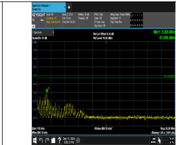
Band66_1.4MHz_QPSK_132665_1RB#0_0.15~30_0.15~30
