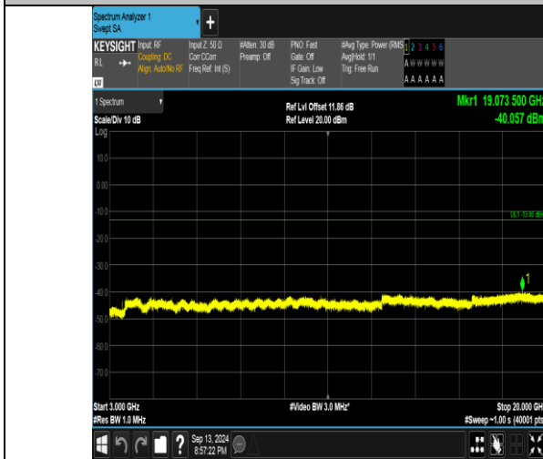
Band66_1.4MHz_QPSK_132322_1RB#5_3000~20000_3000~20000
