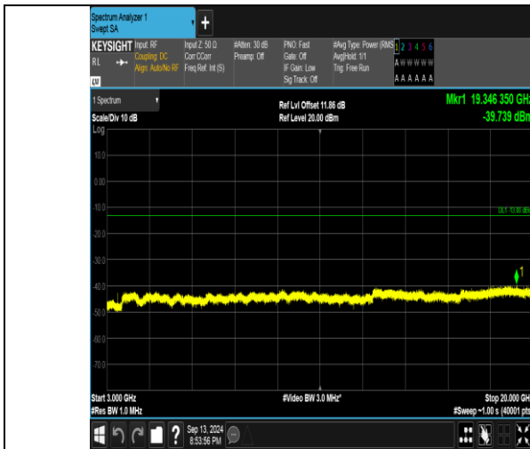
Band66_1.4MHz_QPSK_131979_6RB#0_3000~20000_3000~20000
