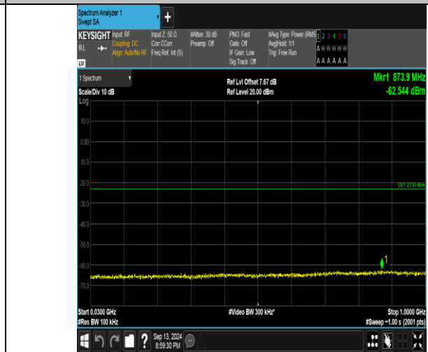
Band66_1.4MHz_16QAM_132322_6RB#0_30~1000_30~1000
