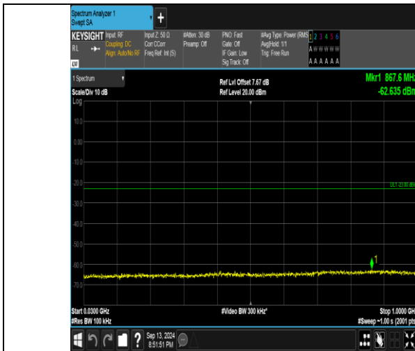
Band66_1.4MHz_QPSK_131979_1RB#5_30~1000_30~1000
