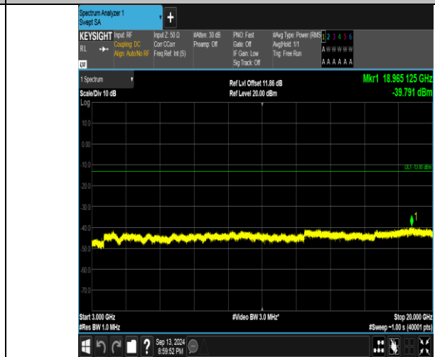
Band66_1.4MHz_16QAM_132322_6RB#0_3000~20000_3000~20000
