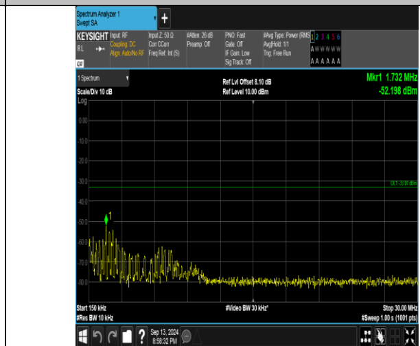
Band66_1.4MHz_QPSK_132322_6RB#0_0.15~30_0.15~30
