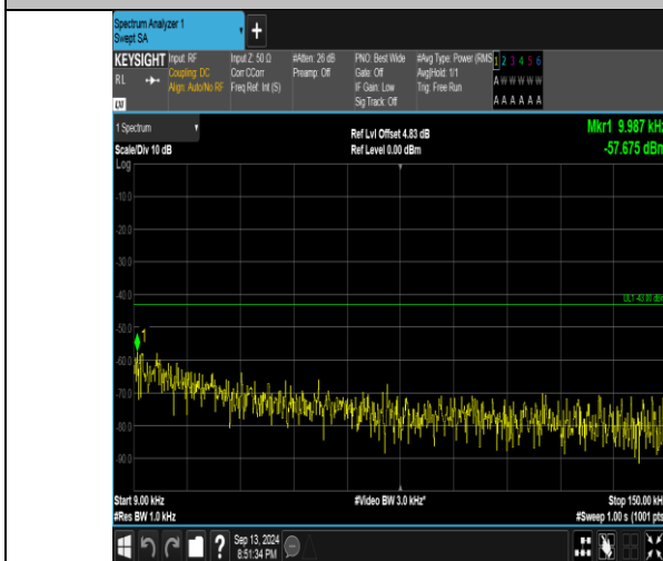
Band66_1.4MHz_QPSK_131979_1RB#5_0.009~0.15_0.009~0.15
