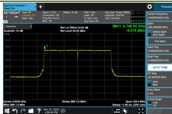
Channel 175 (6825MHz)
