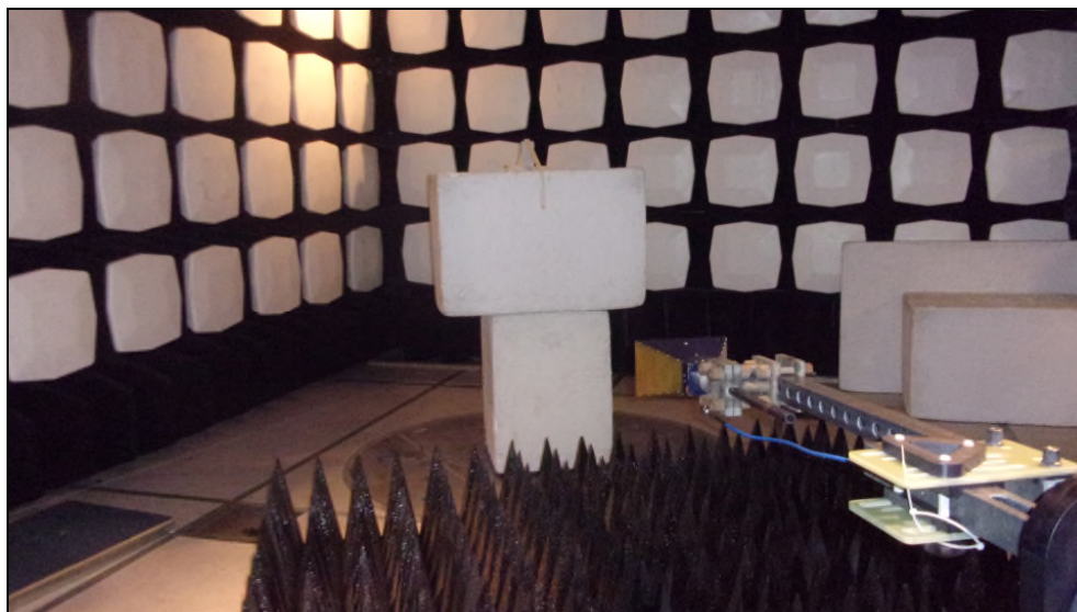
Figure 1: Radiated Emissions – 1GHz – 10GHz
