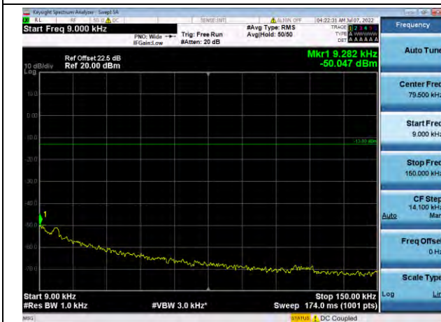
QPSK Middle channel - 9kHz~150KHz
