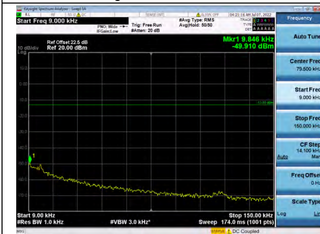
QPSK High channel - 9kHz~150KHz
