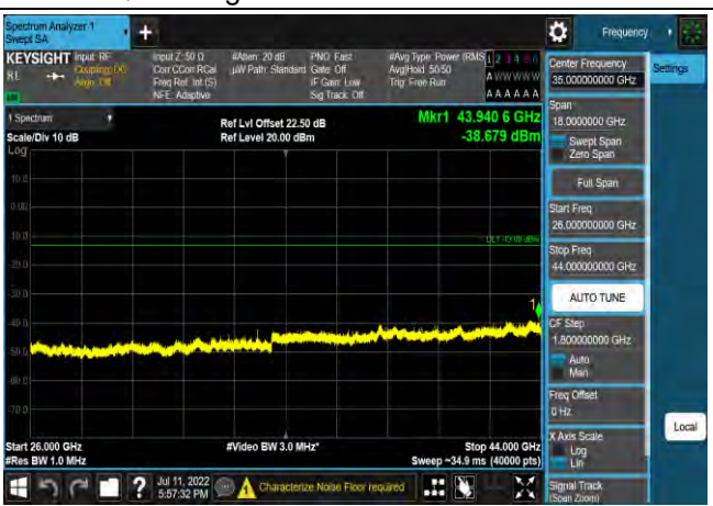
QPSK High channel - 26GHz~44GHz
