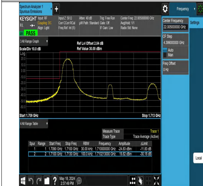
Band4_3MHz_QPSK_19965_1RB#0
