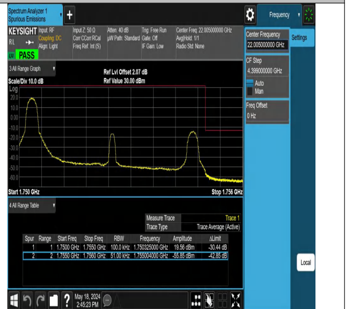
Band4_5MHz_QPSK_20375_1RB#0
