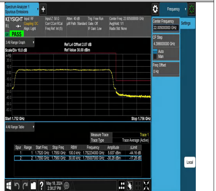
Band4_3MHz_QPSK_20385_15RB#0
