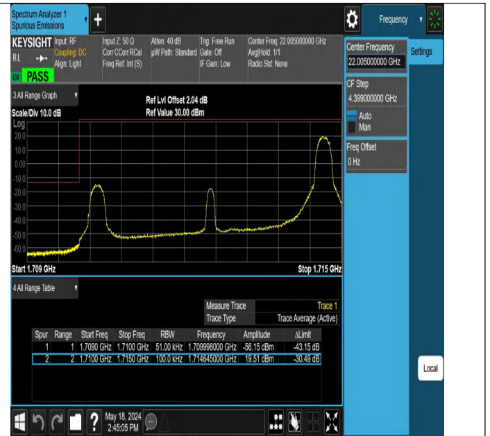
Band4_5MHz_QPSK_19975_1RB#24
