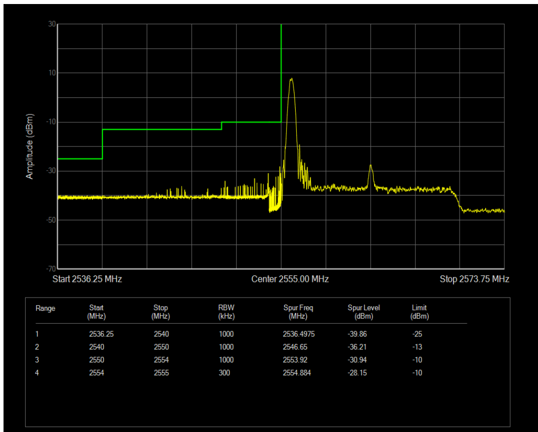
Band41(2555-2655) QAM16 BW=15MHz Channel=40315 RB Size=1 Position=#Max
