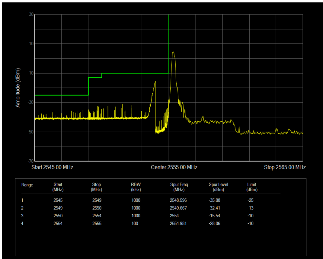
Band41(2555-2655) QAM16 BW=5MHz Channel=40265 RB Size=1 Position=#Max
