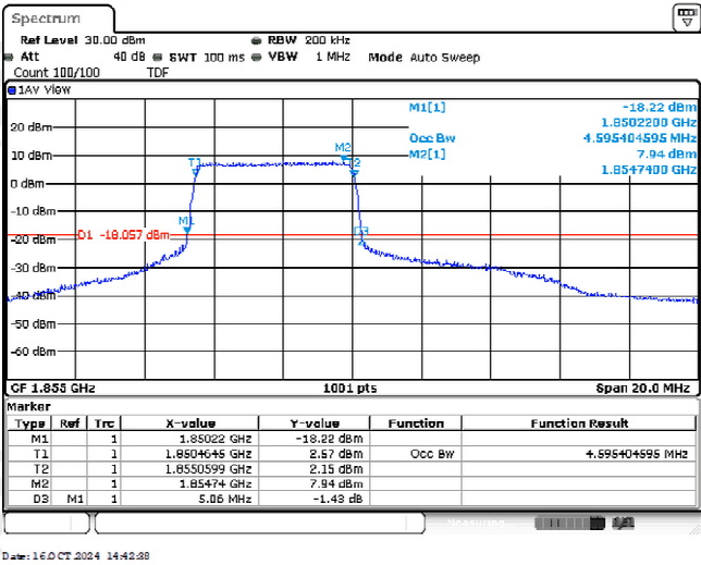
Band2-10MHz-16QAM-18650-25RB#0-4.595
