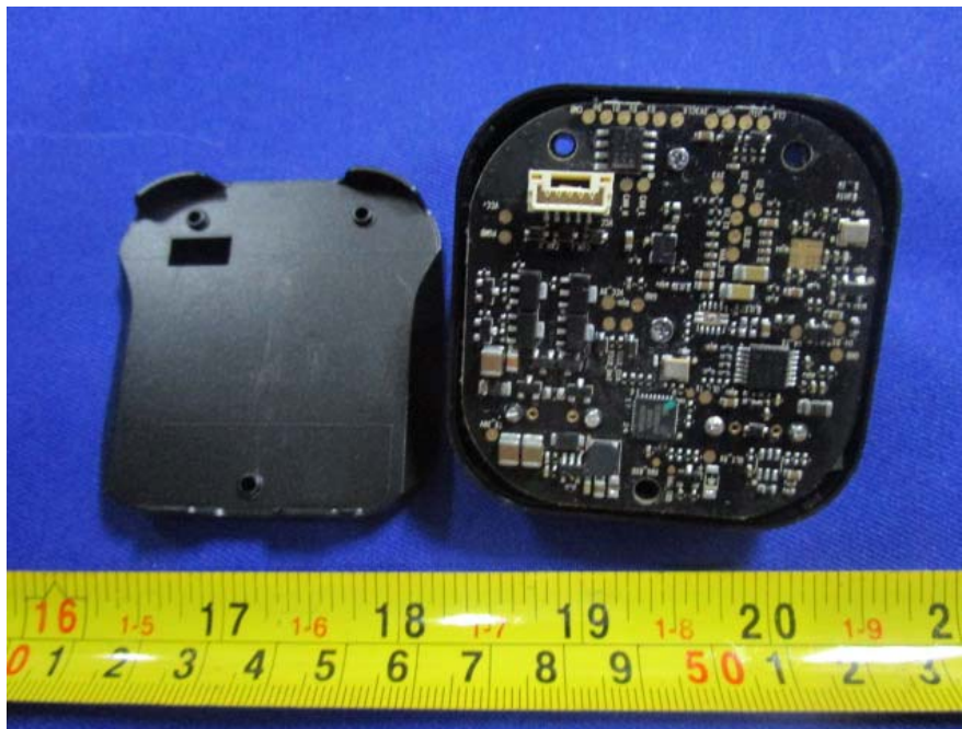
EUT –Sensor Unit Uncover View
