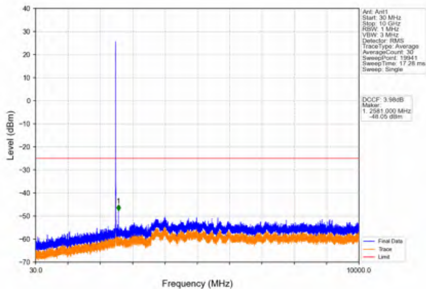
Band41 5MHz 64QAM LCH 2498.5MHz RB 1 0 NTNV
