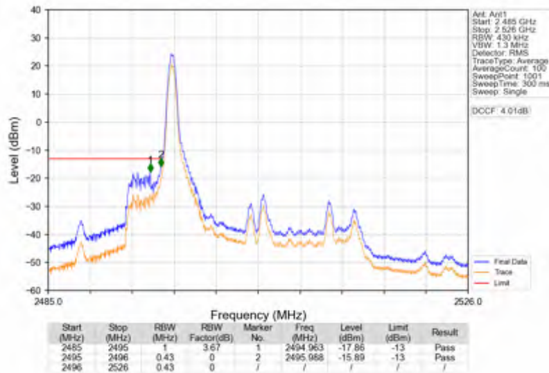
Band41 20MHz 64QAM LCH 2506MHz RB 100 0 NTN
