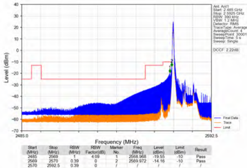
Band38 15MHz 64QAM LCH 2577.5MHz RB 1 0 NTNv
