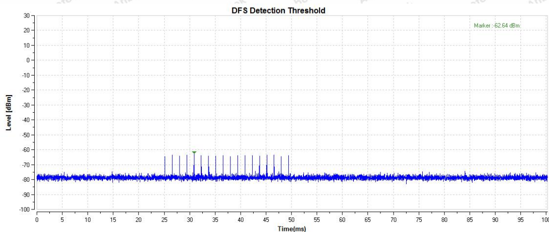
802.11n(HT20) SISO_5700_Type0
