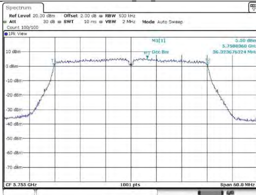
11N40MIMO Ant2 5755
