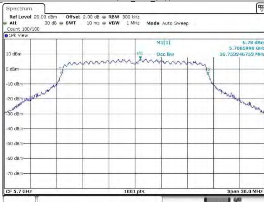
11A-CDD Ant2 5700
