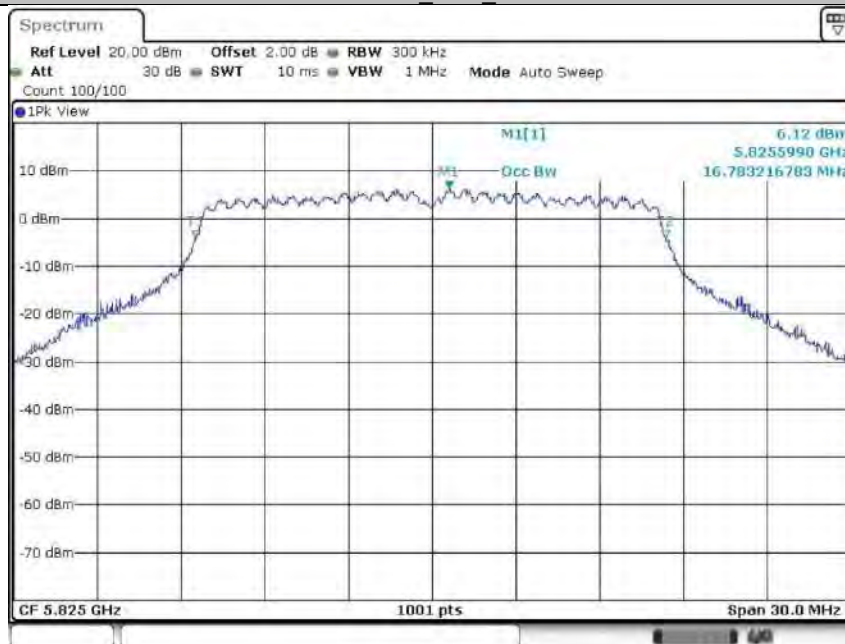
11A-CDD Ant2 5825
