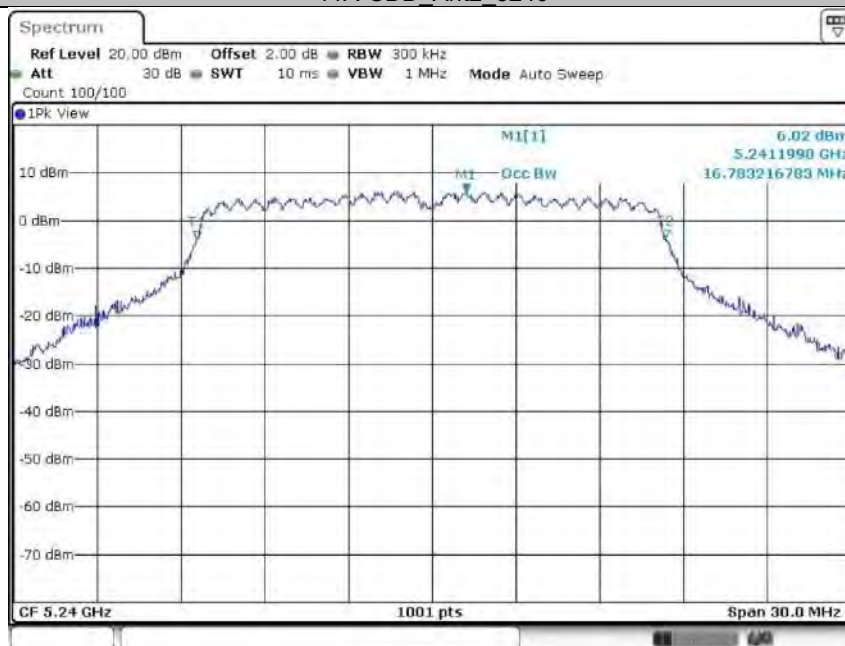
11A-CDD Ant2 5240
