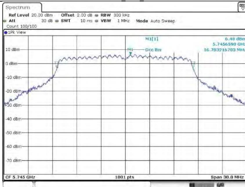
11A-CDD Ant2 5745
