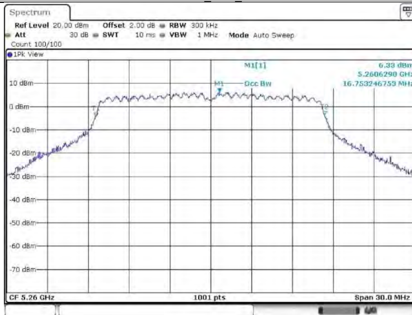
11A-CDD Ant2 5260
