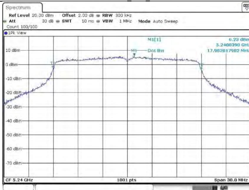
11N20SISO_Ant2_5240
