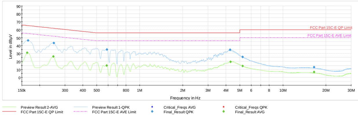
Plot 7-67. AC Line Conducted Emission with 802.15.4 Antenna WF7 (N, 250 kbps, ePA - Ch.11, with AC/DC adaptor via USB-C cable with wire charger)
