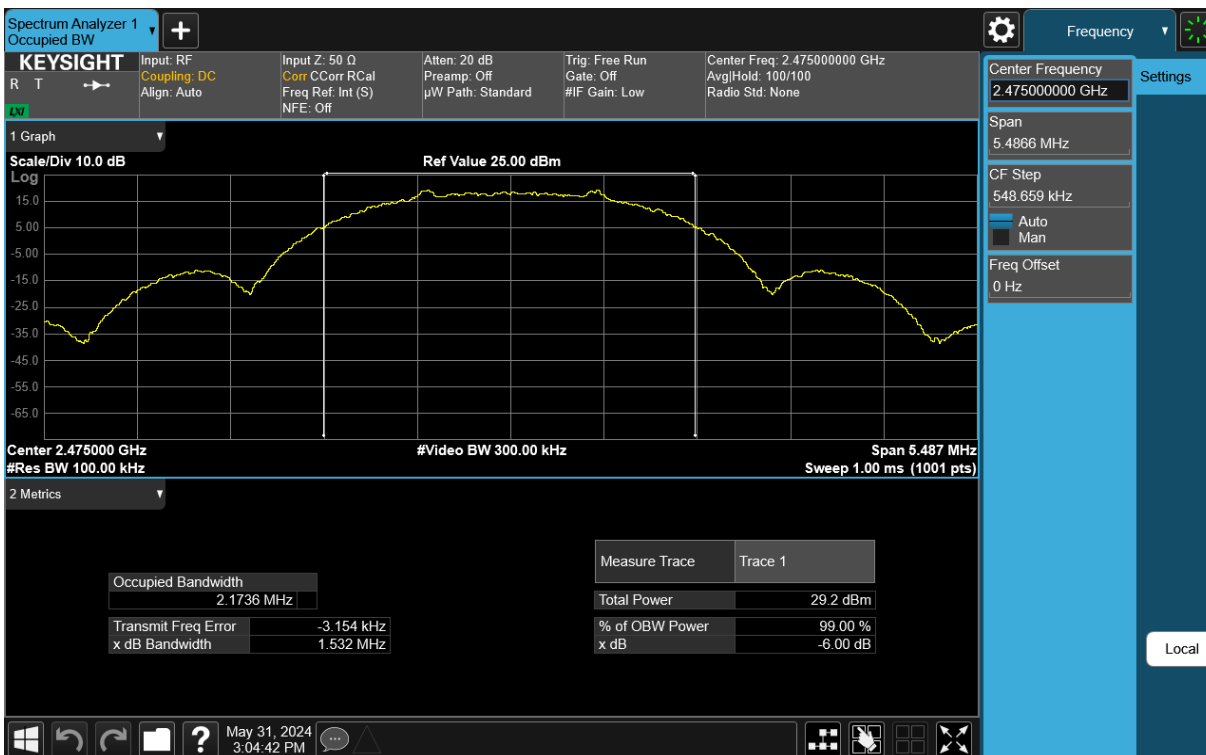
Plot 7-6. 6dB BW & 99% OBW Antenna WF7 (802.15.4, Ch. 25)
