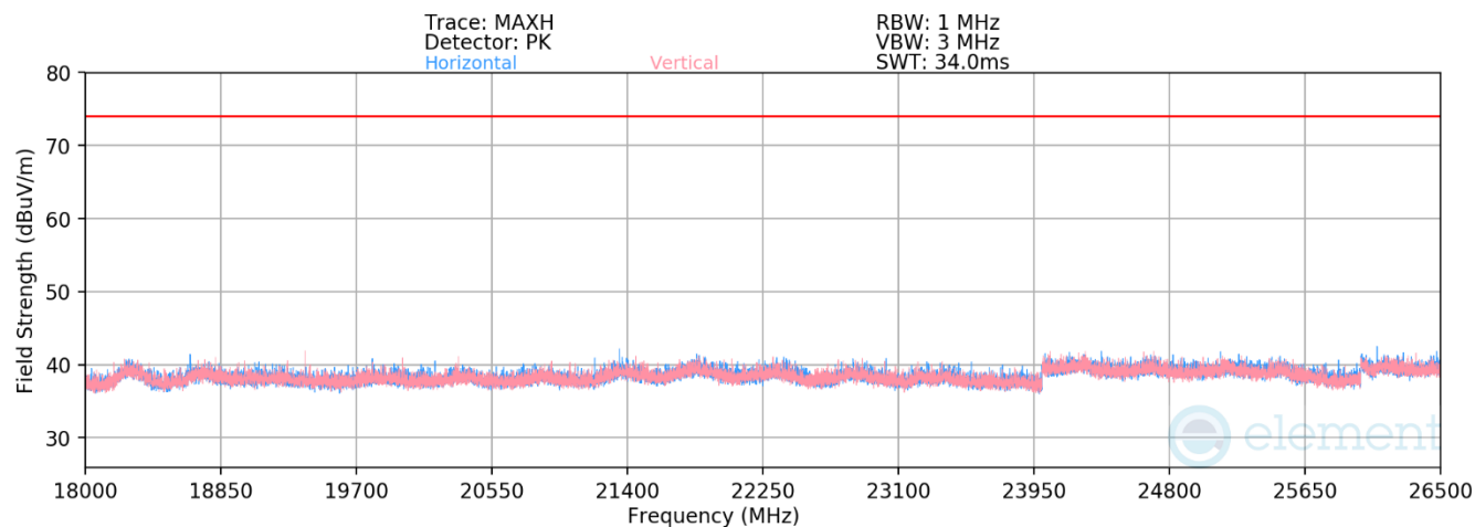
Plot 7-58. Radiated Spurious Emissions Antenna WF7 (802.15.4 ePA – Ch.25)
