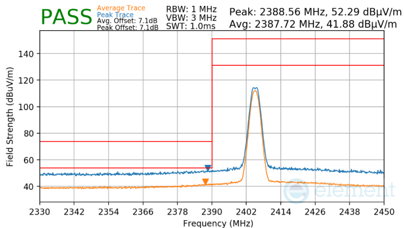
Plot 7-61. Radiated Restricted Lower Band Edge Measurement Antenna WF7
