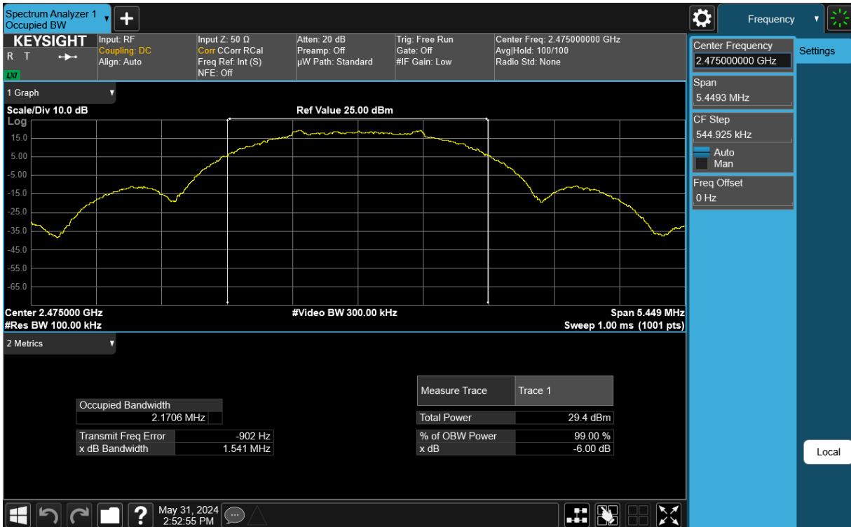
Plot 7-3. 6dB BW & 99% OBW Antenna WF8 (802.15.4, Ch. 25)
