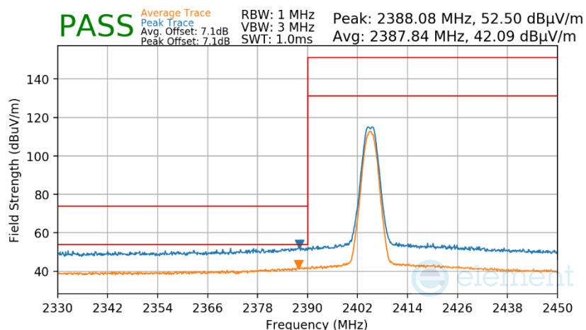
Plot 7-59. Radiated Restricted Lower Band Edge Measurement Antenna WF8
