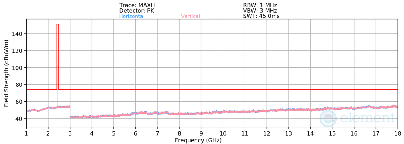
Plot 7-53. Radiated Spurious Emissions 1-18GHz Antenna WF7 (802.15.4 ePA – Ch. 18)
