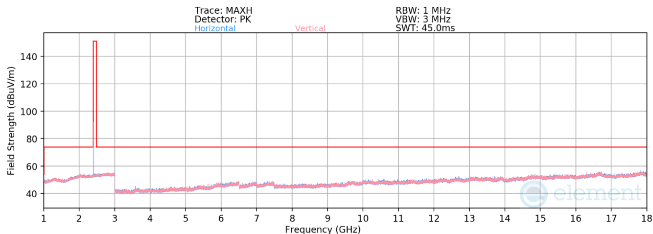
Plot 7-55. Radiated Spurious Emissions 1-18GHz Antenna WF2 (802.15.4 iPA – Ch. 11)
