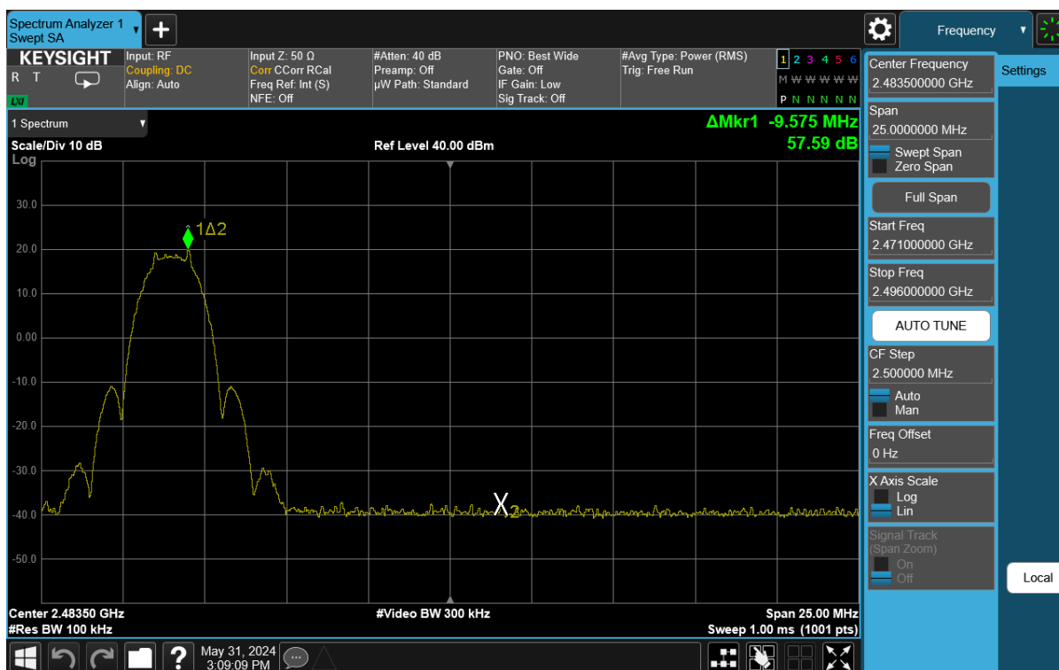
Plot 7-28. Band Edge Antenna WF7 (802.15.4, ePA – Ch. 25)
