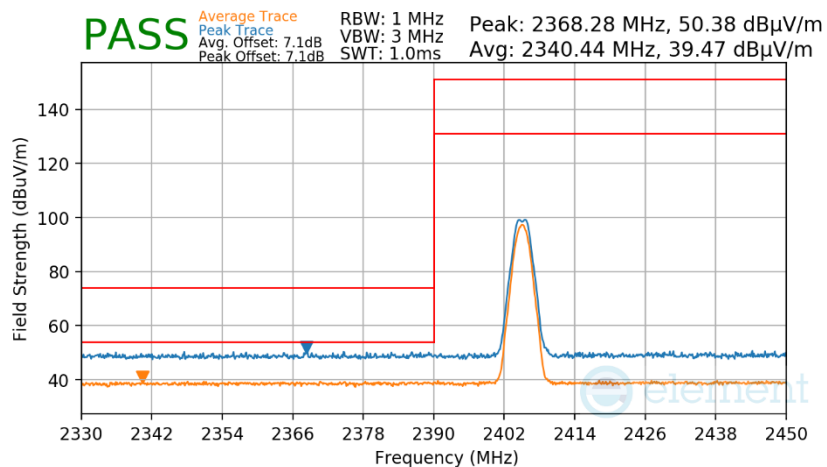
Plot 7-63. Radiated Restricted Lower Band Edge Measurement Antenna WF2
