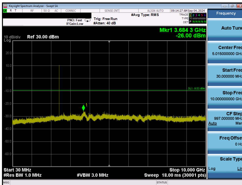
Plot 7-45. Conducted Spurious Antenna WF2 (802.15.4, iPA – Ch. 18)
