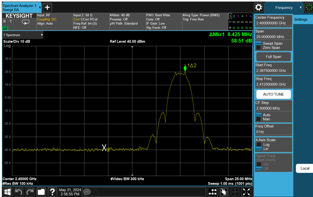
Plot 7-25. Band Edge Antenna WF8 (802.15.4, ePA – Ch. 11)
