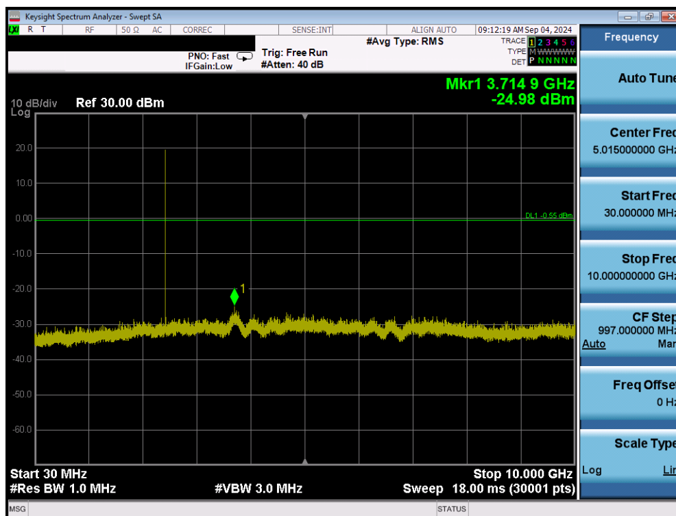
Plot 7-39. Conducted Spurious Antenna WF7 (802.15.4, ePA – Ch. 18)
