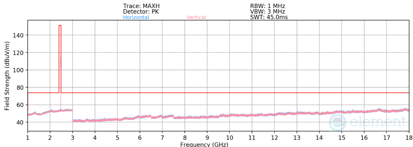
Plot 7-51. Radiated Spurious Emissions 1-18GHz Antenna WF8 (802.15.4 ePA – Ch. 25)
