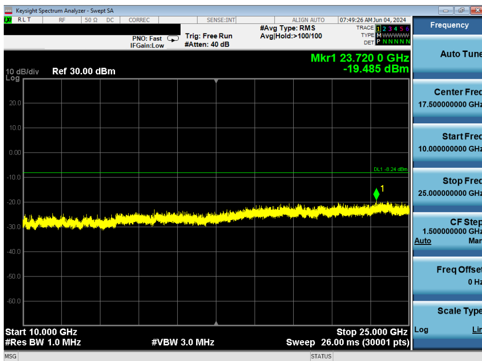
Plot 7-48. Conducted Spurious Antenna WF2 (802.15.4, iPA – Ch. 25)
