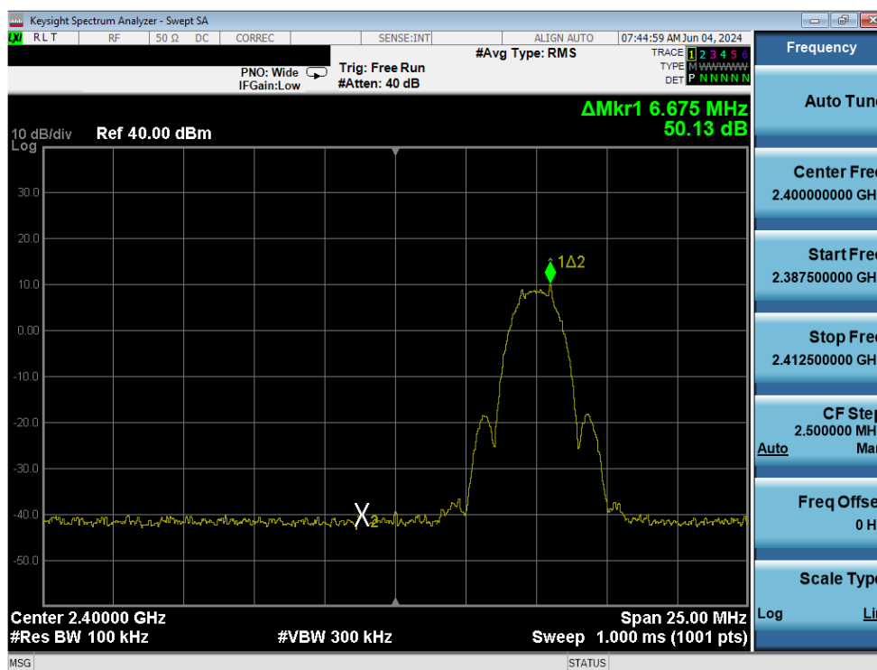
Plot 7-29. Band Edge Antenna WF2 (802.15.4, iPA – Ch. 11)
