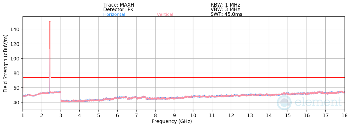
Plot 7-52. Radiated Spurious Emissions 1-18GHz Antenna WF7 (802.15.4 ePA – Ch. 11)
