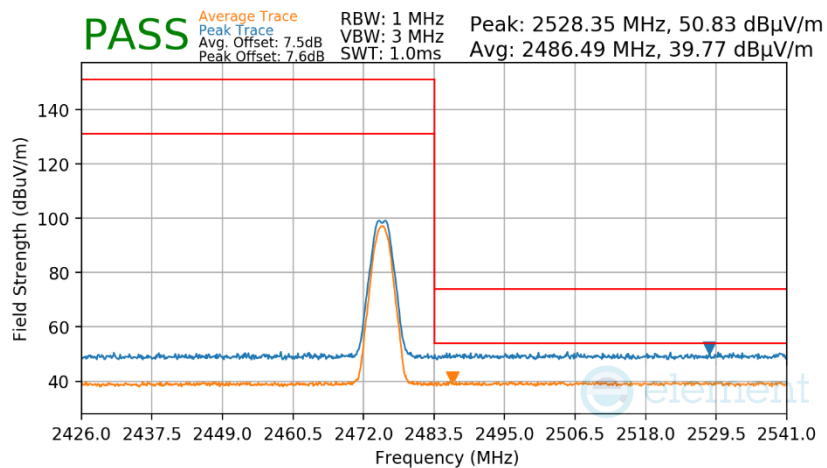
Plot 7-64. Radiated Restricted Upper Band Edge Measurement Antenna WF2
