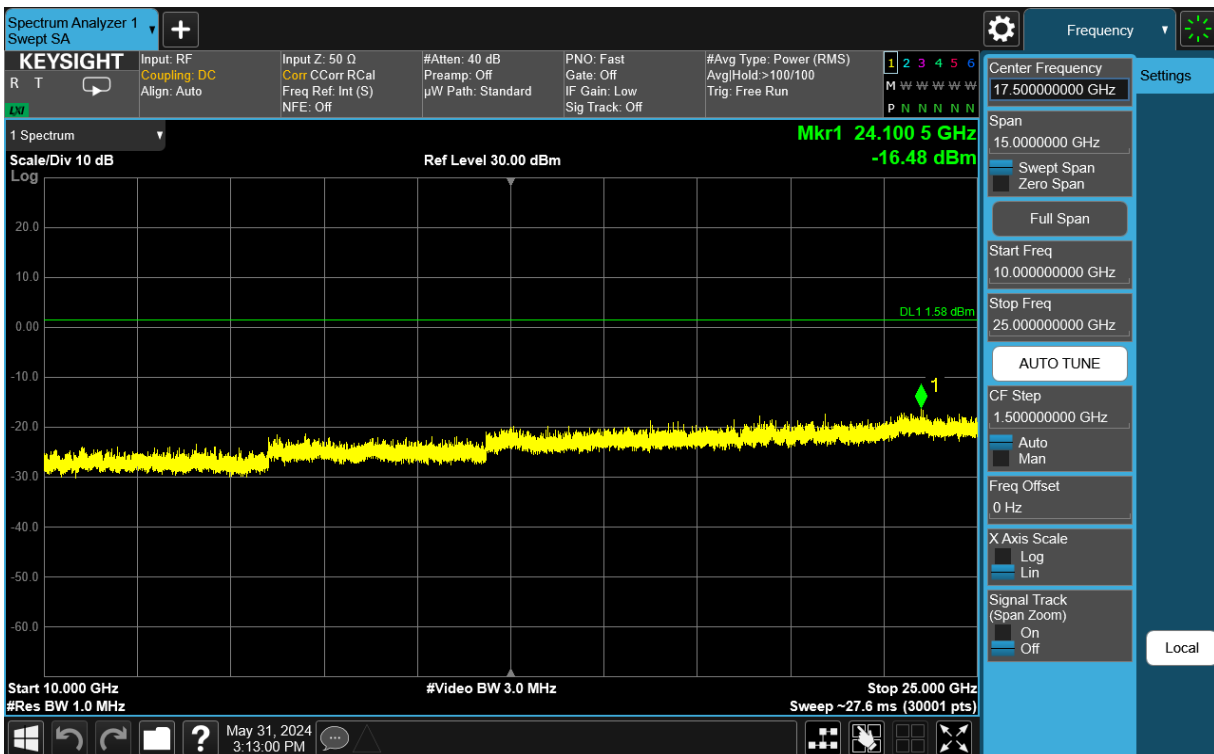
Plot 7-42. Conducted Spurious Antenna WF7 (802.15.4, ePA – Ch. 25)
