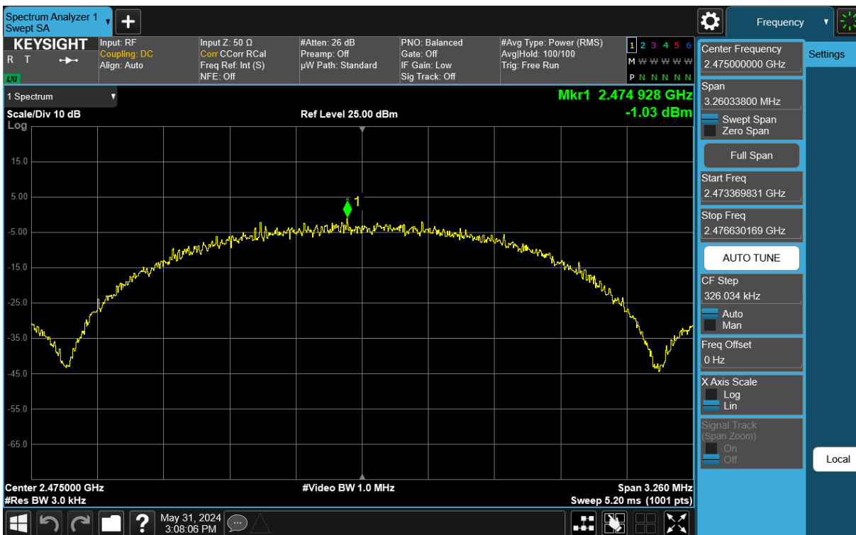
Plot 7-21. Power Spectral Density Antenna WF7 (802.15.4, iPA – Ch. 25)
