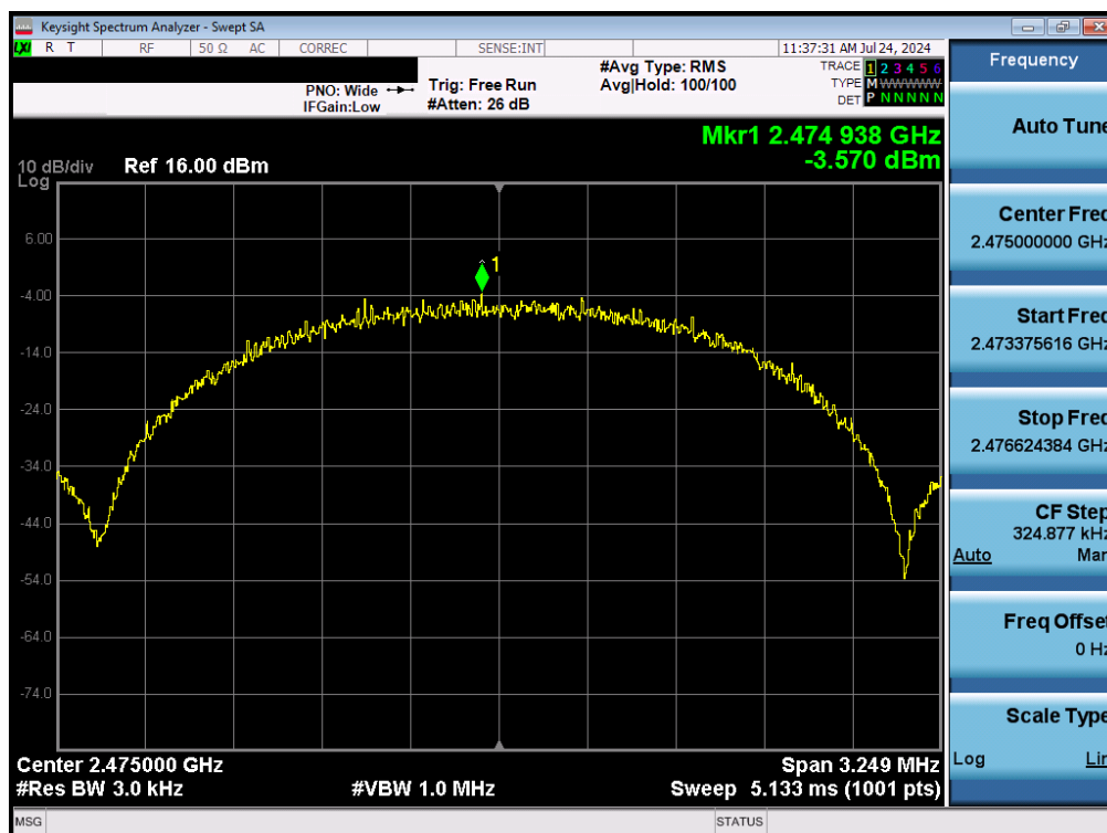
Plot 7-24. Power Spectral Density Antenna WF2 (802.15.4, iPA – Ch. 25)
