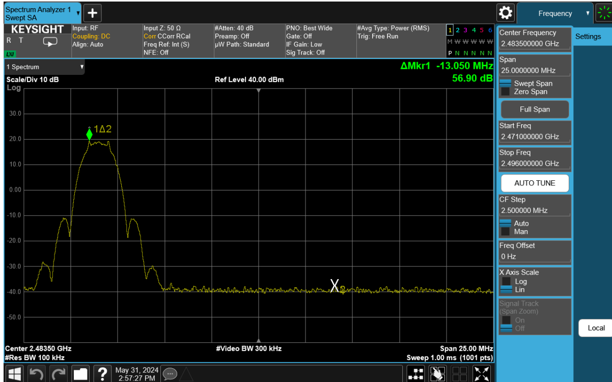
Plot 7-26. Band Edge Antenna WF8 (802.15.4, ePA – Ch. 25)
