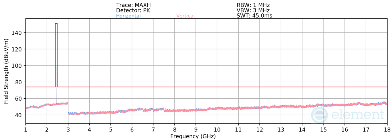
Plot 7-56. Radiated Spurious Emissions 1-18GHz Antenna WF2 (802.15.4 iPA – Ch. 18)
