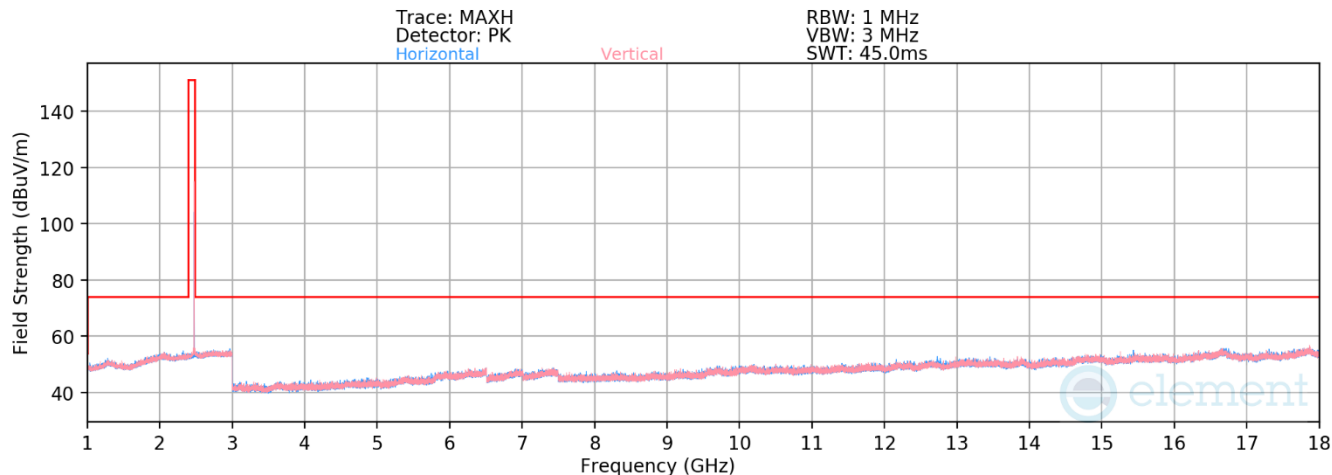
Plot 7-54. Radiated Spurious Emissions 1-18GHz Antenna WF7 (802.15.4 ePA – Ch. 25)
