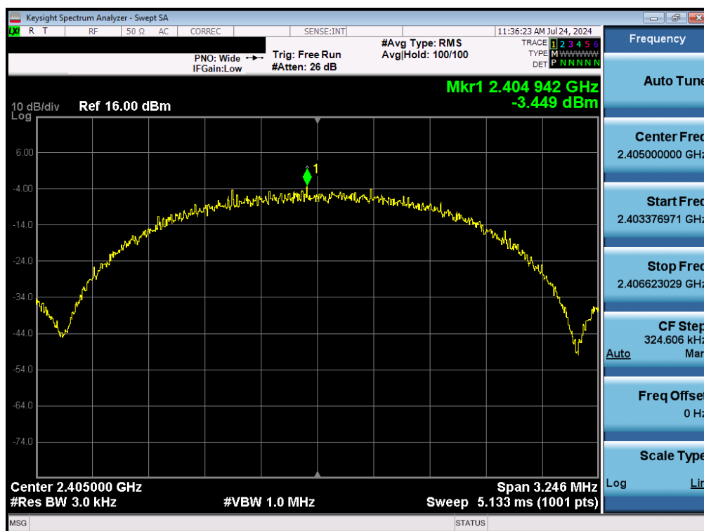
Plot 7-22. Power Spectral Density Antenna WF2 (802.15.4, iPA – Ch. 11)
