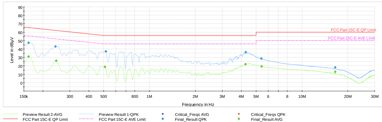
Plot 7-66. AC Line Conducted Emission with 802.15.4 Antenna WF7 (L1, 250 kbps, ePA - Ch.11, with AC/DC adaptor via USB-C cable with wire charger)
