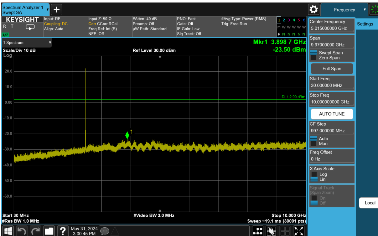
Plot 7-35. Conducted Spurious Antenna WF8 (802.15.4, ePA – Ch. 25)
