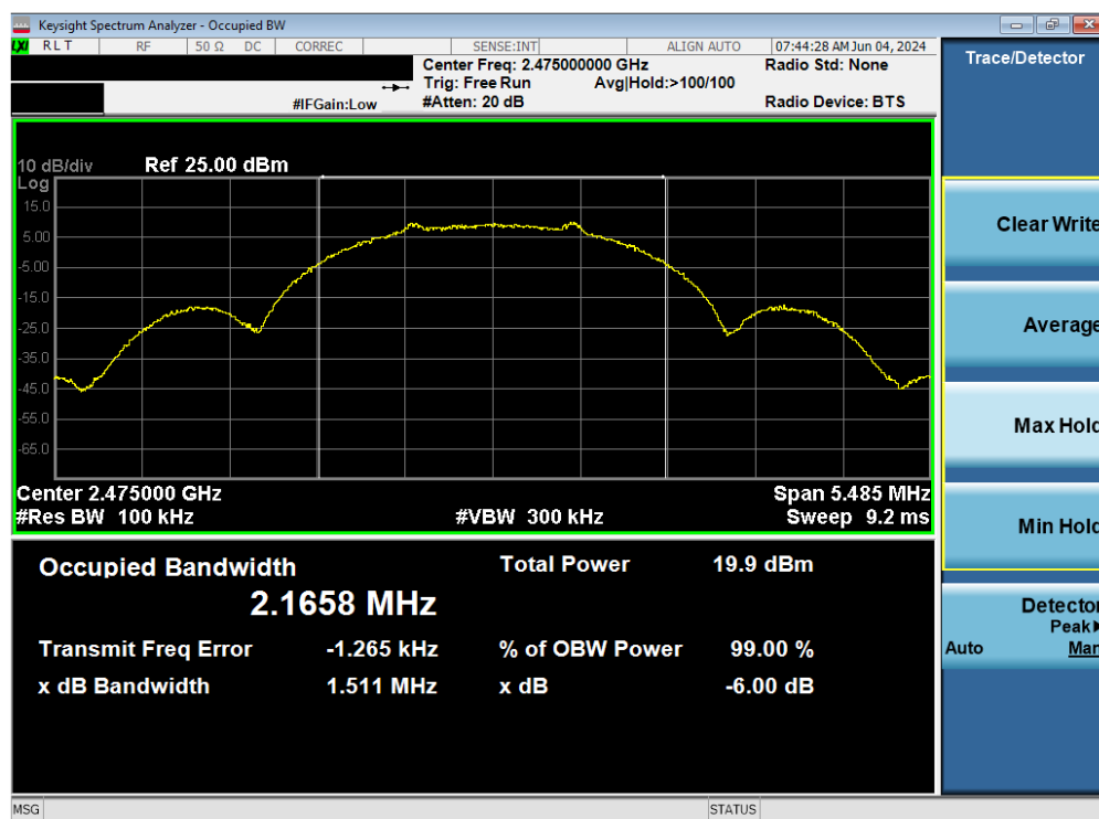
Plot 7-9. 6dB BW & 99% OBW Antenna WF2 (802.15.4, Ch. 25)
