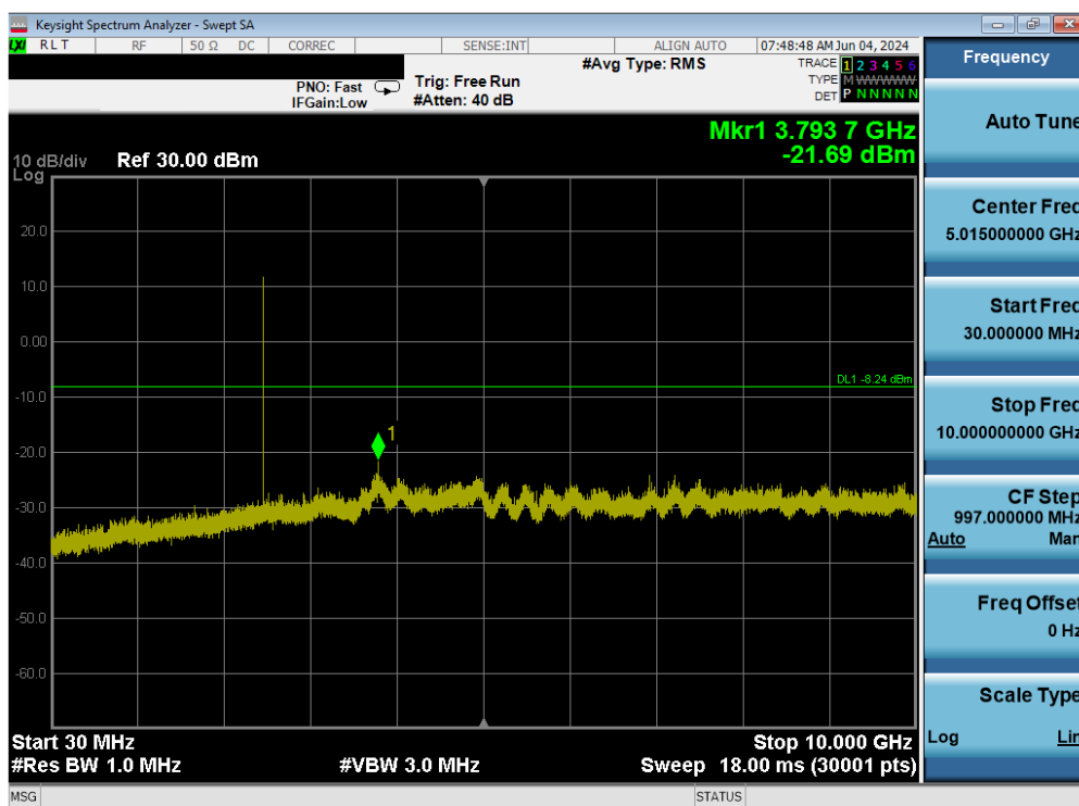
Plot 7-47. Conducted Spurious Antenna WF2 (802.15.4, iPA – Ch. 25)
