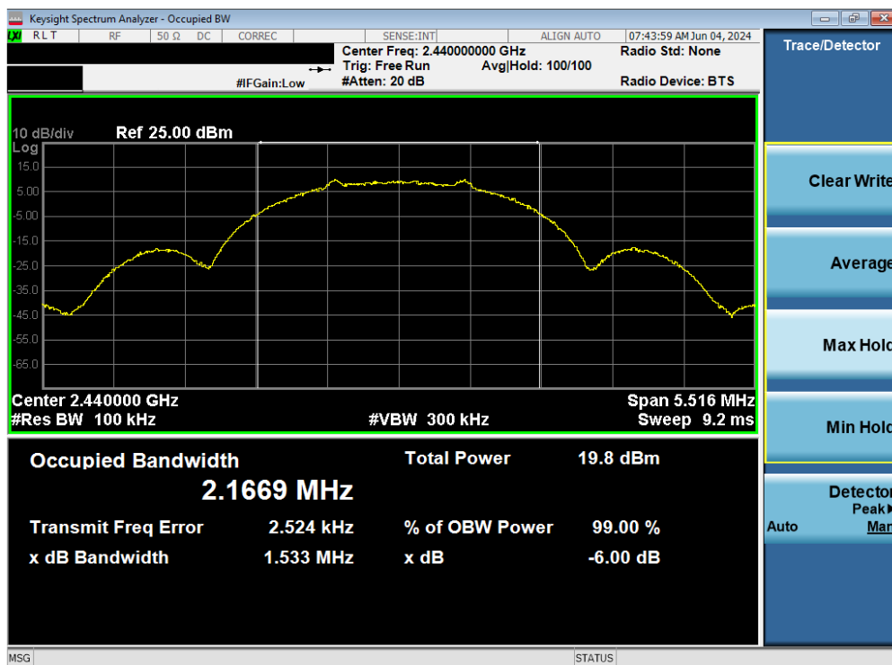
Plot 7-8. 6dB BW & 99% OBW Antenna WF2 (802.15.4, Ch. 18)
