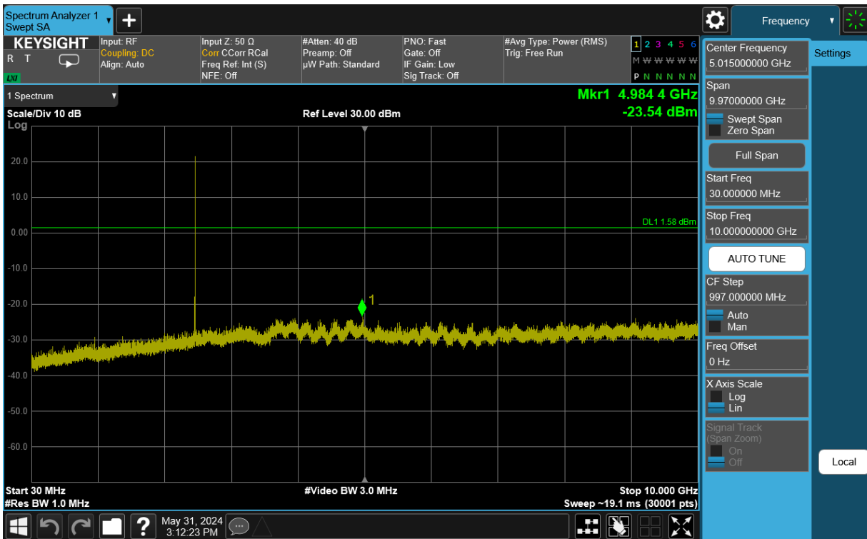
Plot 7-41. Conducted Spurious Antenna WF7 (802.15.4, ePA – Ch. 25)
