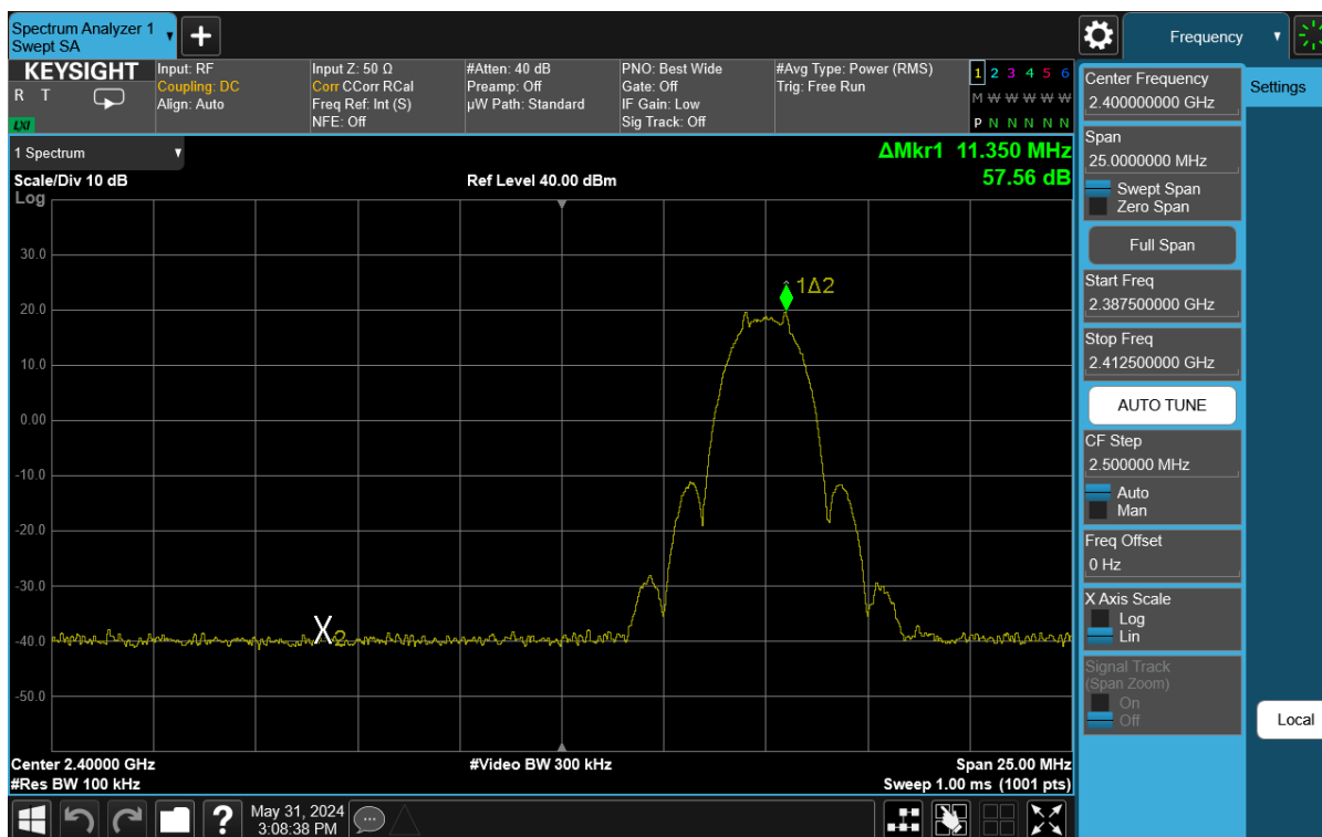
Plot 7-27. Band Edge Antenna WF7 (802.15.4, ePA – Ch. 11)
