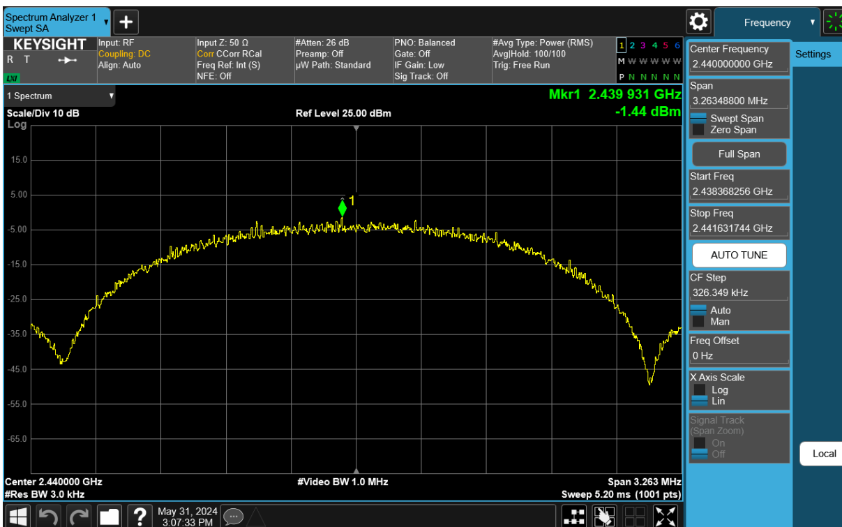
Plot 7-20. Power Spectral Density Antenna WF7 (802.15.4, iPA – Ch. 18)
