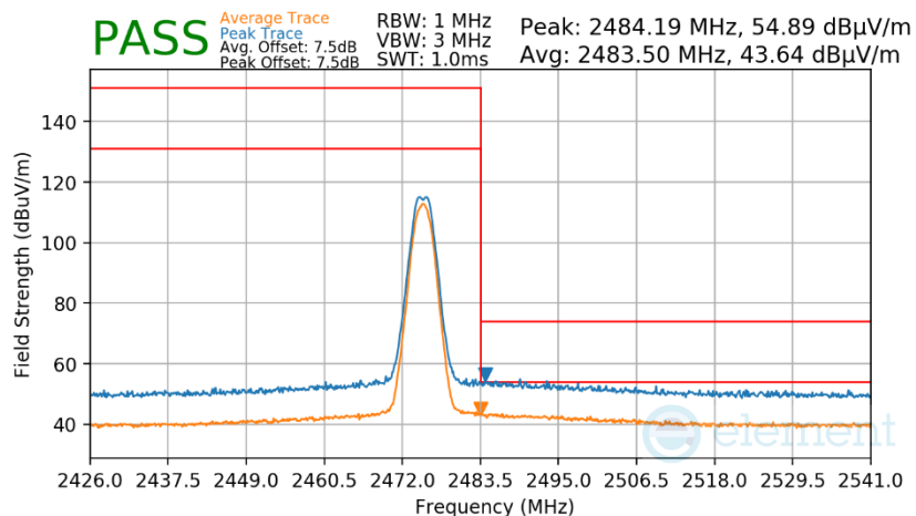
Plot 7-60. Radiated Restricted Upper Band Edge Measurement Antenna WF8
