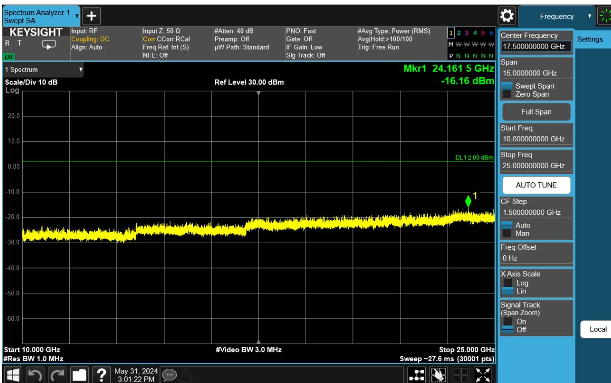
Plot 7-36. Conducted Spurious Antenna WF8 (802.15.4, ePA – Ch. 25)
