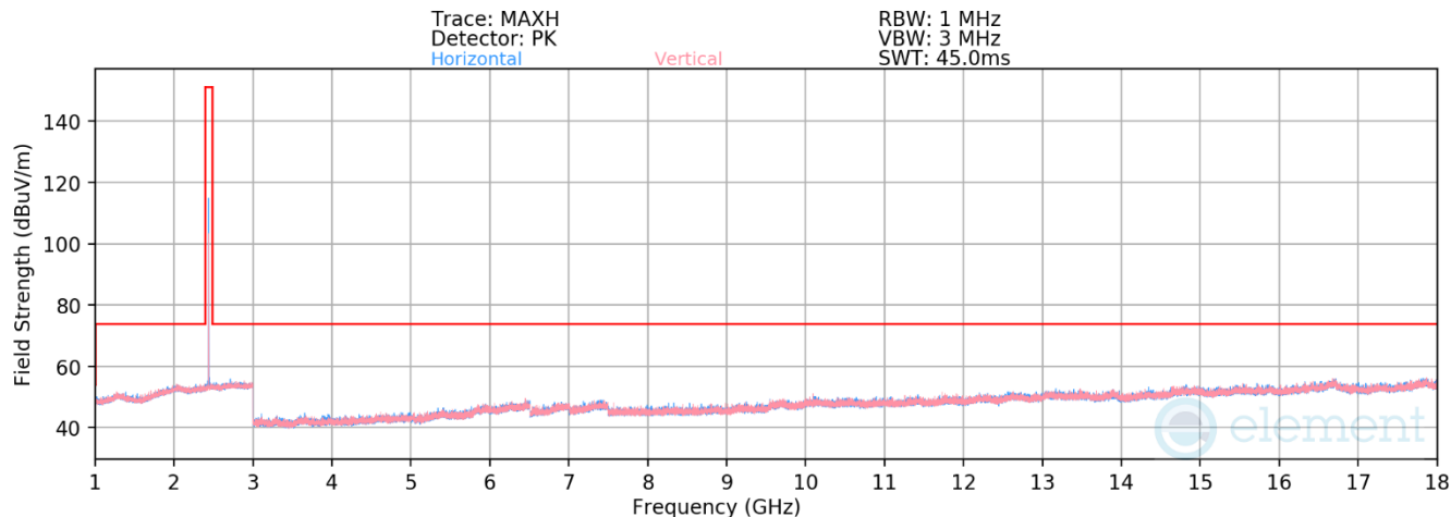
Plot 7-50. Radiated Spurious Emissions 1-18GHz Antenna WF8 (802.15.4 ePA – Ch. 18)
