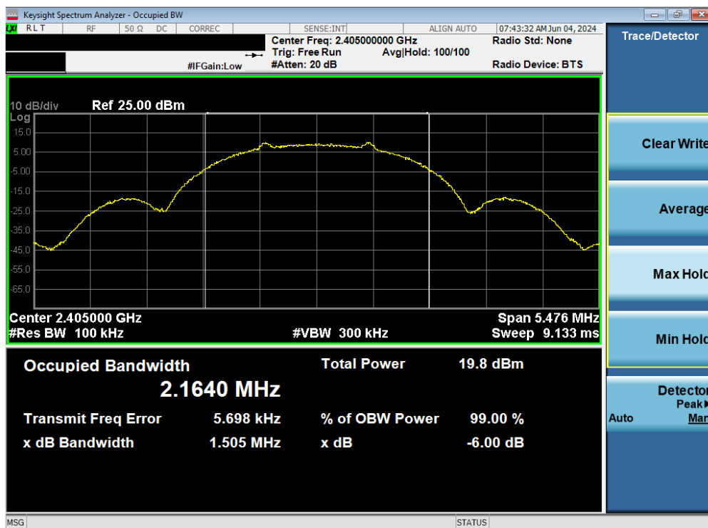
Plot 7-7. 6dB BW & 99% OBW Antenna WF2 (802.15.4, Ch. 11)
