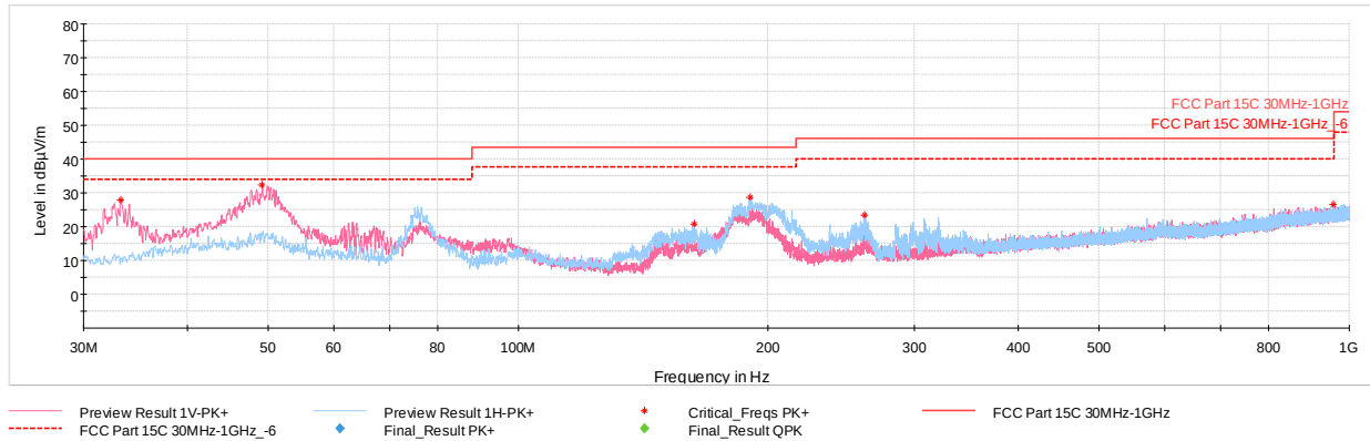
Plot 7-65. Radiated Spurious Emissions 30MHz-1GHz Antenna WF7 (250kbps, ePA - Ch.11, with AC/DC adaptor via USB-C cable with wire charger)
