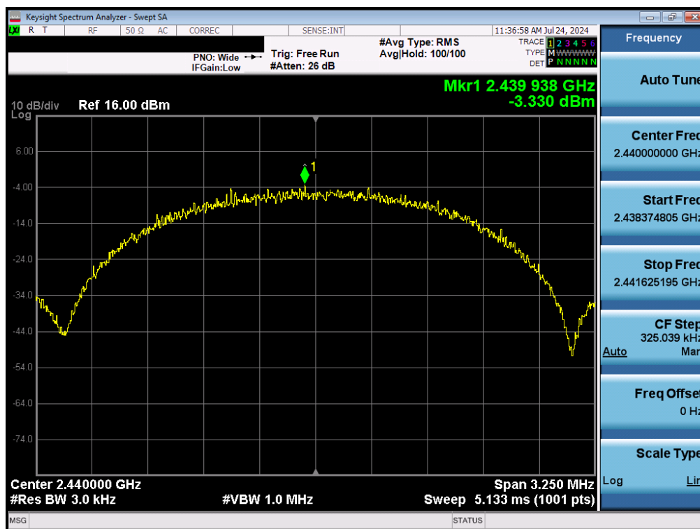
Plot 7-23. Power Spectral Density Antenna WF2 (802.15.4, iPA – Ch. 18)
