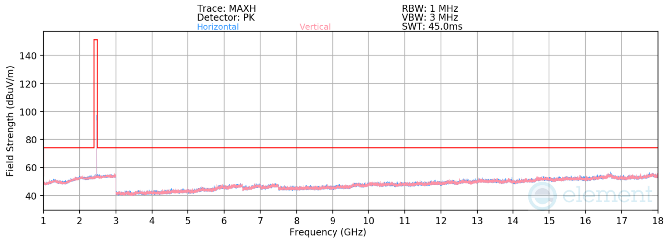
Plot 7-57. Radiated Spurious Emissions 1-18GHz Antenna WF2 (802.15.4 iPA – Ch. 25)
