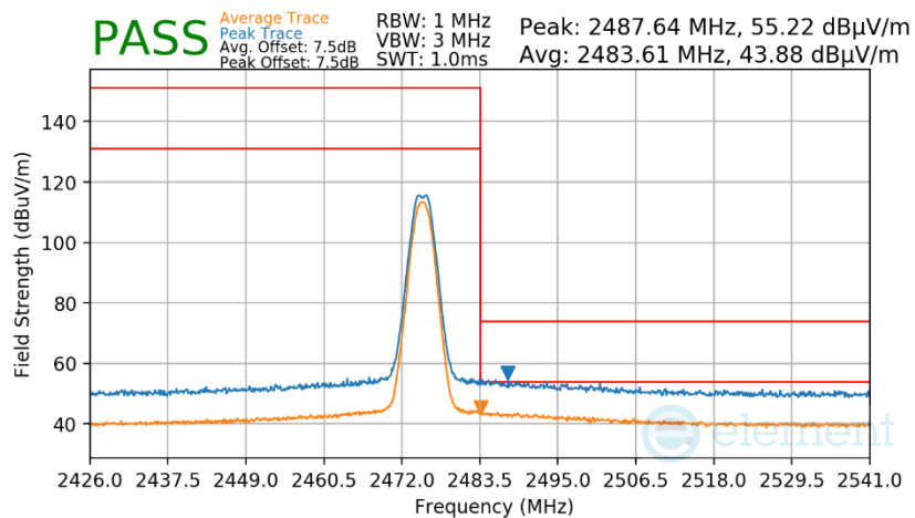
Plot 7-62. Radiated Restricted Upper Band Edge Measurement Antenna WF7
