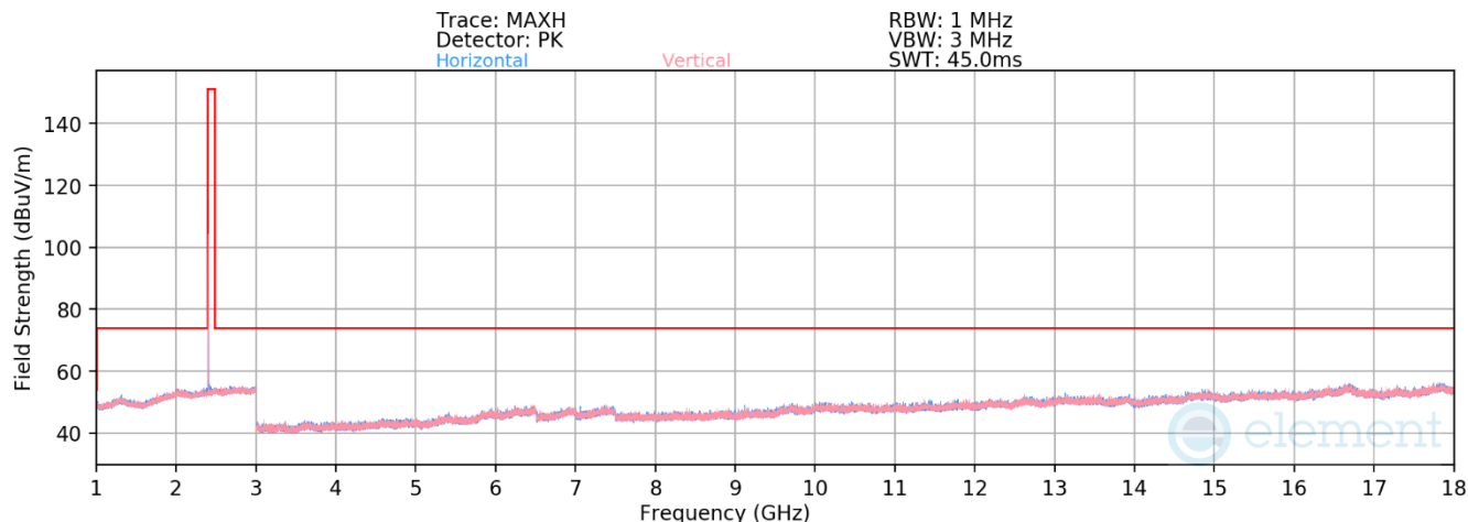
Plot 7-49. Radiated Spurious Emissions 1-18GHz Antenna WF8 (802.15.4 ePA – Ch. 11)
