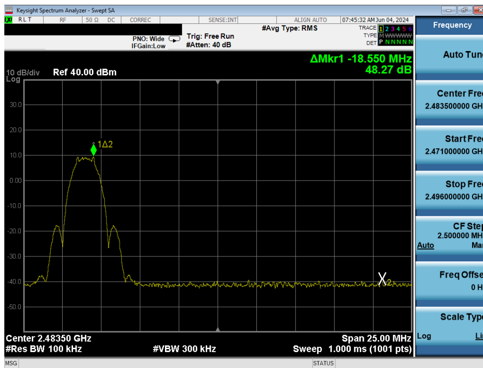
Plot 7-30. Band Edge Antenna WF2 (802.15.4, iPA – Ch. 25)
