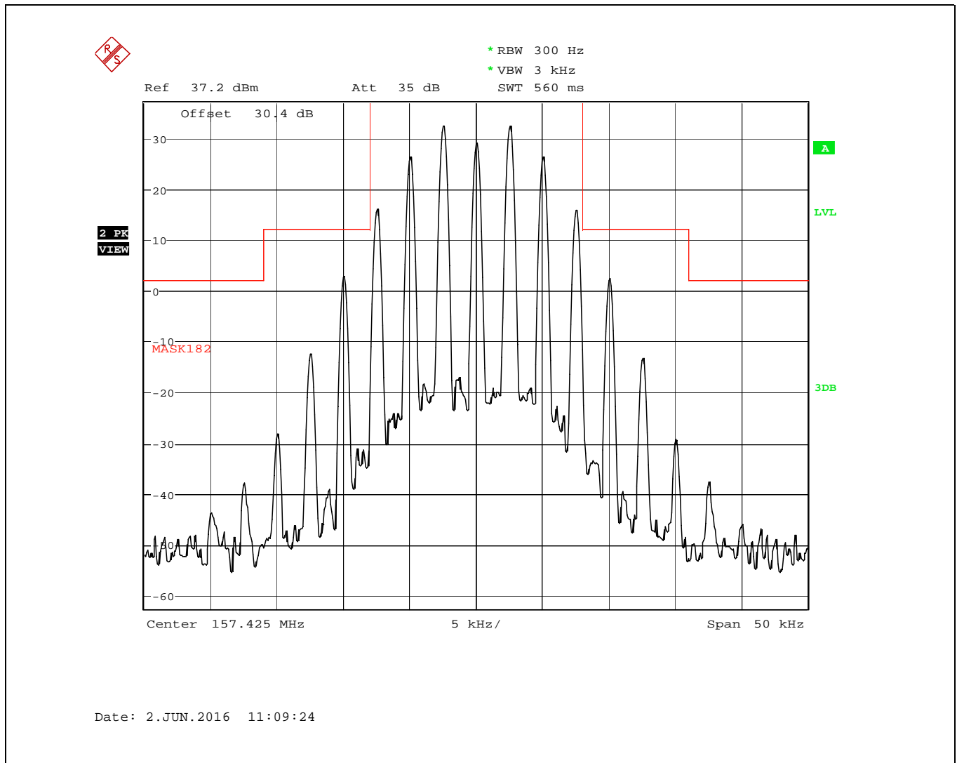
Plot 5.4.4.2.6. Emission Limitation for 157.425 MHz, 25 kHz Channel Spacing High Power (5 W), G3E, 50 kHz Span
