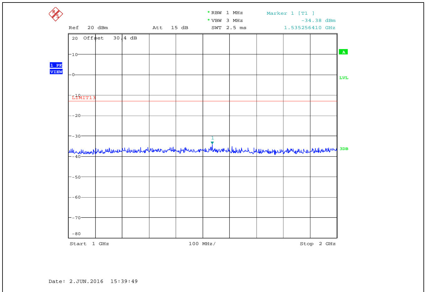
Plot 5.5.4.3. Spurious Emissions at Antenna Terminals, 156.050 MHz, 25 kHz Channel Spacing, 5 W, 1 GHz - 2 GHz
