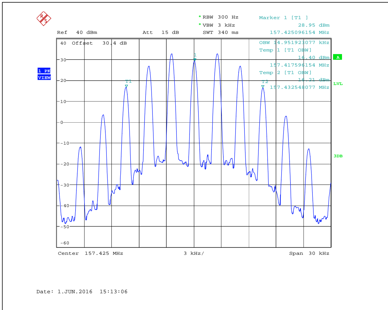
Plot 5.4.4.1.2. Occupied Bandwidth for 157.425 MHz, 25 kHz Channel Spacing, High Power (5 W), G3E
