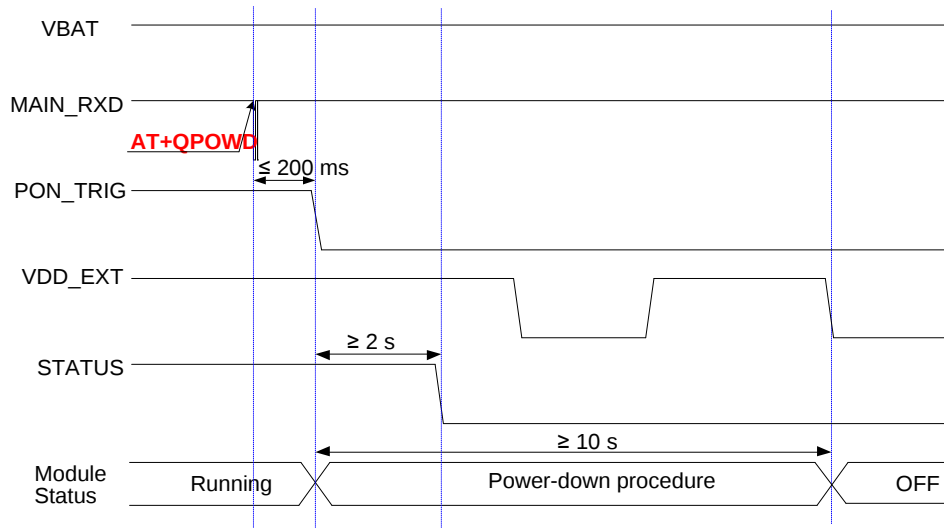
Figure 13: Power-down Timing (AT Command & PON_TRIG)
