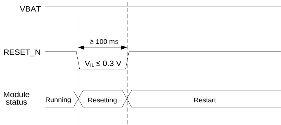
Figure 16: Reset Timing
