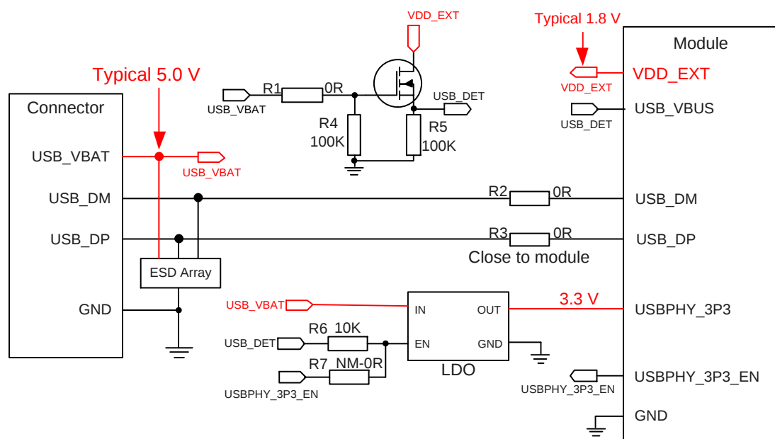
Figure 20: Reference Design of USB Interface
