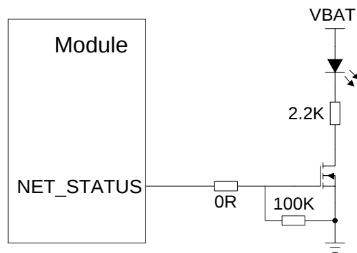
Figure 23: Reference Design of NET_STATUS
