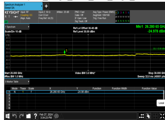
N78(70M)_CP-OFDM_16 QAM_Edge_1RB_Left_High_CH
