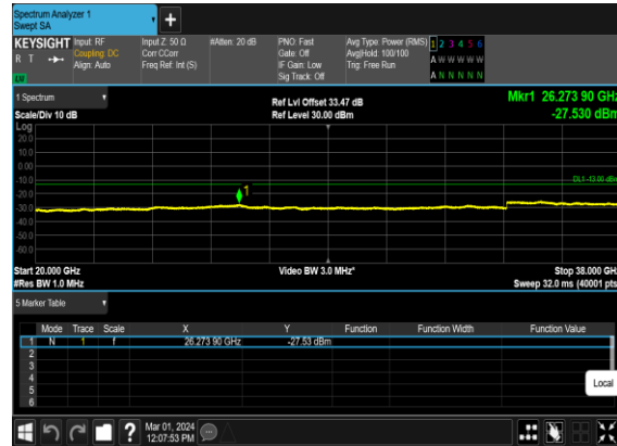
B26_N78(70M)_DFT-s- OFDM_BPSK_Edge_1RB_Left_High_CH
