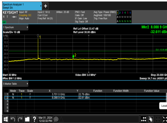
B26_N78(70M)_DFT-s-OFDM_QPSK_Edge_1RB_Left_Low_CH
