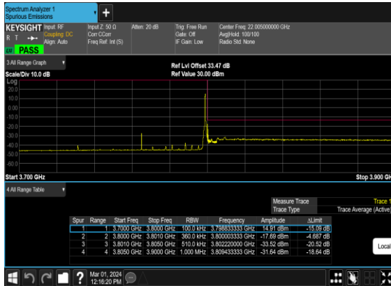
B26_N78(70M)_DFT-s- OFDM_BPSK_Edge_1RB_Right_High_CH
