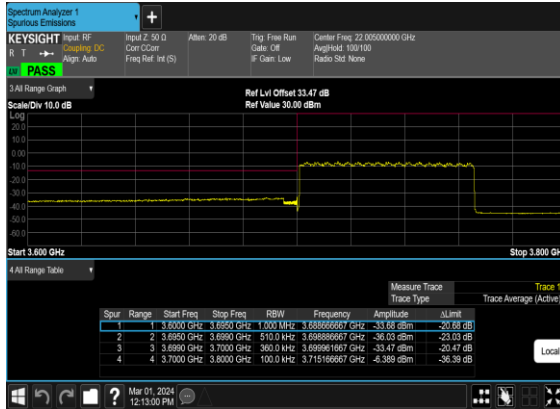
B26_N78(70M)_DFT-s- OFDM_BPSK_Outer_Full_Low_CH
