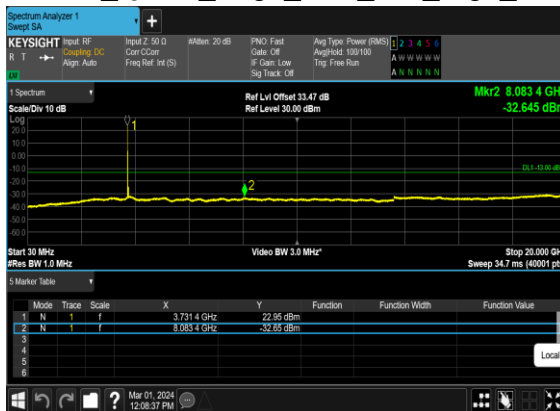
B26_N78(70M)_DFT-s- OFDM_QPSK_Edge_1RB_Left_High_CH
