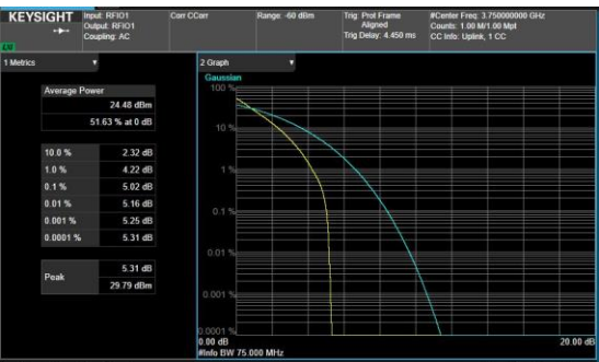
B26_N78(70M)_DFT-s-OFDM_PI_2- BPSK_Full_Mid_CH
