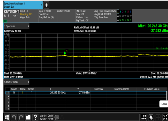
B26_N78(70M)_DFT-s- OFDM_QPSK_Edge_1RB_Left_Mid_CH
