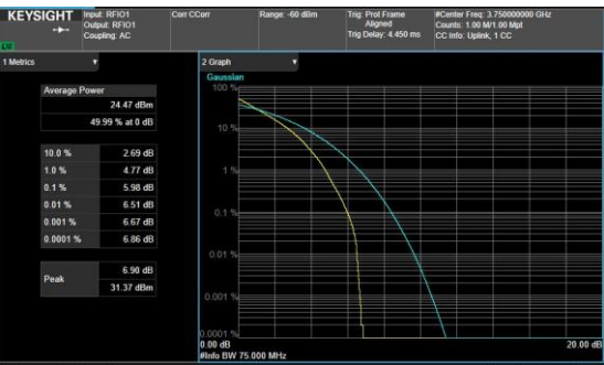
B26_N78(70M)_DFT-s-OFDM_PI_2- BPSK_1RB_Left_Mid_CH
