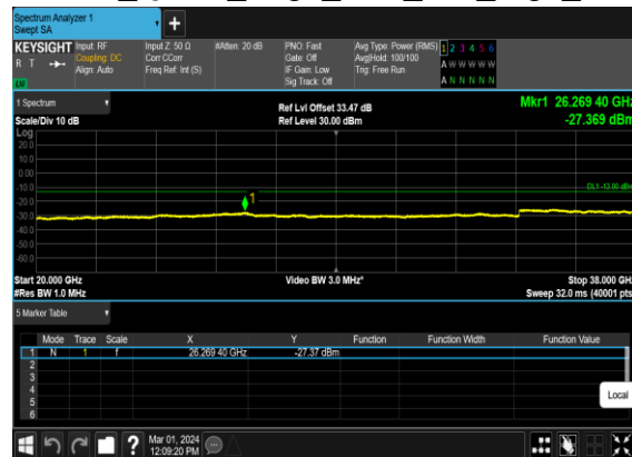
B26_N78(70M)_DFT-s- OFDM_QPSK_Edge_1RB_Left_High_CH
