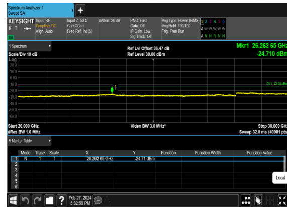
N78(70M)_CP- OFDM_QPSK_Edge_1RB_Left_High_CH
