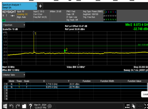
B26_N78(70M)_DFT-s-OFDM_BPSK_Edge_1RB_Left_Mid_CH
