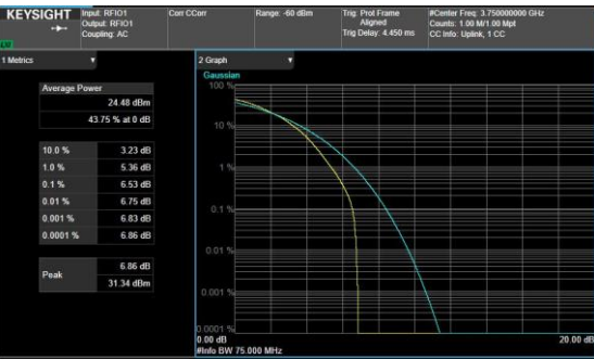
B26_N78(70M)_DFT-s- OFDM_QPSK_1RB_Left_Mid_CH
