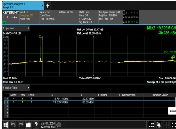
B26_N78(70M)_DFT-s- OFDM_BPSK_Edge_1RB_Left_High_CH
