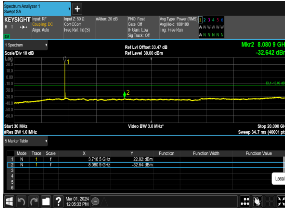
B26_N78(70M)_DFT-s- OFDM_QPSK_Edge_1RB_Left_Mid_CH
