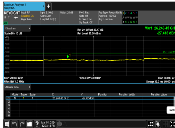
B26_N78(70M)_DFT-s-OFDM_QPSK_Edge_1RB_Left_Low_CH
