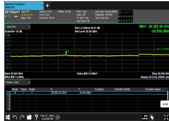
N78(70M)_CP-OFDM_16 QAM_Edge_1RB_Left_Mid_CH
