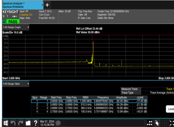
B26_N78(70M)_DFT-s- OFDM_BPSK_Edge_1RB_Left_Low_CH
