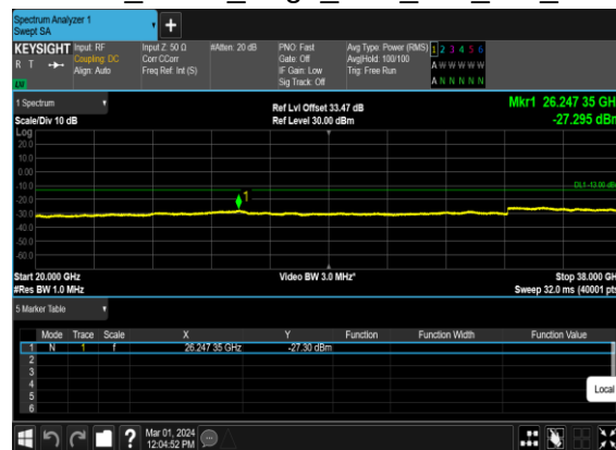
B26_N78(70M)_DFT-s-OFDM_BPSK_Edge_1RB_Left_Mid_CH
