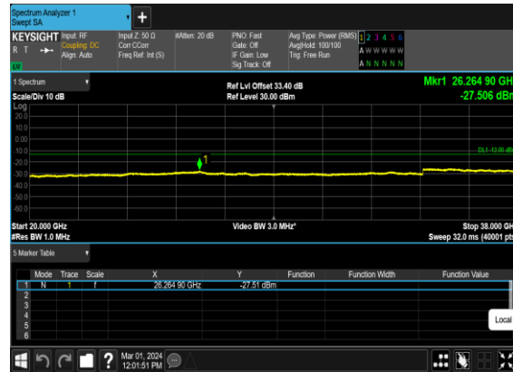
B26_N78(70M)_DFT-s-OFDM_BPSK_Edge_1RB_Left_Low_CH
