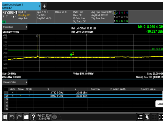
N78(70M)_CP-OFDM_16 QAM_Edge_1RB_Left_High_CH
