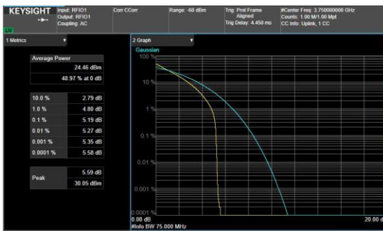
N78(70M)_CP- OFDM_QPSK_1RB_Left_Mid_CH
