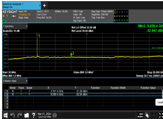
B26_N78(70M)_DFT-s-OFDM_BPSK_Edge_1RB_Left_Low_CH
