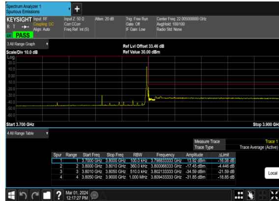
B26_N78(70M)_DFT-s- OFDM_QPSK_Edge_1RB_Right_High_CH
