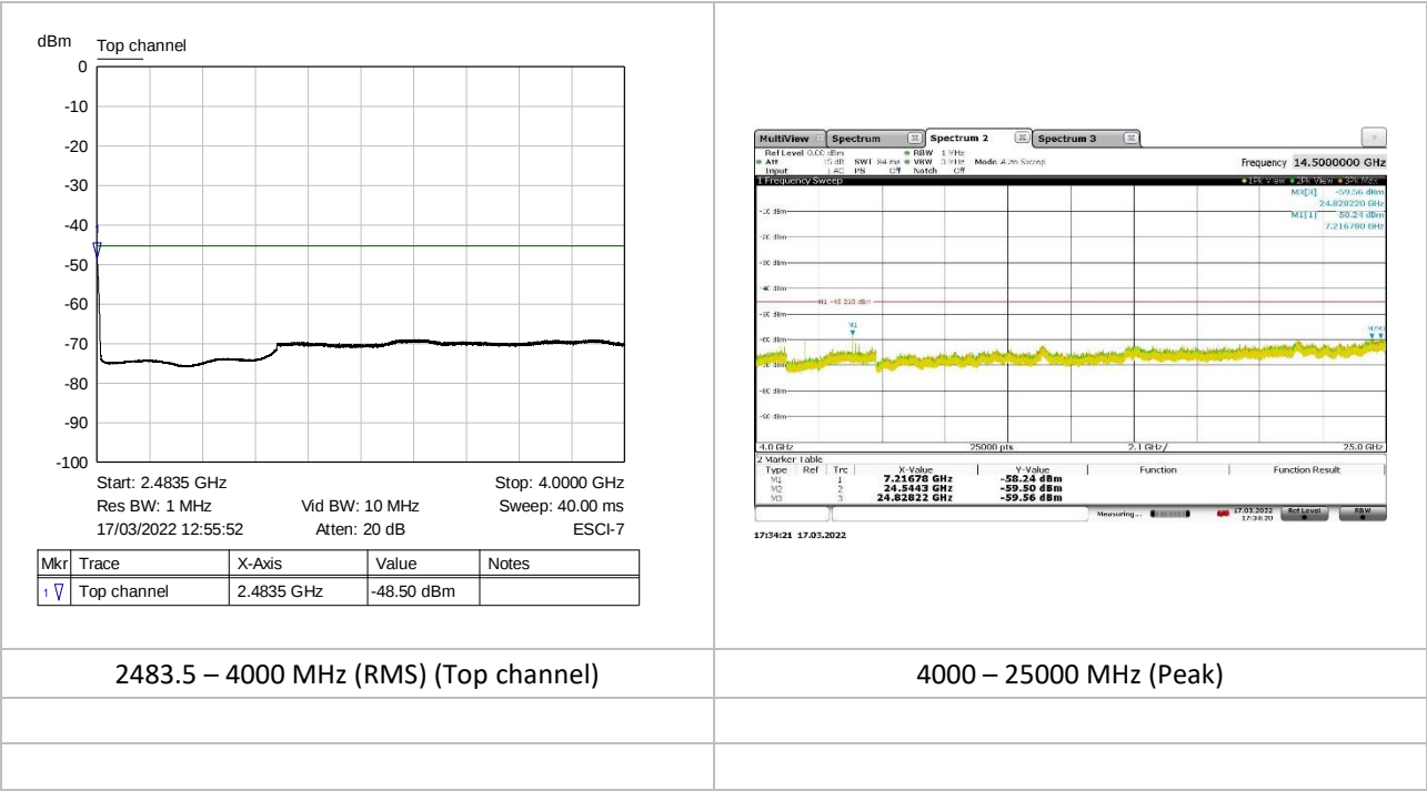
Figure 5: Emissions in restricted frequency bands
