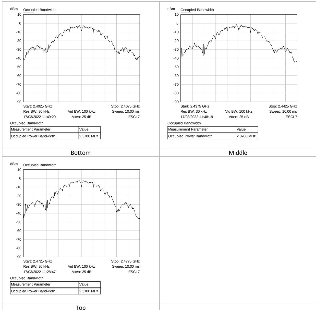
Figure 6: Occupied Bandwidth
