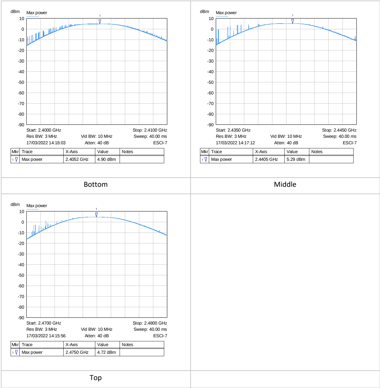
Figure 2: Peak Conducted Power plots
