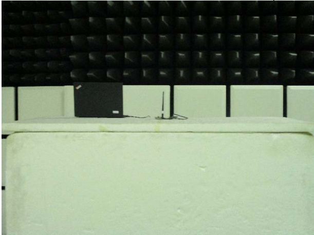
FCC_15_247_902~928MHz_OFDM_Radiated_Setup
