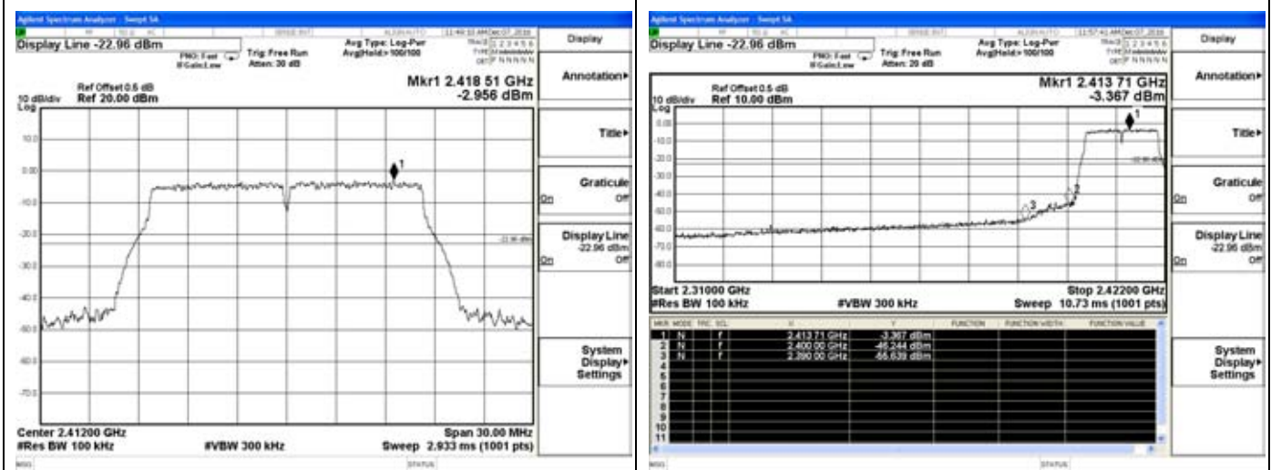
802.11g Low channel Reference
