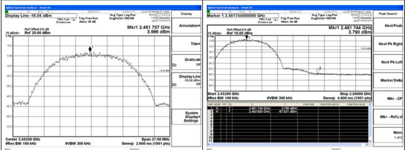
802.11b High channel Reference
