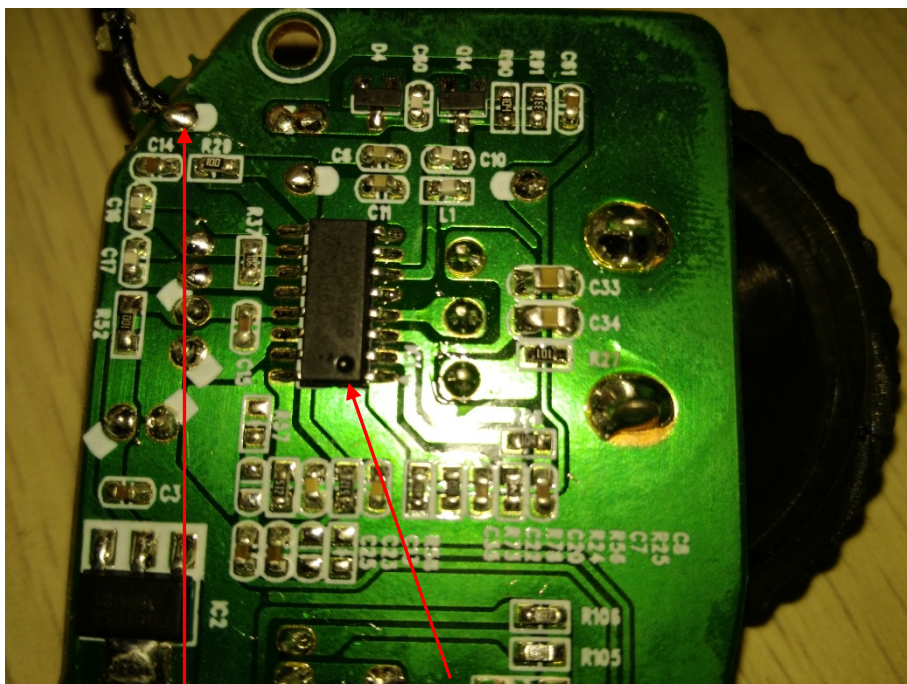
FM ANTENNA FM MODULE
