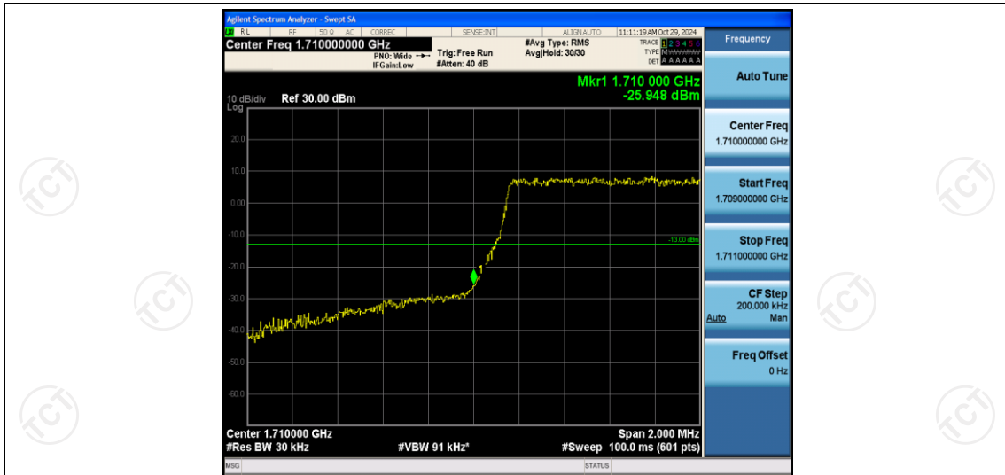
Band4-1.4MHz-QPSK-19957-6RB#0
