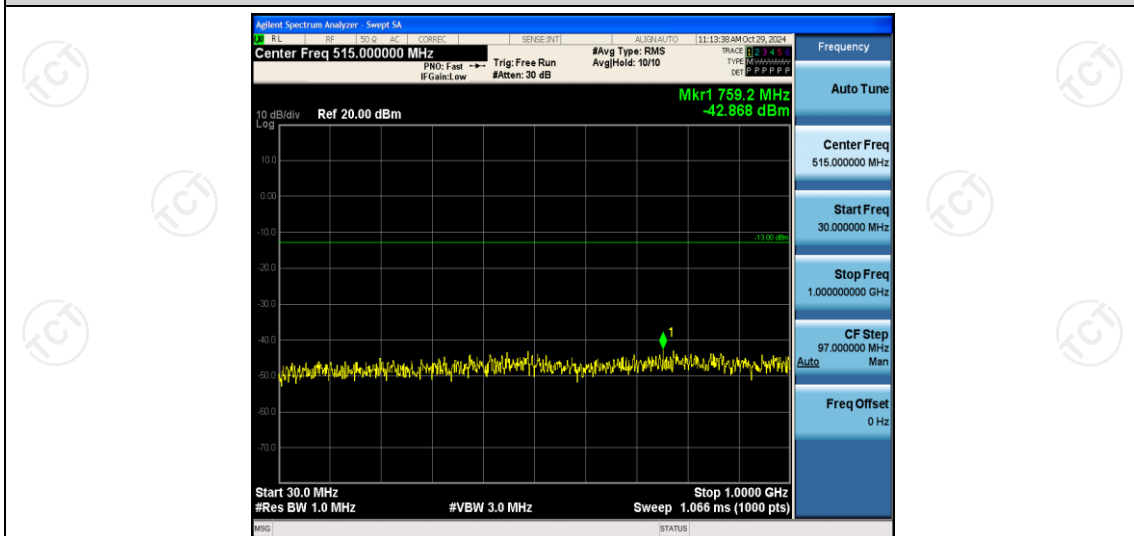
Band4-1.4MHz-QPSK-20175-1RB#0-Range1:30~1000MHz
