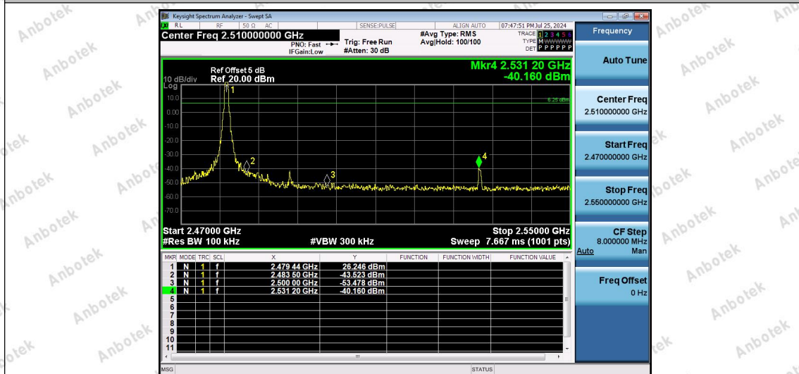
2.4G-Ant2-2479.4-PASS
