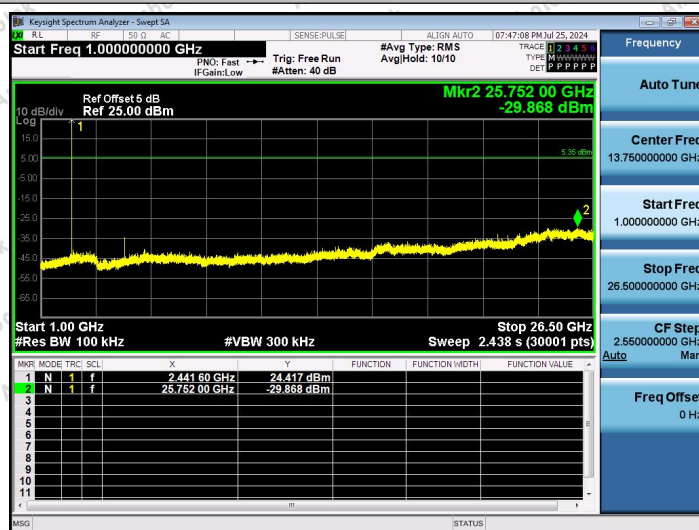
2.4G-Ant2-2441.4-1000~26500-PASS
