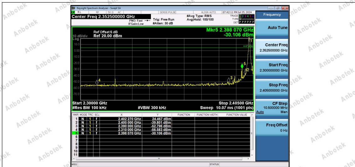
2.4G-Ant2-2402.4-PASS
