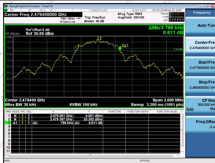
2.4G-Ant2-2479.4
