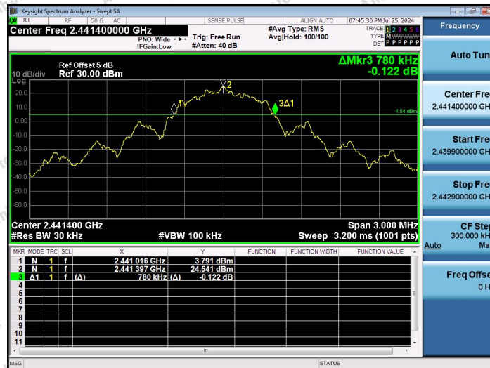
2.4G-Ant2-2441.4
