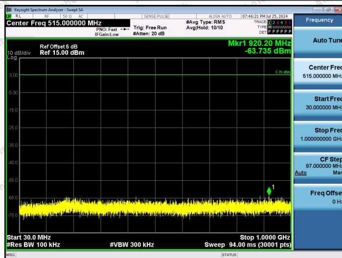
2.4G-Ant2-2441.4-30~1000-PASS
