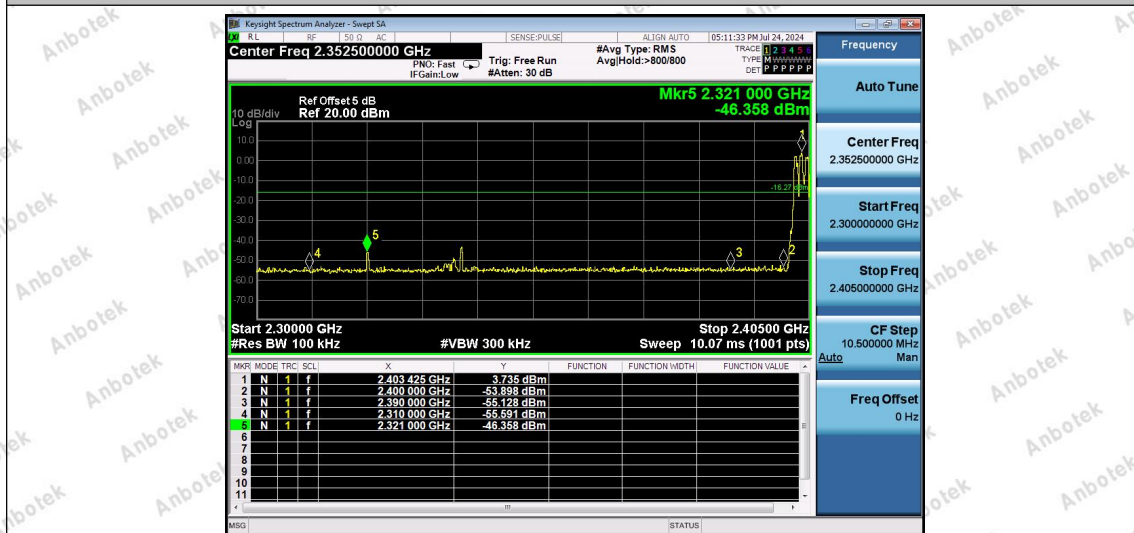
2.4G-Ant2-Hop_2402.4-PASS
