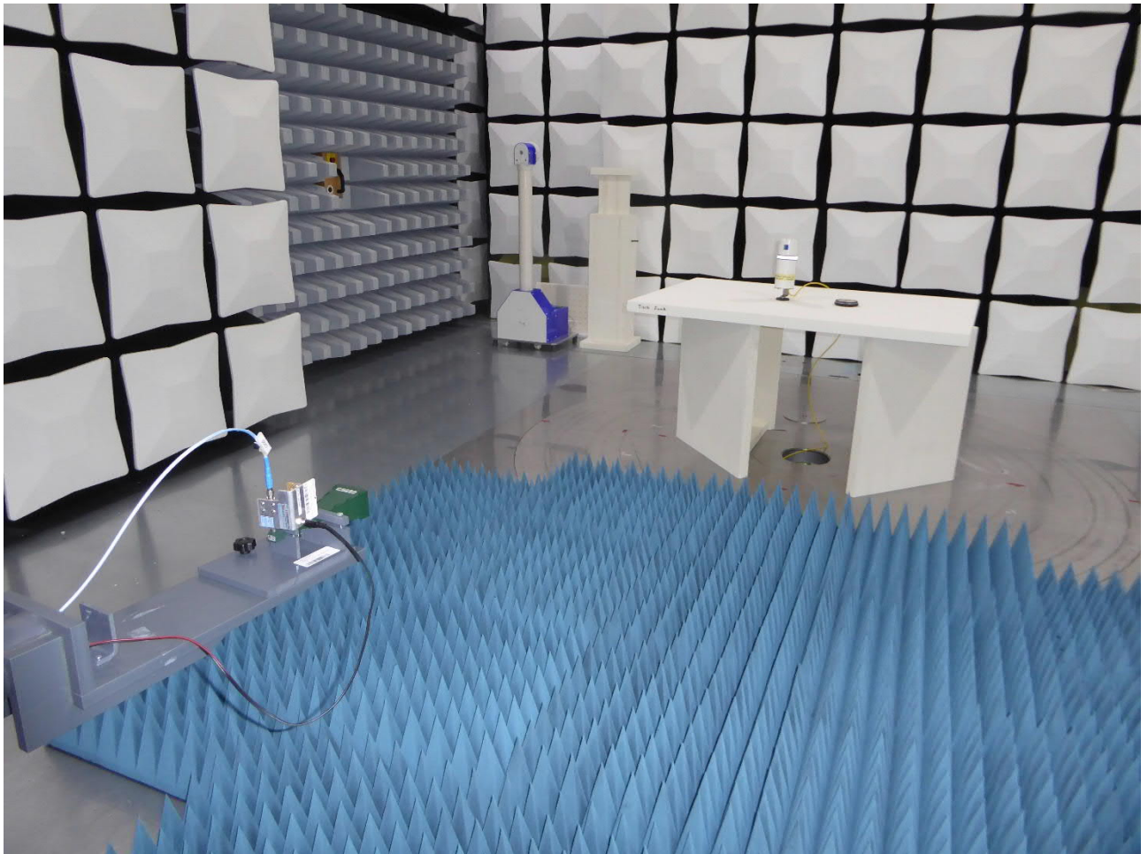
Test setup semi anechoic chamber TX spurious emissions from 18 GHz – 26.5 GHz
