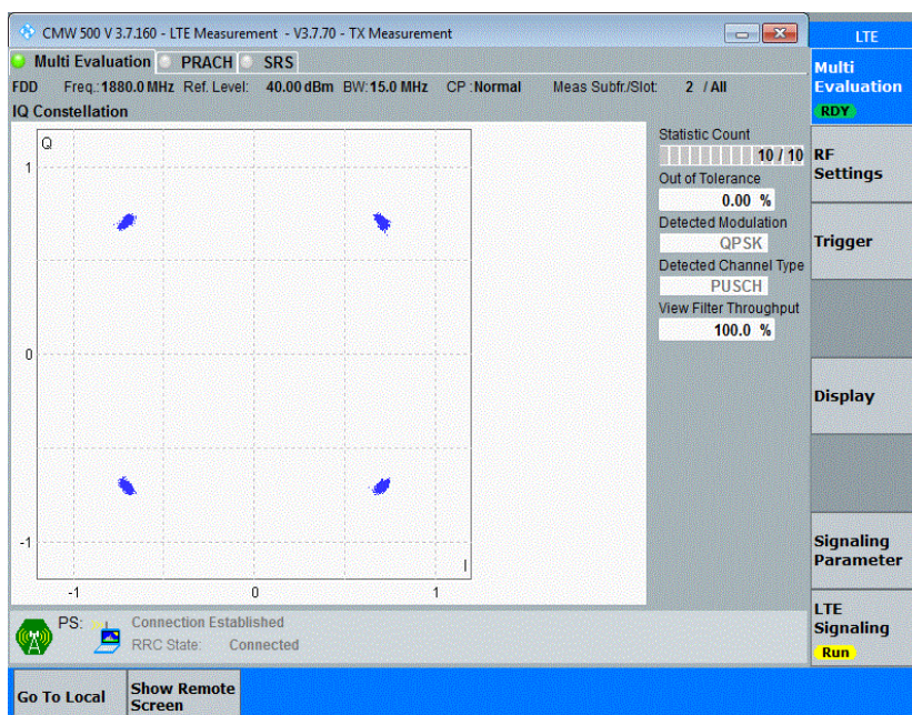
Band2-15MHz-QPSK-19125-75RB#0
