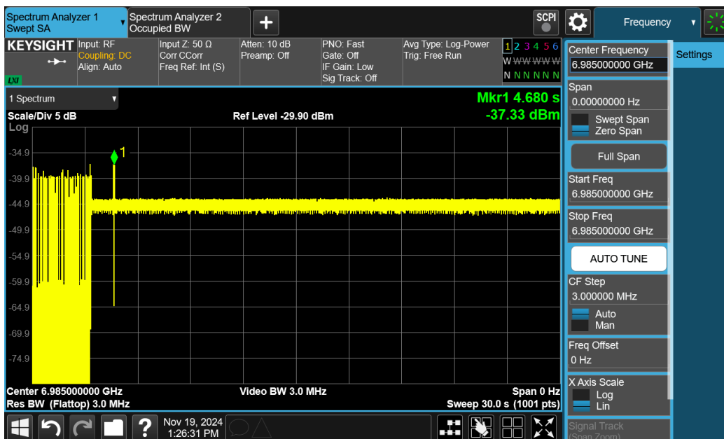
Plot 5: AWGN Signal Detection Center 160MHz
