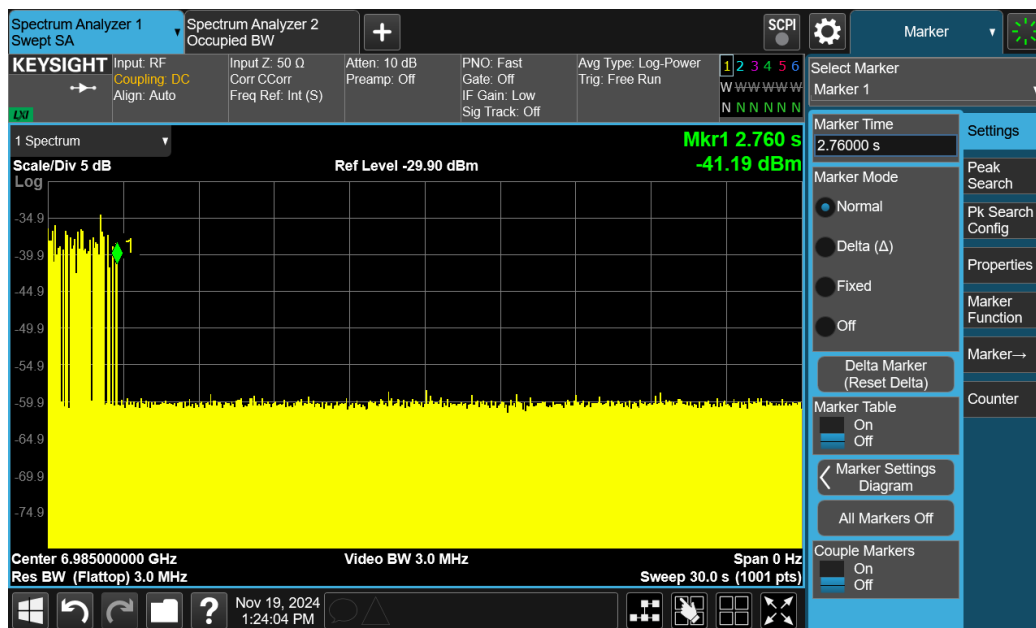
Plot 4: AWGN Signal Detection Lower Edge 160MHz
