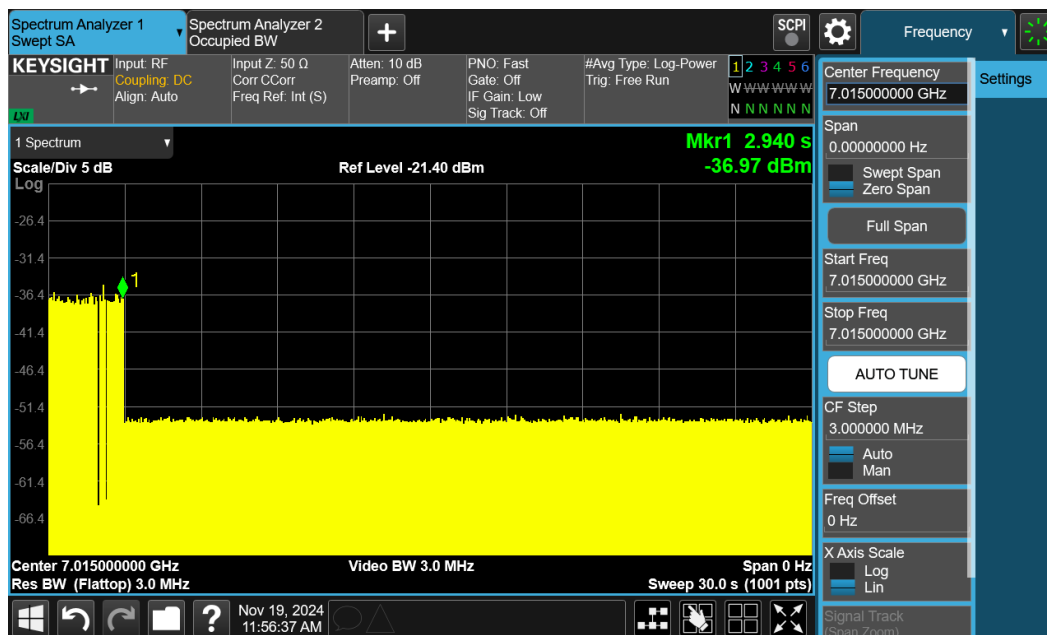
Plot 3: AWGN Signal Detection 20MHz
