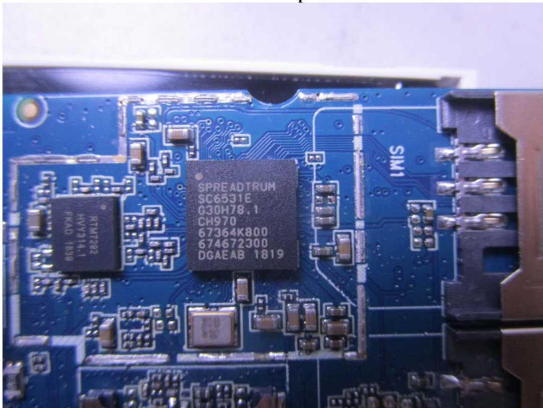
Main Chip
