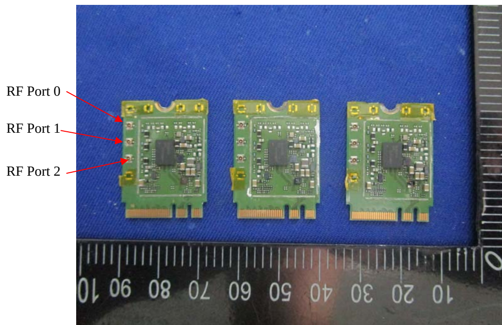
EUT –802.11ad Module Top Uncover View
