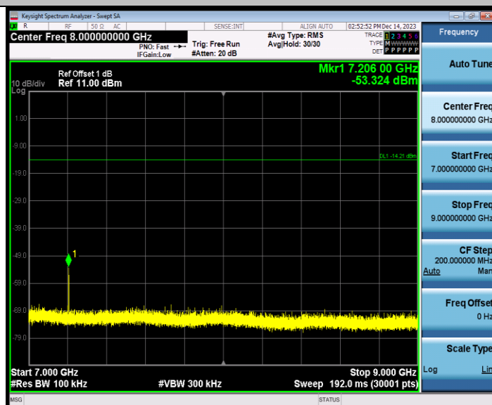
3DH5_Ant1_2402_9000~11000
