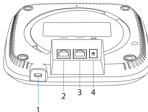
Figure 2: Rear Connectors
