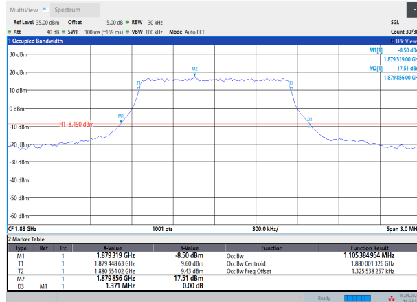
Band2-1.4MHz-QPSK-18900-6RB#0
