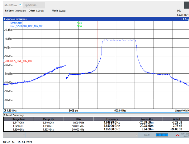
Band2-1.4MHz-QPSK-18607-6RB#0
