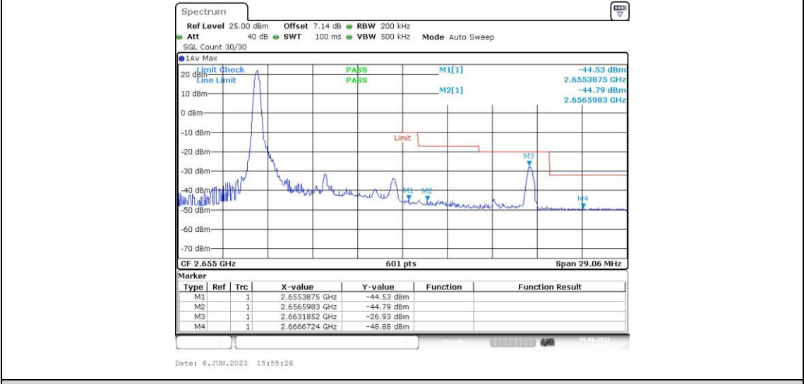
Band41-10MHz-16QAM-41190-1RB#49
