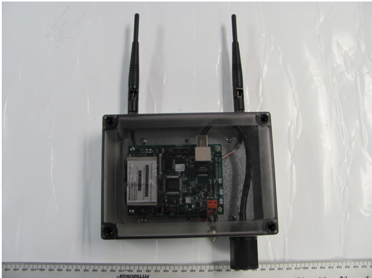
Figure 1. Front View
