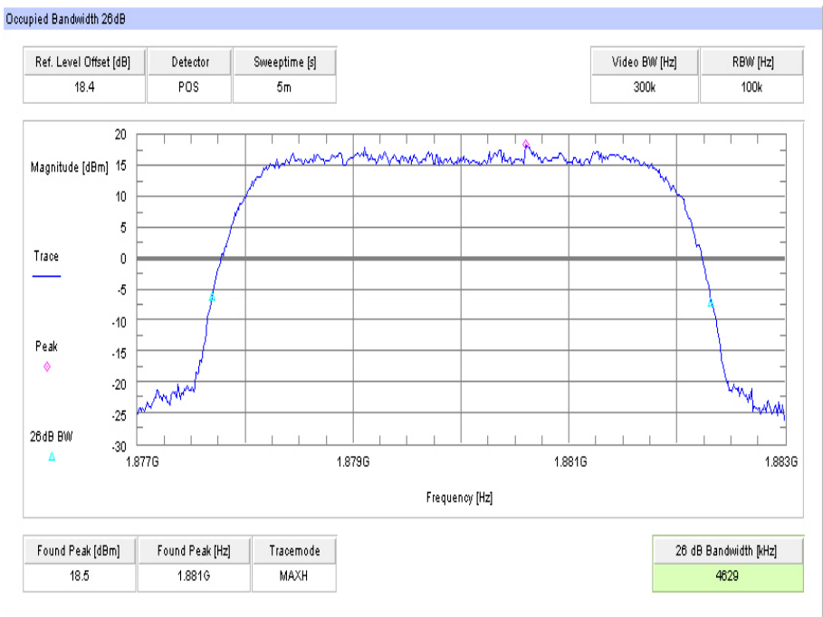
Plot 4: Channel 9400 (-26 dBc BW)
