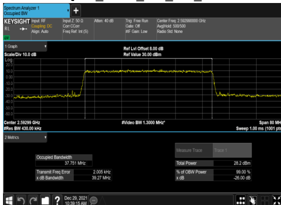
B4_N41(40M)_CP-OFDM_64 QAM_Outer_Full_Mid_CH
