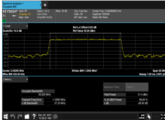
B4_N41(40M)_DFT-s-OFDM_PI_2- BPSK_Outer_Full_Mid_CH
