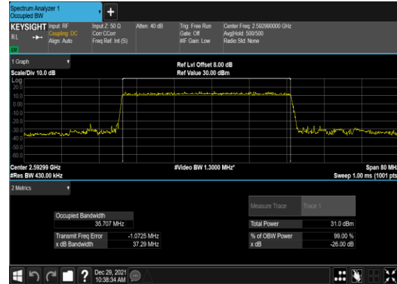
B4_N41(40M)_DFT-s- OFDM_QPSK_Outer_Full_Mid_CH
