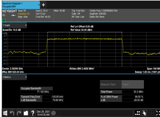
B4_N41(80M)_DFT-s-OFDM_PI_2- BPSK_Outer_Full_Mid_CH
