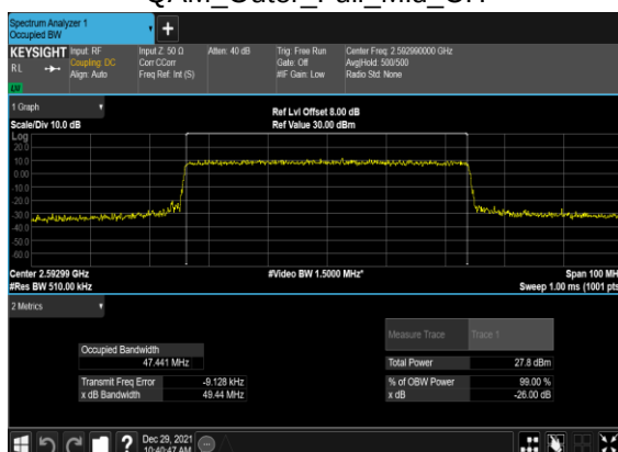
B4_N41(50M)_CP-OFDM_64 QAM_Outer_Full_Mid_CH
