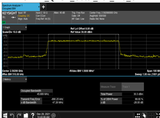
B4_N41(50M)_DFT-s- OFDM_QPSK_Outer_Full_Mid_CH
