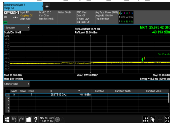
B4_N41(20M)_DFT-s- OFDM_QPSK_Edge_1RB_Left_High_CH
