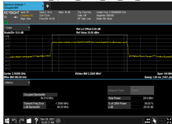
B4_N41(70M)_DFT-s- OFDM_QPSK_Outer_Full_Mid_CH
