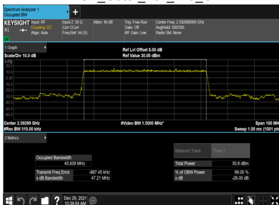
B4_N41(50M)_DFT-s-OFDM_PI_2- BPSK_Outer_Full_Mid_CH
