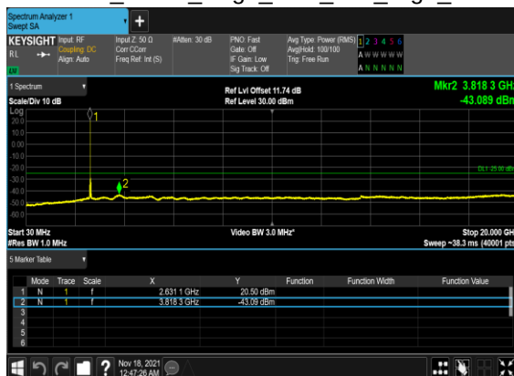
B4_N41(60M)_DFT-s- OFDM_BPSK_Edge_1RB_Left_High_CH
