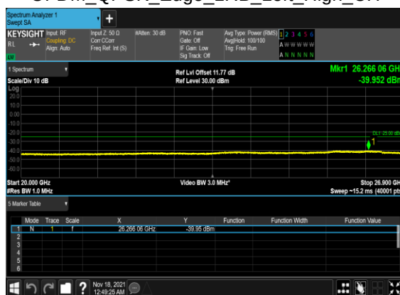
B4_N41(60M)_DFT-s- OFDM_QPSK_Edge_1RB_Left_High_CH
