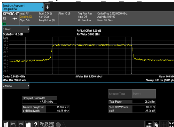
B4_N41(50M)_CP- OFDM_QPSK_Outer_Full_Mid_CH
