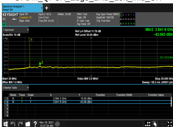
B4_N41(20M)_DFT-s- OFDM_QPSK_Edge_1RB_Left_Mid_CH
