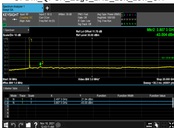
B4_N41(60M)_DFT-s- OFDM_QPSK_Edge_1RB_Left_Low_CH
