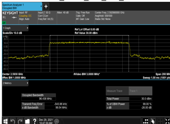
B4_N41(100M)_DFT-s-OFDM_PI_2- BPSK_Outer_Full_Mid_CH
