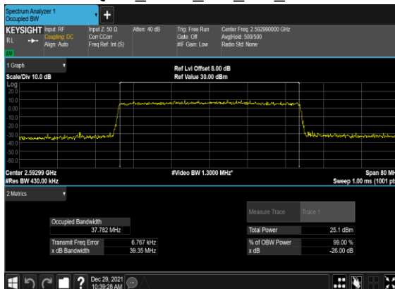
B4_N41(40M)_CP-OFDM_256 QAM_Outer_Full_Mid_CH
