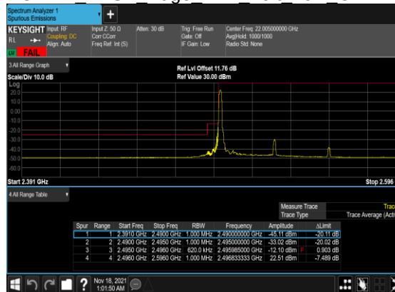
B4_N41(60M)_DFT-s- OFDM_BPSK_Edge_1RB_Left_Low_CH
