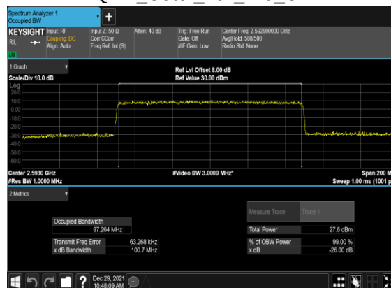
B4_N41(100M)_CP-OFDM_16 QAM_Outer_Full_Mid_CH
