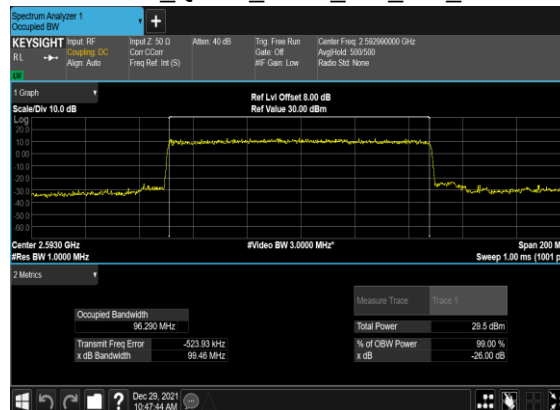
B4_N41(100M)_DFT-s- OFDM_QPSK_Outer_Full_Mid_CH
