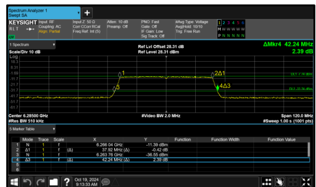
Figure 80 - 802.11ax HE40 SU VLP Maximum 26 dB EBW
