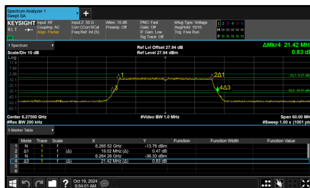
Figure 126 - 802.11ax HE20 SU VLP Maximum 26 dB EBW
