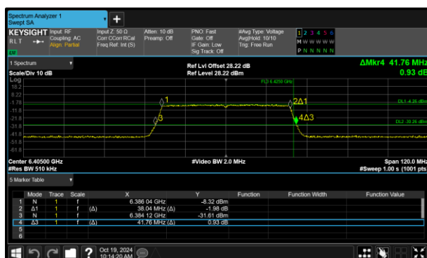
Figure 127 - 802.11ax HE40 SU VLP Minimum 26 dB EBW
