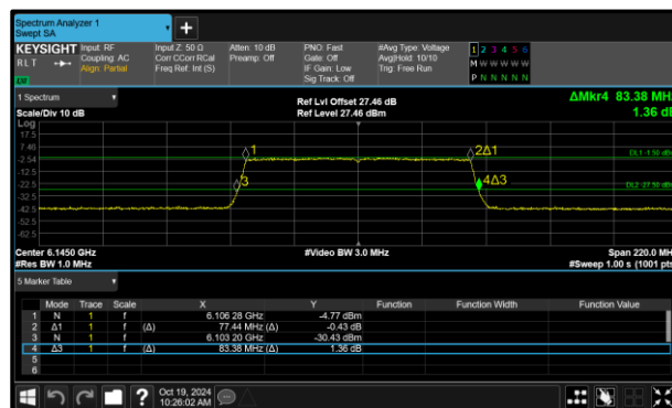
Figure 130 - 802.11ax HE80 SU VLP Maximum 26 dB EBW
