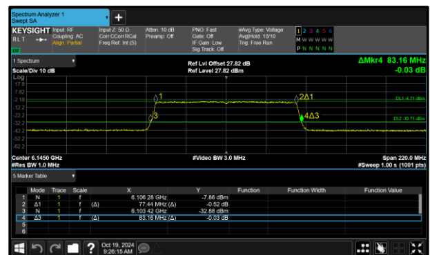
Figure 82 - 802.11ax HE80 SU VLP Maximum 26 dB EBW
