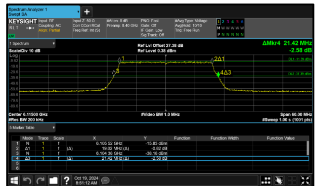
Figure 78 - 802.11ax HE20 SU VLP Maximum 26 dB EBW
