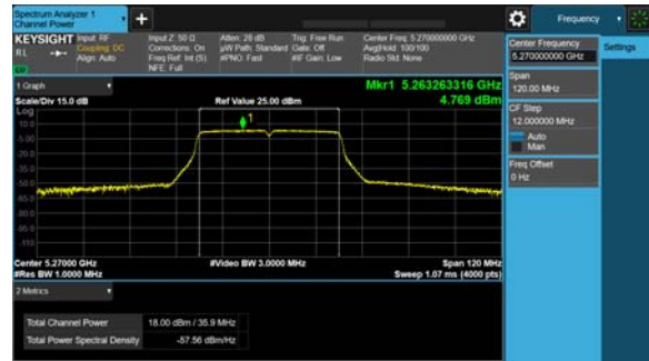
Antenna B
