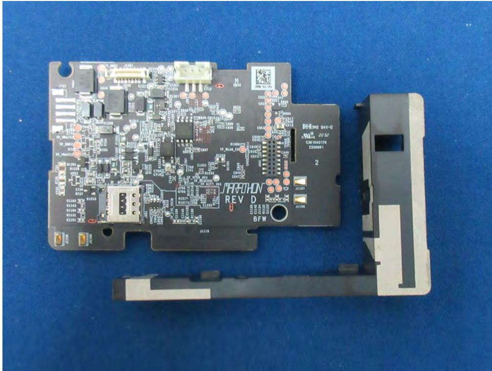
(12) EUT Photo (WWAN+GPS Antenna)
