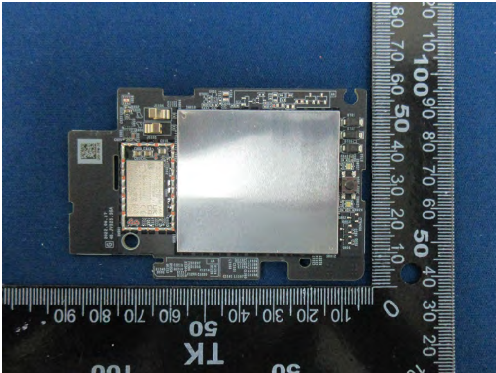
(10) EUT Photo (BT LE+WiFi Antenna)
