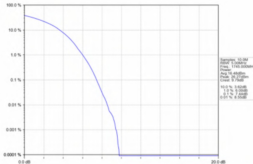
Band66_20MHz_16QAM_MCH_1745MHz_RB_100_0_NTNV
