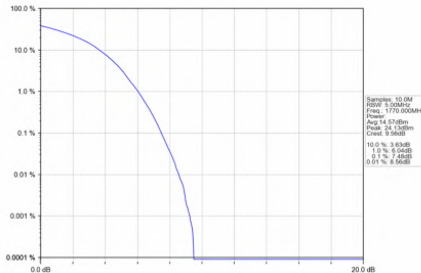
Band66_20MHz_256QAM_HCH_1770MHz_RB_100_0_NTNV
