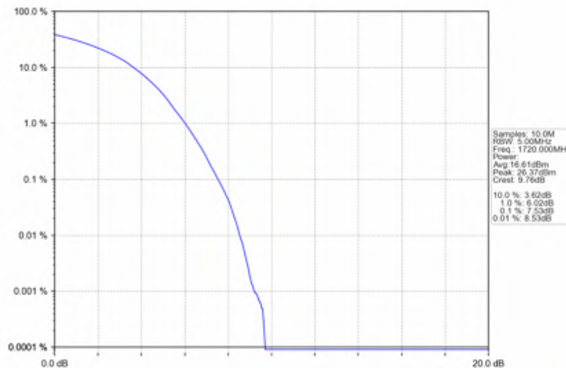
Band66_20MHz_64QAM_LCH_1720MHz_RB_100_0_NTNV
