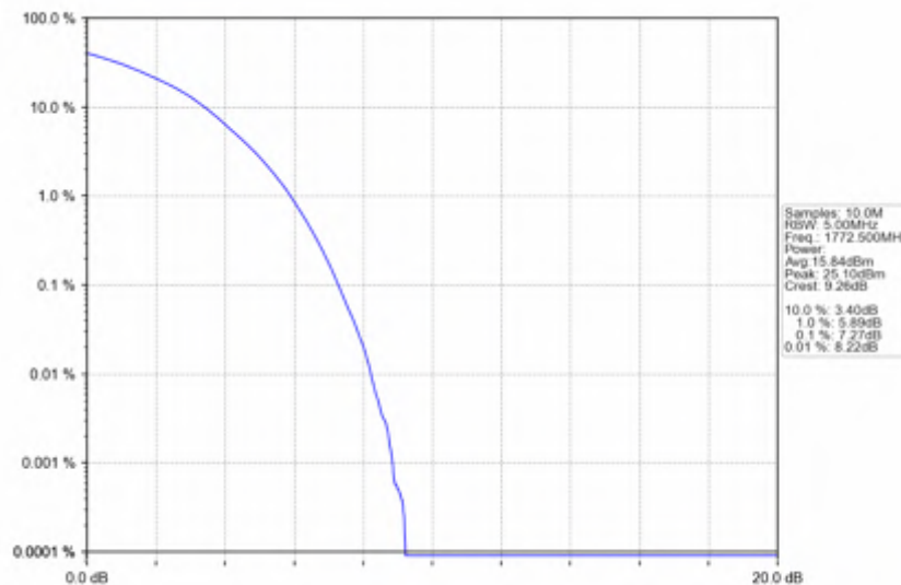
Band66_15MHz_256QAM_HCH_1772.5MHz_RB_75_0_NTNV
