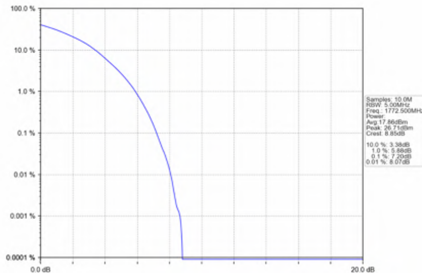
Band66_15MHz_64QAM_HCH_1772.5MHz_RB_75_0_NTNV
