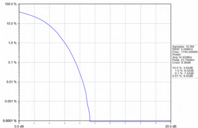
Band66_20MHz_256QAM_MCH_1745MHz_RB_100_0_NTNV
