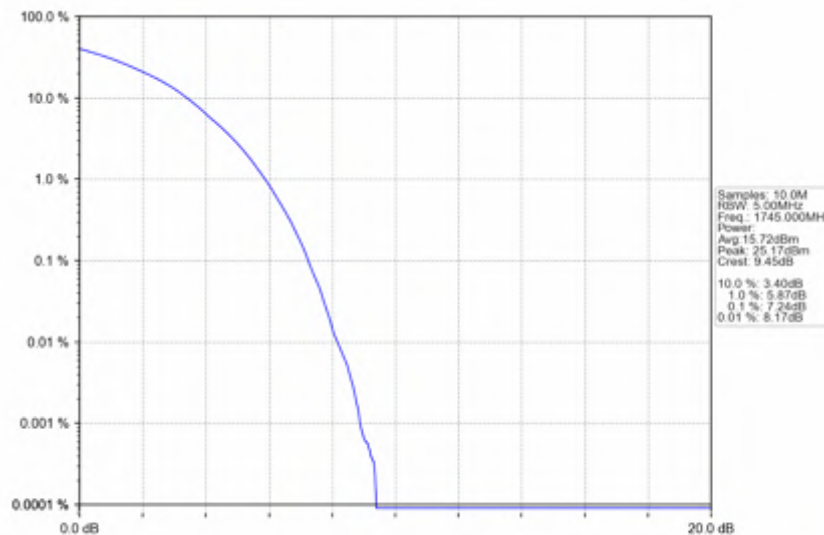
Band66_15MHz_256QAM_MCH_1745MHz_RB_75_0_NTNV
