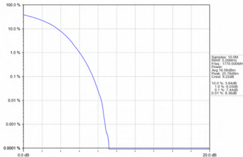
Band66_20MHz_64QAM_HCH_1770MHz_RB_100_0_NTNV
