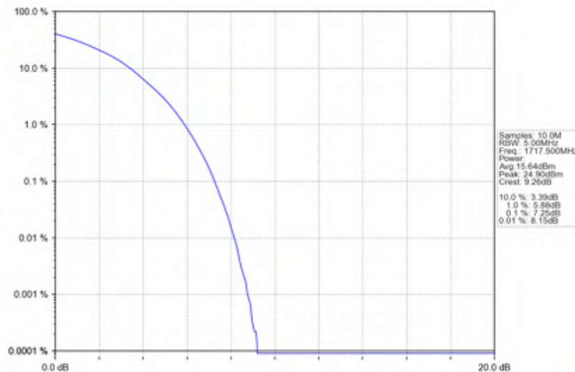
Band66_15MHz_256QAM_LCH_1717.5MHz_RB_75_0_NTNV
