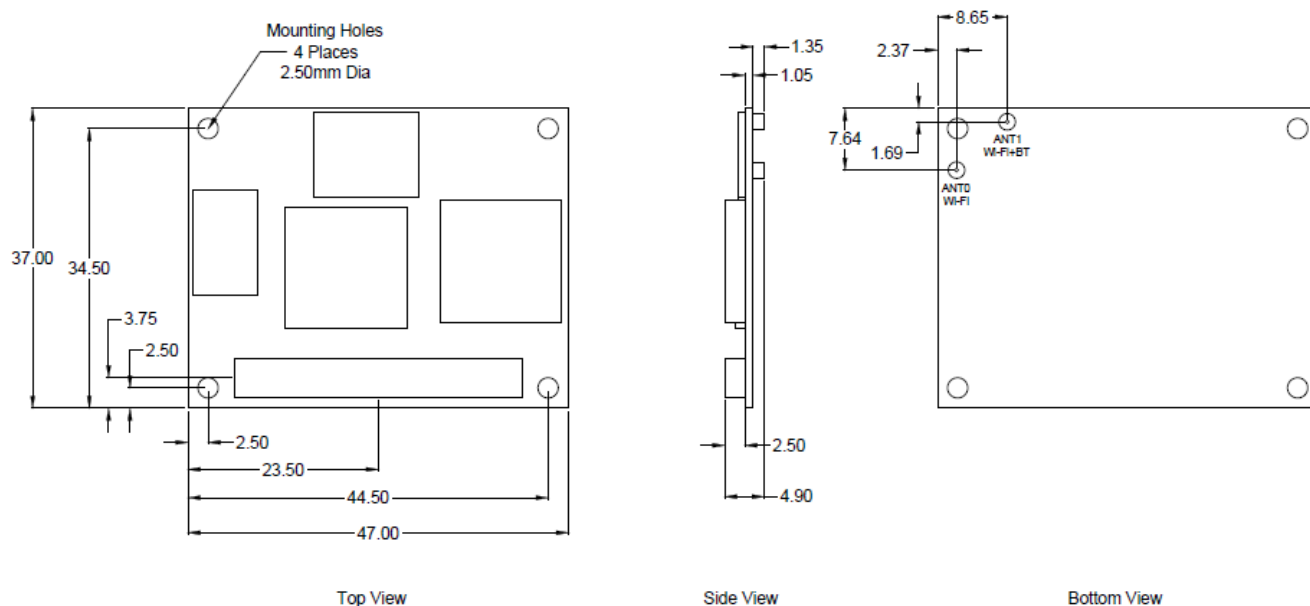
Figure 1: WB50NBT mechanical drawing
