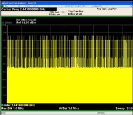
Number of Pulses in 31.6 seconds 8DPSK_3-DH5
