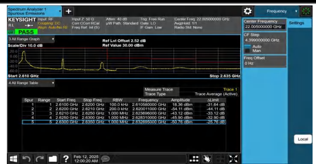
Band38-10MHz-QPSK-38200-1RB#0-PASS
