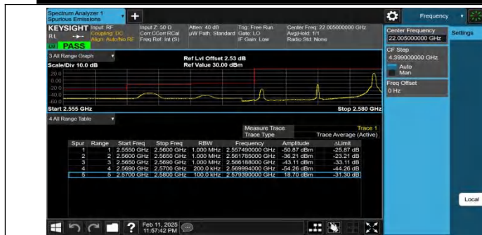
Band38-10MHz-QPSK-37800-1RB#49-PASS
