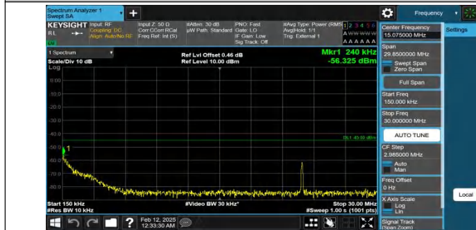
Band38-15MHz-QPSK-37825-1RB#74-0.15~30-PASS
