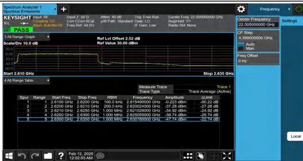
Band38-10MHz-QPSK-38200-50RB#0-PASS
