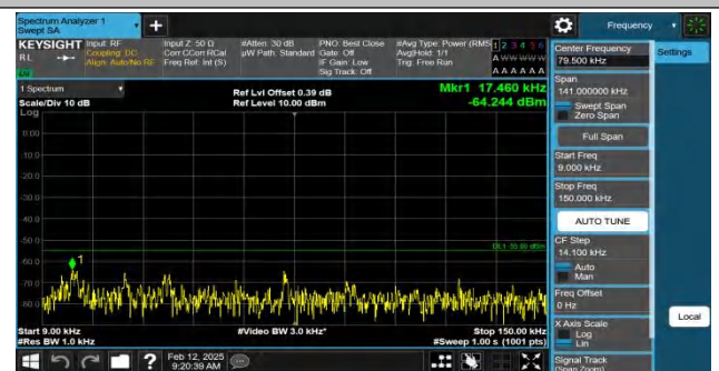
Band38-15MHz-QPSK-38175-1RB#74-0.009~0.15-PASS
