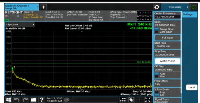
Band38-15MHz-QPSK-38175-1RB#0-0.15~30-PASS
