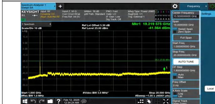
Band38-15MHz-QPSK-37825-1RB#74-1000~20000-PASS
