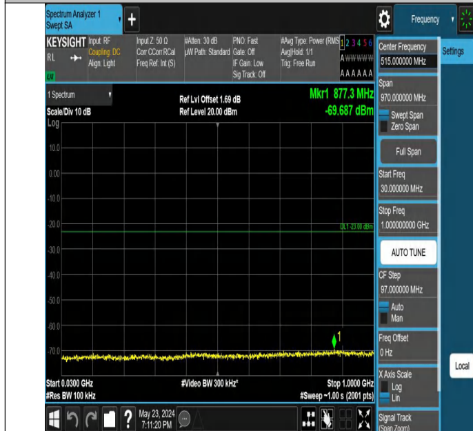
Band66_5MHz_QPSK_131997_1RB#0_30~1000_30~1000
