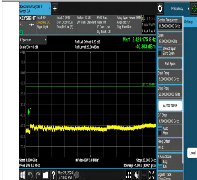
Band66_10MHz_QPSK_132022_1RB#0_3000~20000_3000~200
