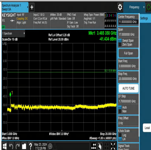
Band66_5MHz_QPSK_132322_1RB#0_3000~20000_3000~2000
