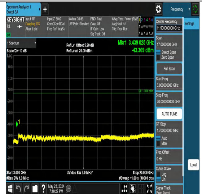
Band66_10MHz_QPSK_132022_1RB#49_3000~20000_3000~200
