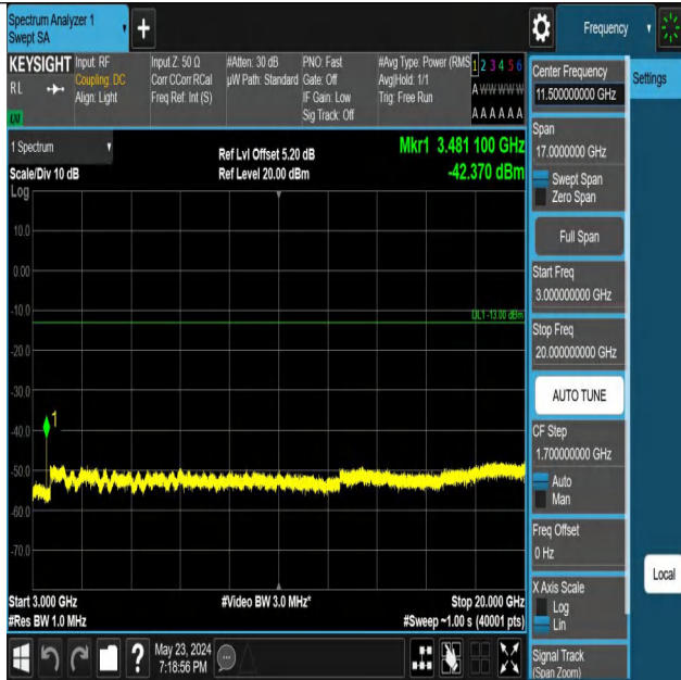
Band66_10MHz_QPSK_132322_1RB#0_3000~20000_3000~20000
