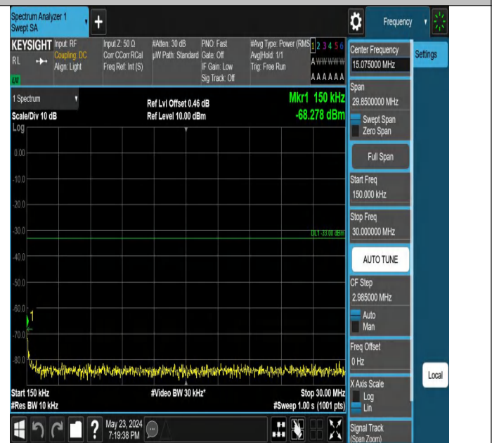
Band66_10MHz_QPSK_132622_1RB#0_0.15~30_0.15~30
