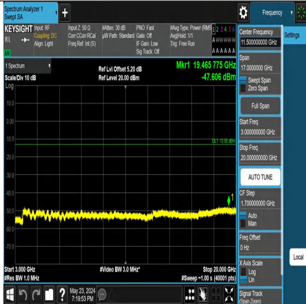
Band66_10MHz_QPSK_132622_1RB#0_3000~20000_3000~200
