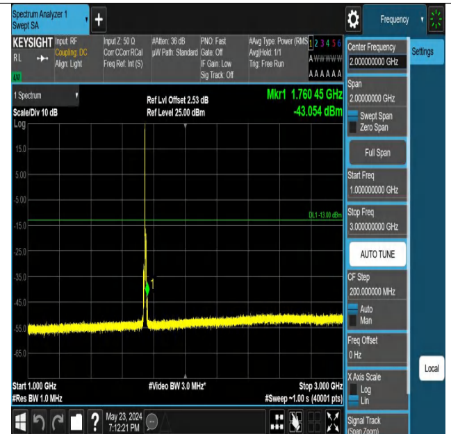
Band66_5MHz_QPSK_132322_1RB#0_1000~3000_1000~3000
