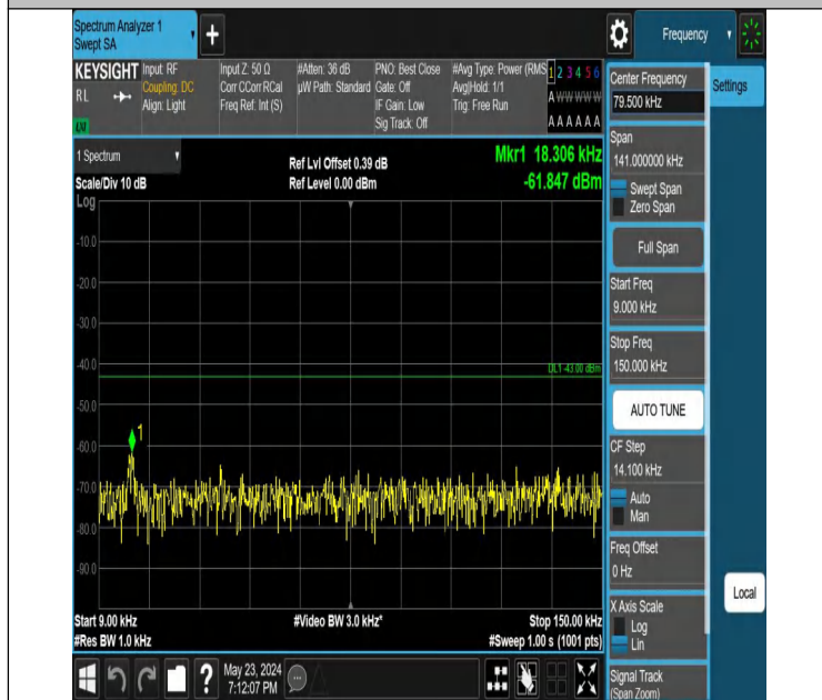
Band66_5MHz_QPSK_132322_1RB#0_0.009~0.15_0.009~0.15
