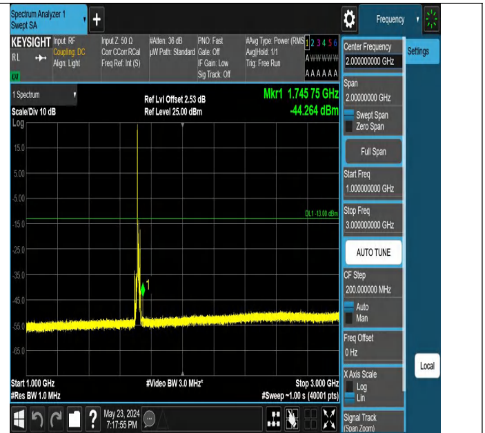
Band66_10MHz_QPSK_132022_1RB#0_1000~3000_1000~3000
