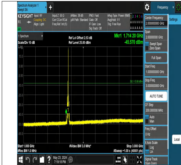
Band66_10MHz_QPSK_132322_1RB#49_1000~3000_1000~300
