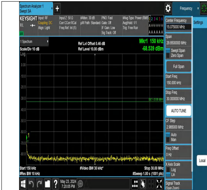
Band66_10MHz_QPSK_132622_1RB#49_0.15~30_0.15~30
