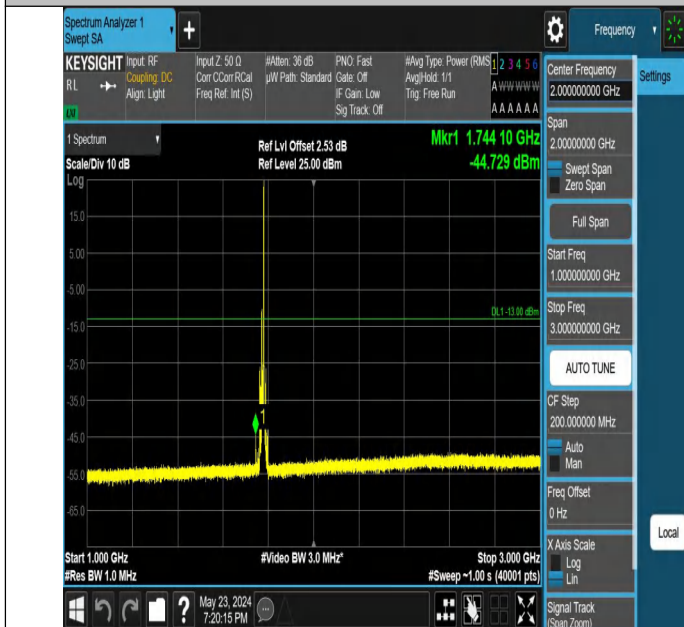
Band66_10MHz_QPSK_132622_1RB#49_1000~3000_1000~300
