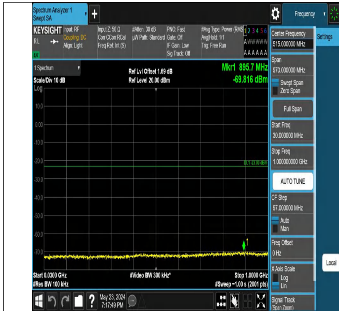
Band66_10MHz_QPSK_132022_1RB#0_30~1000_30~1000
