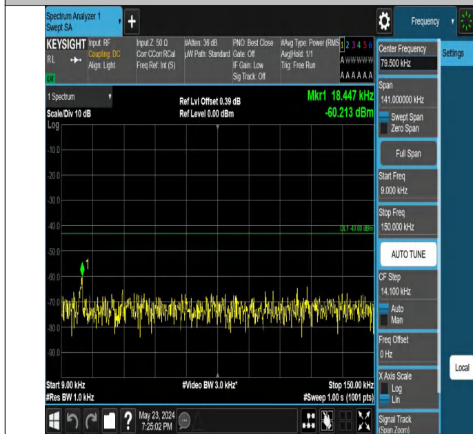
Band66_15MHz_QPSK_132322_1RB#0_0.009~0.15_0.009~0.15
