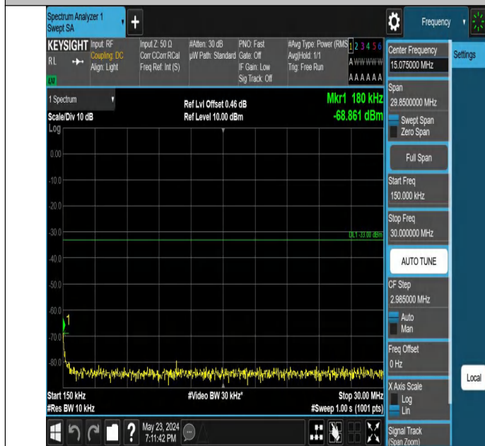
Band66_5MHz_QPSK_131997_1RB#24_0.15~30_0.15~30
