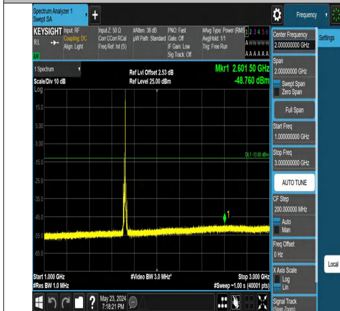
Band66_10MHz_QPSK_132022_1RB#49_1000~3000_1000~300
