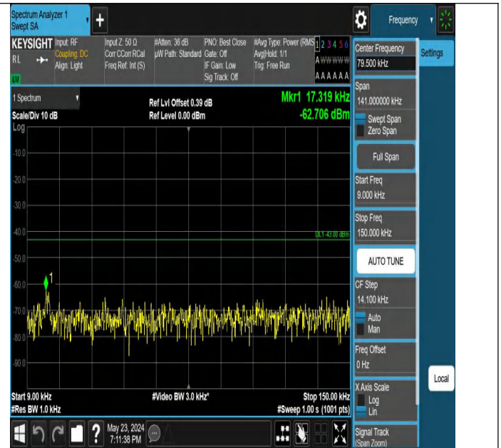
Band66_5MHz_QPSK_131997_1RB#24_0.009~0.15_0.009~0.15
