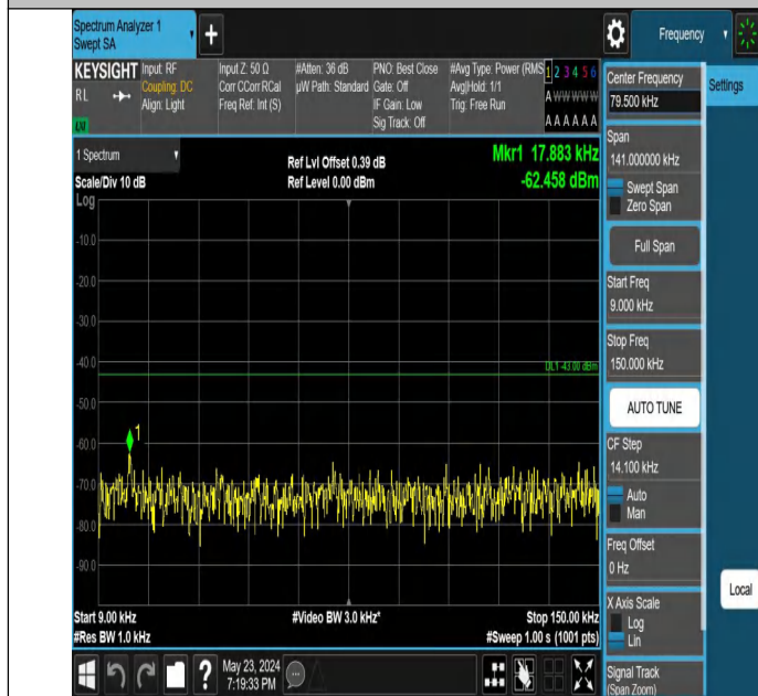
Band66_10MHz_QPSK_132622_1RB#0_0.009~0.15_0.009~0.15
