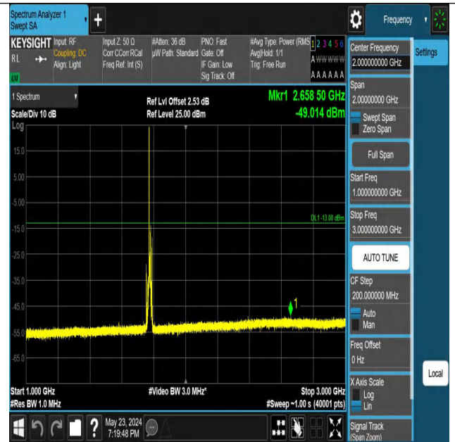
Band66_10MHz_QPSK_132622_1RB#0_1000~3000_1000~3000
