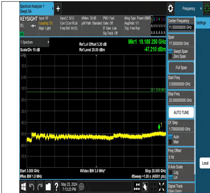
Band66_5MHz_QPSK_132647_1RB#0_3000~20000_3000~2000
