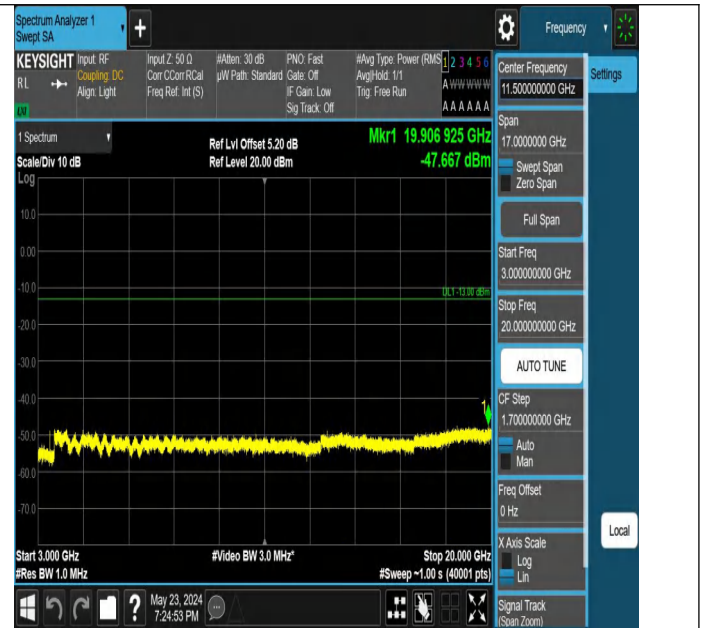
Band66_15MHz_QPSK_132047_1RB#74_3000~20000_3000~2000
