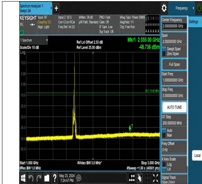
Band66_15MHz_QPSK_132047_1RB#74_1000~3000_1000~3000
