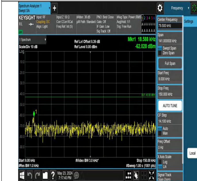
Band66_10MHz_QPSK_132022_1RB#0_0.009~0.15_0.009~0.15
