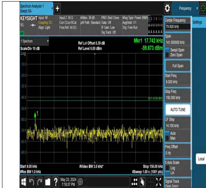
Band66_10MHz_QPSK_132322_1RB#0_0.009~0.15_0.009~0.15
