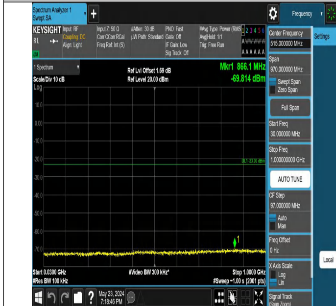
Band66_10MHz_QPSK_132322_1RB#0_30~1000_30~1000
