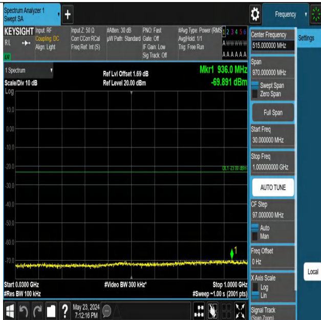
Band66_5MHz_QPSK_132322_1RB#0_30~1000_30~1000
