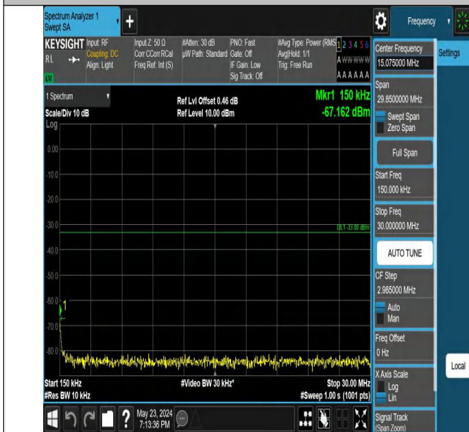
Band66_5MHz_QPSK_132647_1RB#24_0.15~30_0.15~30
