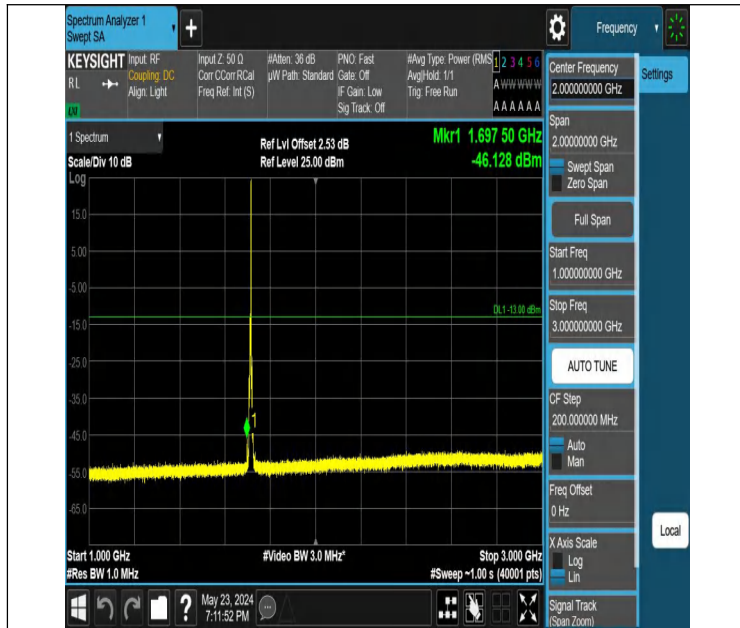
Band66_5MHz_QPSK_131997_1RB#24_1000~3000_1000~3000
