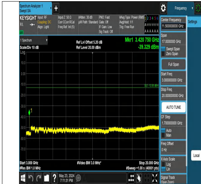
Band66_5MHz_QPSK_131997_1RB#0_3000~20000_3000~2000
