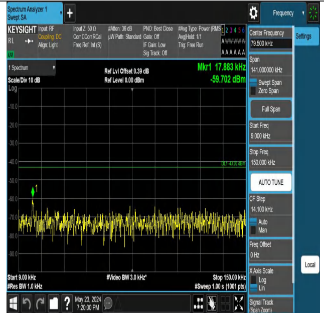
Band66_10MHz_QPSK_132622_1RB#49_0.009~0.15_0.009~0.15
