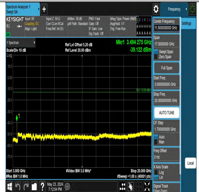
Band66_5MHz_QPSK_132322_1RB#24_3000~20000_3000~2000
