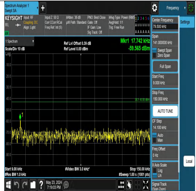
Band66_10MHz_QPSK_132322_1RB#49_0.009~0.15_0.009~0.15
