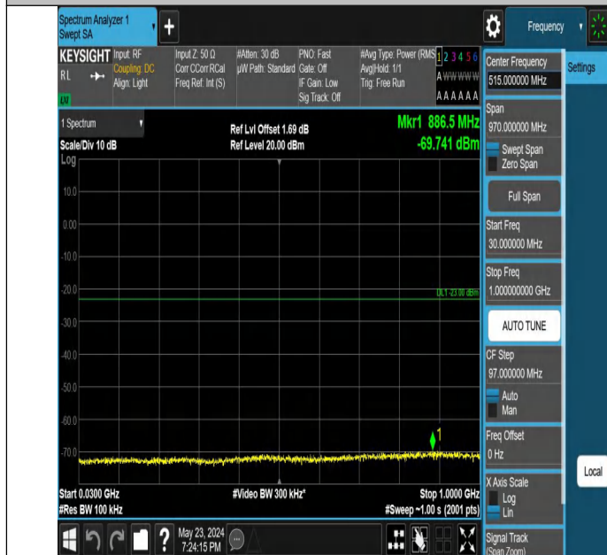
Band66_15MHz_QPSK_132047_1RB#0_30~1000_30~1000
