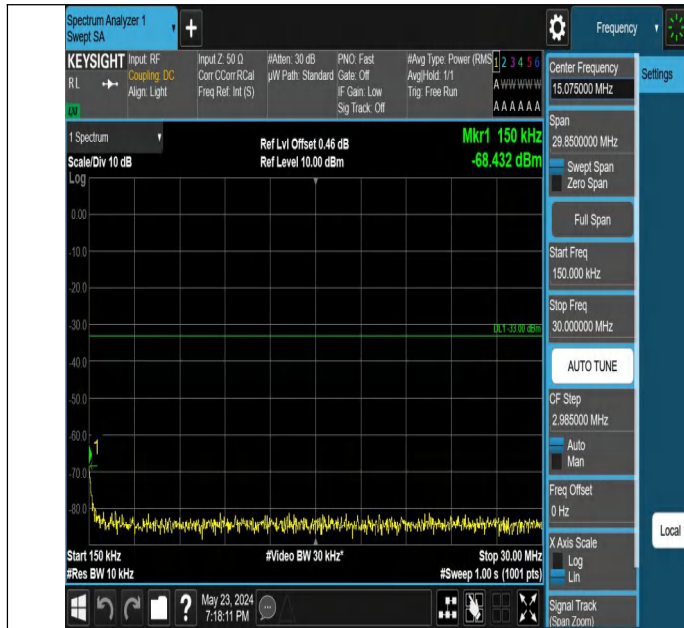
Band66_10MHz_QPSK_132022_1RB#49_0.15~30_0.15~30
