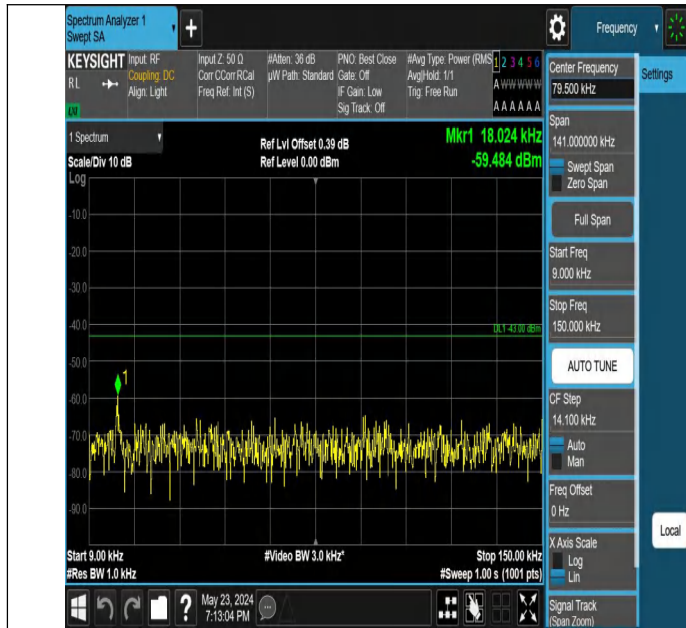
Band66_5MHz_QPSK_132647_1RB#0_0.009~0.15_0.009~0.15
