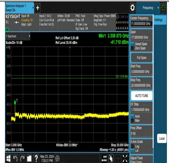
Band66_10MHz_QPSK_132622_1RB#49_3000~20000_3000~200
