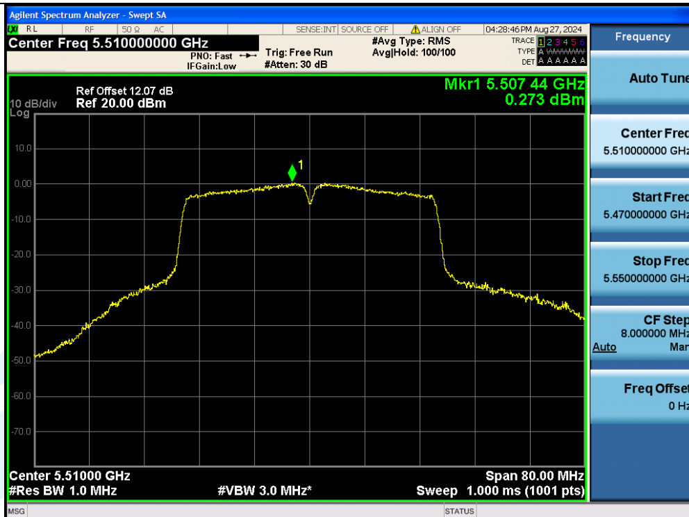
11AC40MIMO-Ant3-5510-PASS
