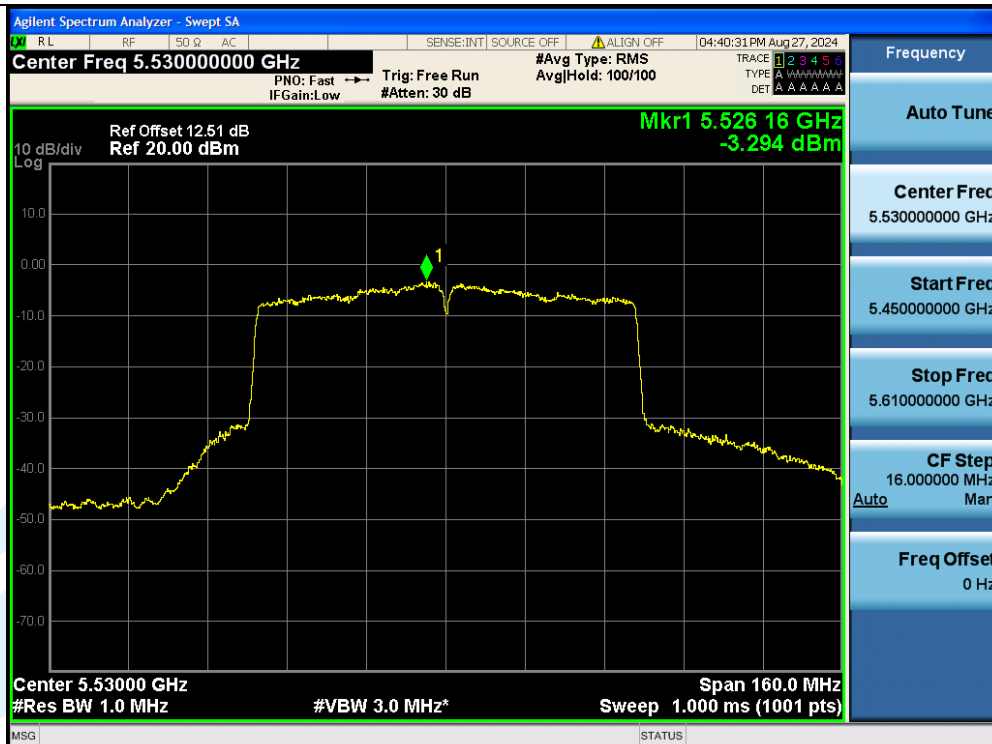
11AC80MIMO-Ant3-5530-PASS
