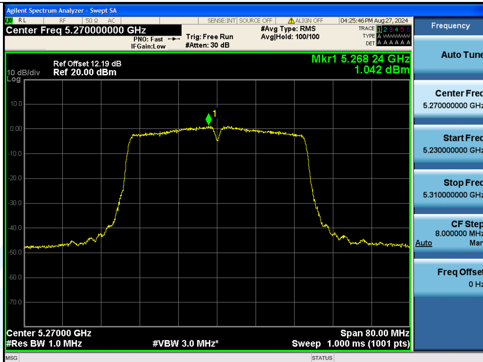
11AC40MIMO-Ant3-5270-PASS
