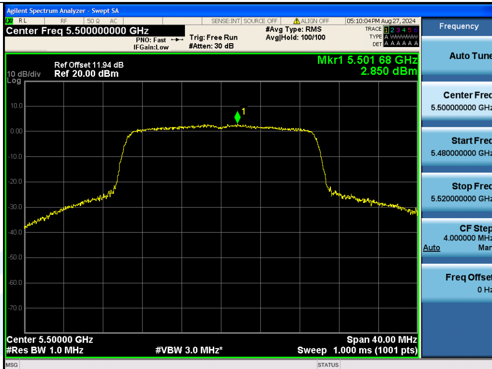
11AX20MIMO-Ant3-5500-PASS
