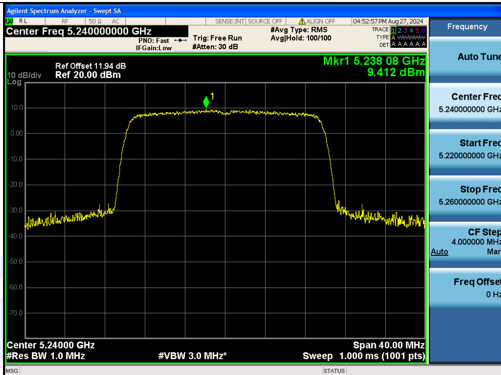
11AX20MIMO-Ant3-5240-PASS
