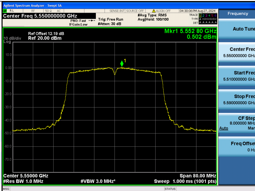
11AC40MIMO-Ant3-5550-PASS
