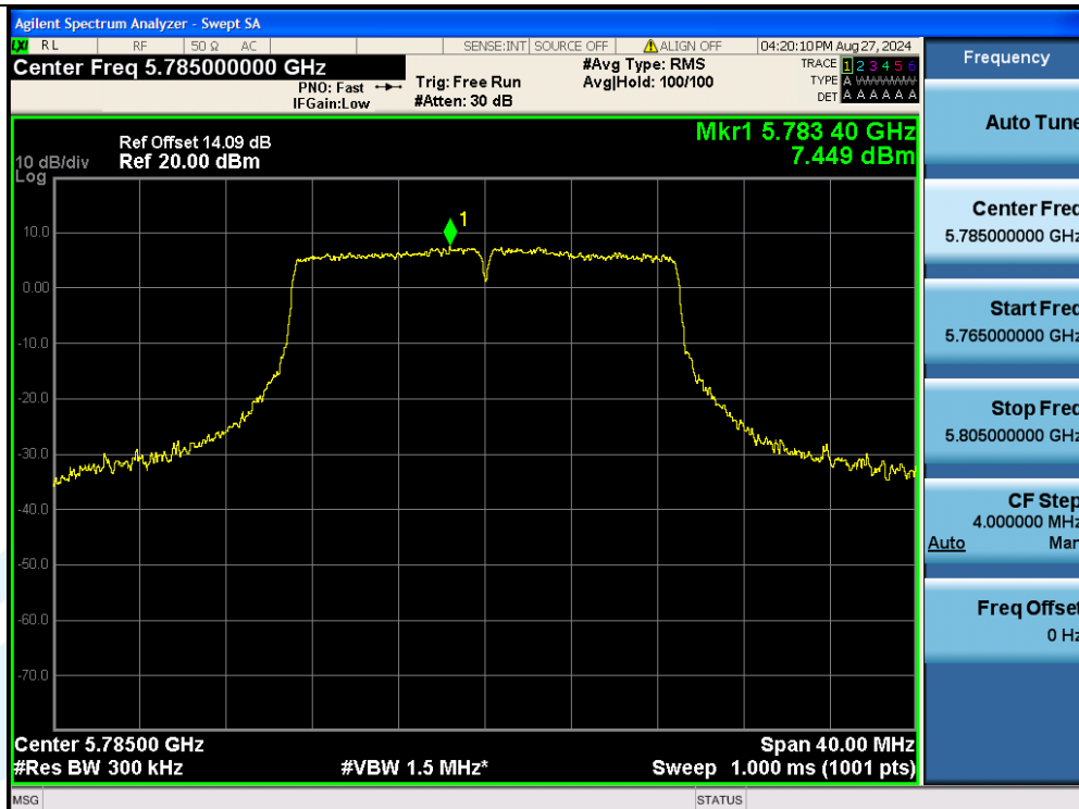
11AC20MIMO-Ant3-5785-PASS
