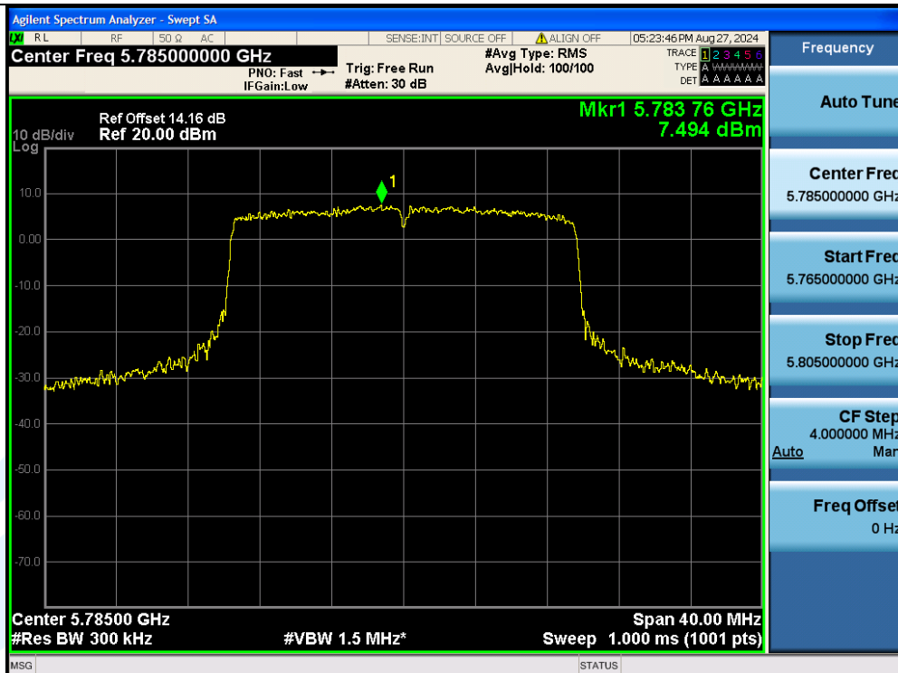
11AX20MIMO-Ant3-5785-PASS
