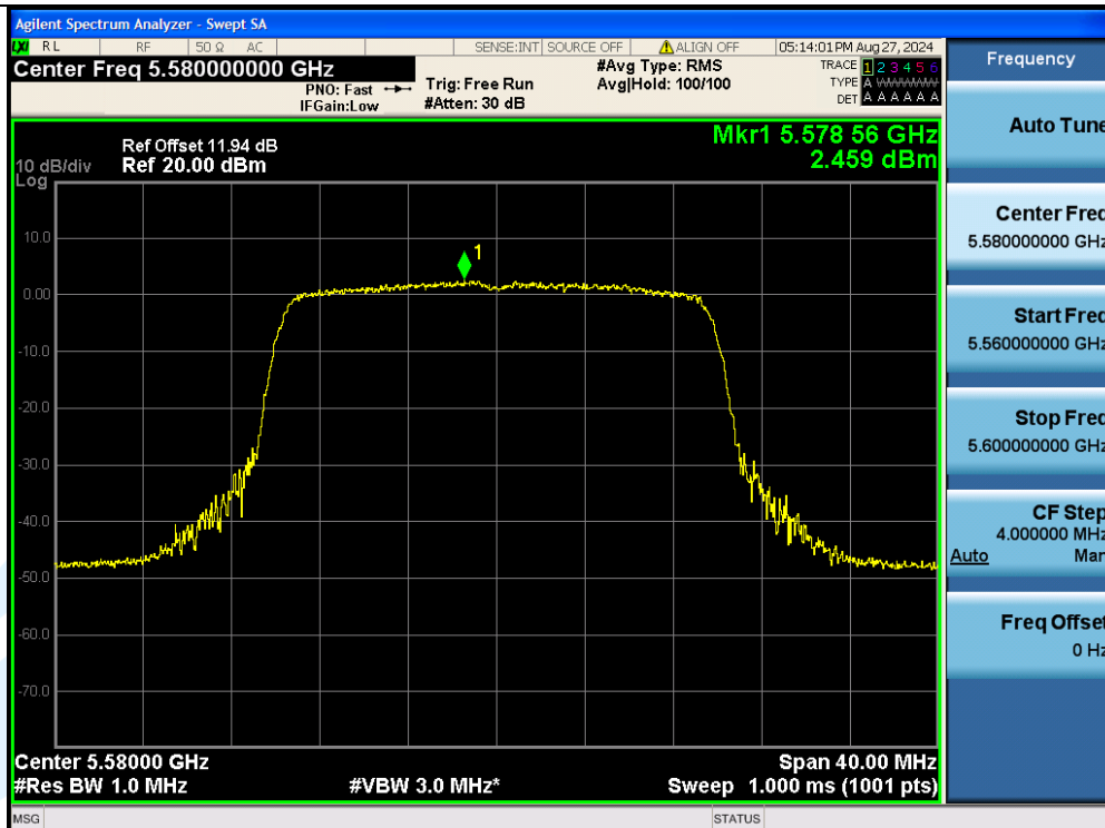
11AX20MIMO-Ant3-5580-PASS
