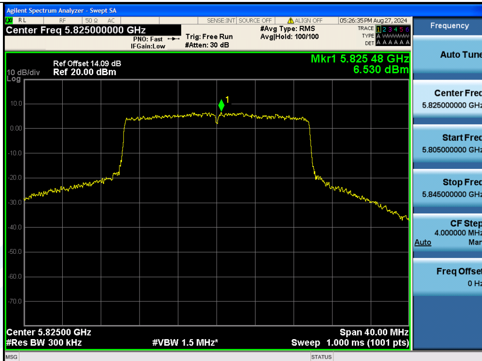
11AX20MIMO-Ant3-5825-PASS
