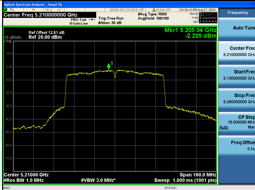
11AC80MIMO-Ant3-5210-PASS
