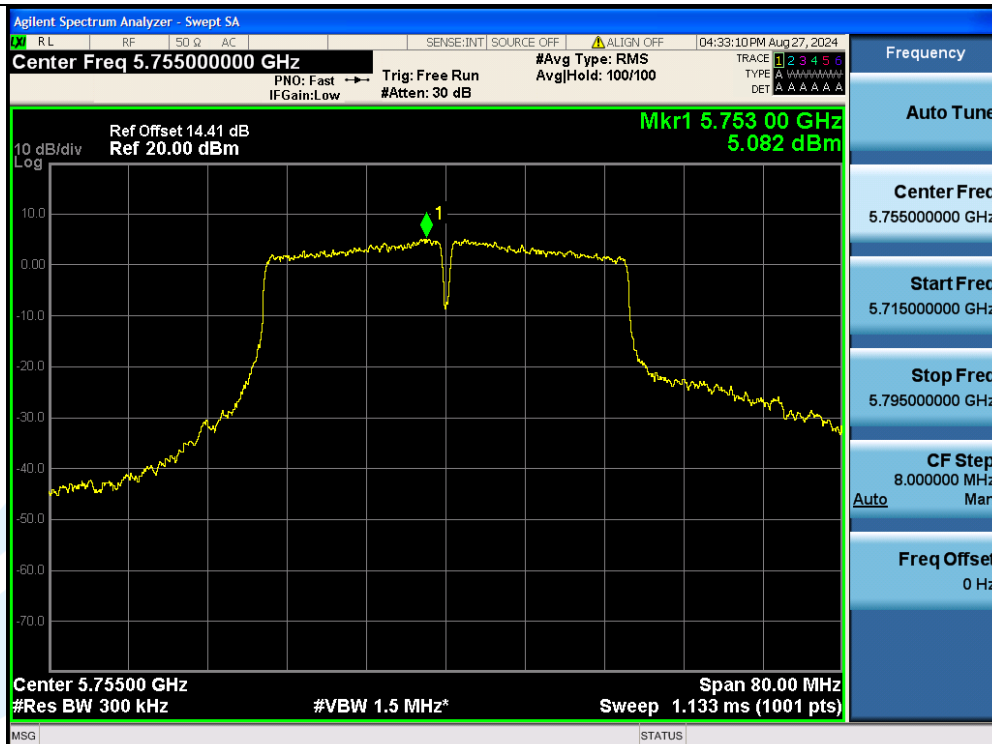
11AC40MIMO-Ant3-5755-PASS
