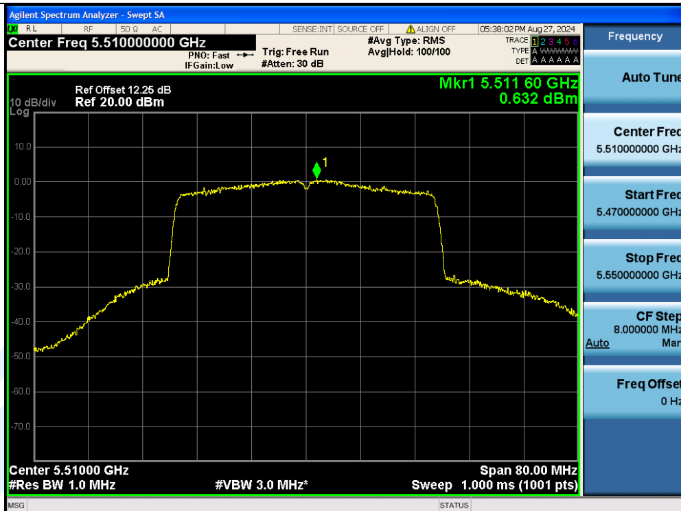
11AX40MIMO-Ant3-5510-PASS
