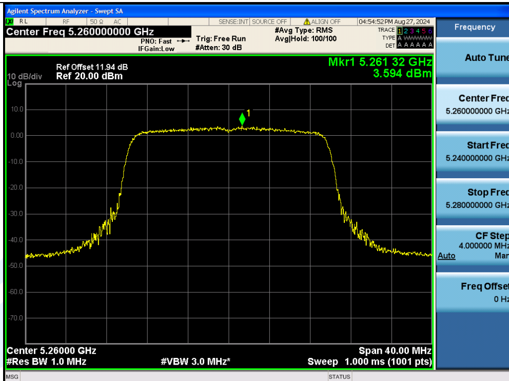
11AX20MIMO-Ant3-5260-PASS
