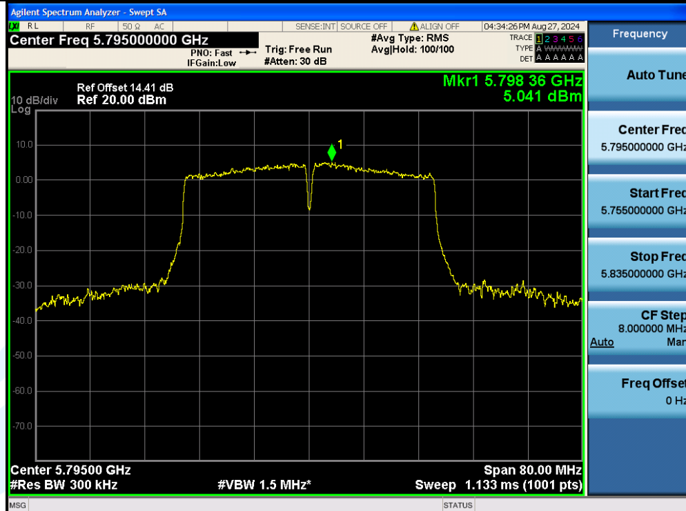
11AC40MIMO-Ant3-5795-PASS
