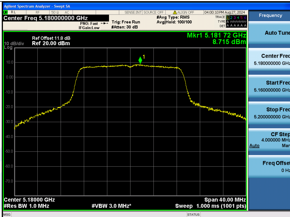
11AC20MIMO-Ant3-5180-PASS
