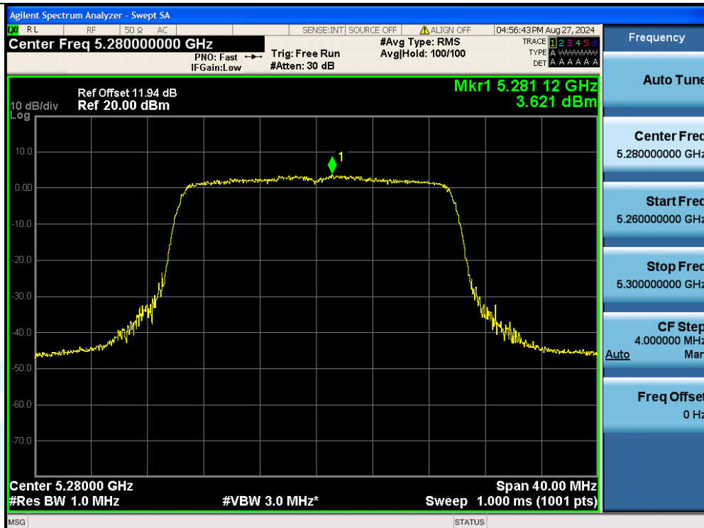
11AX20MIMO-Ant3-5280-PASS
