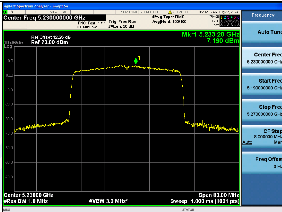
11AX40MIMO-Ant3-5230-PASS
