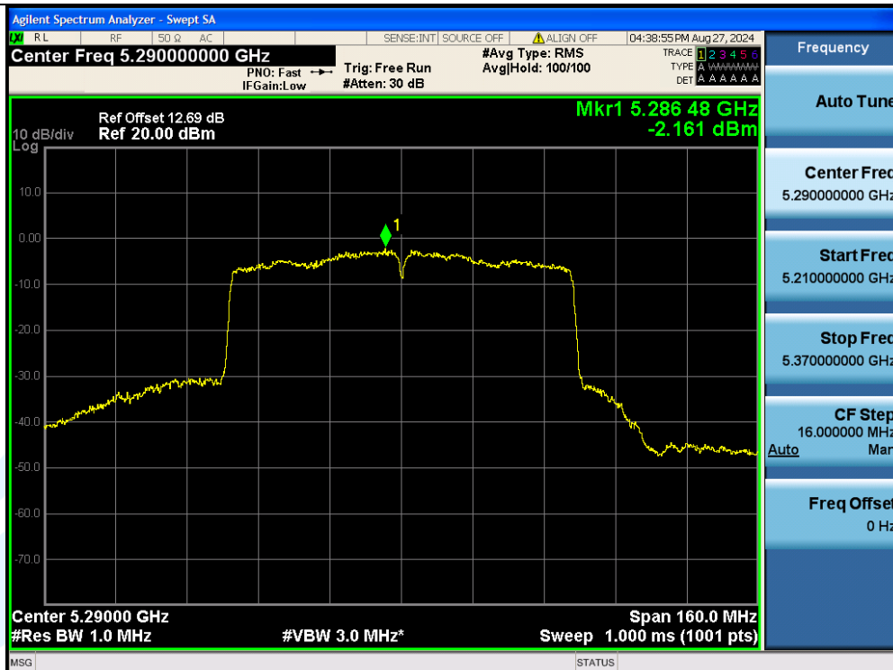
11AC80MIMO-Ant3-5290-PASS
