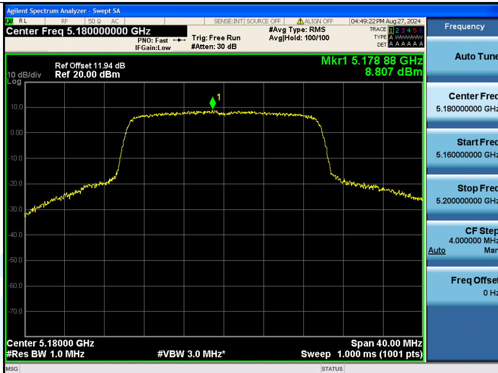
11AX20MIMO-Ant3-5180-PASS
