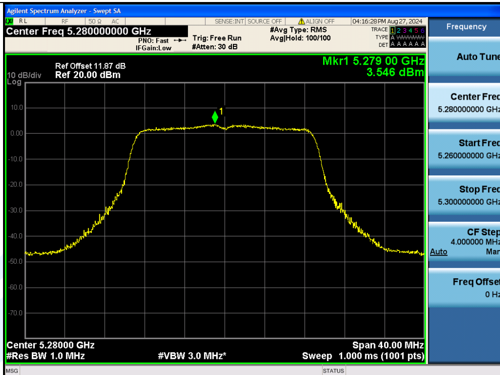
11AC20MIMO-Ant3-5280-PASS
