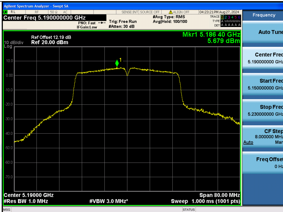
11AC40MIMO-Ant3-5190-PASS
