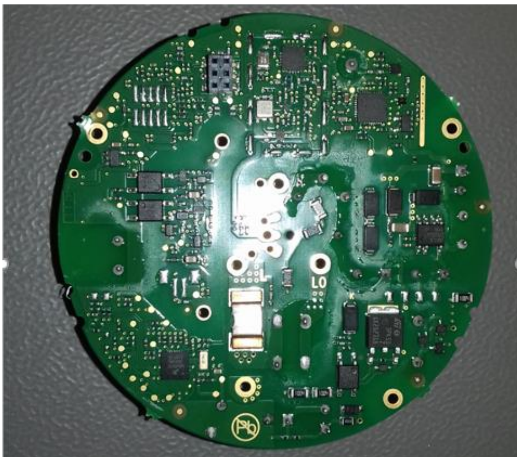
Figure 2 Main PCB bottom RF screening enclosure and varistor removed
