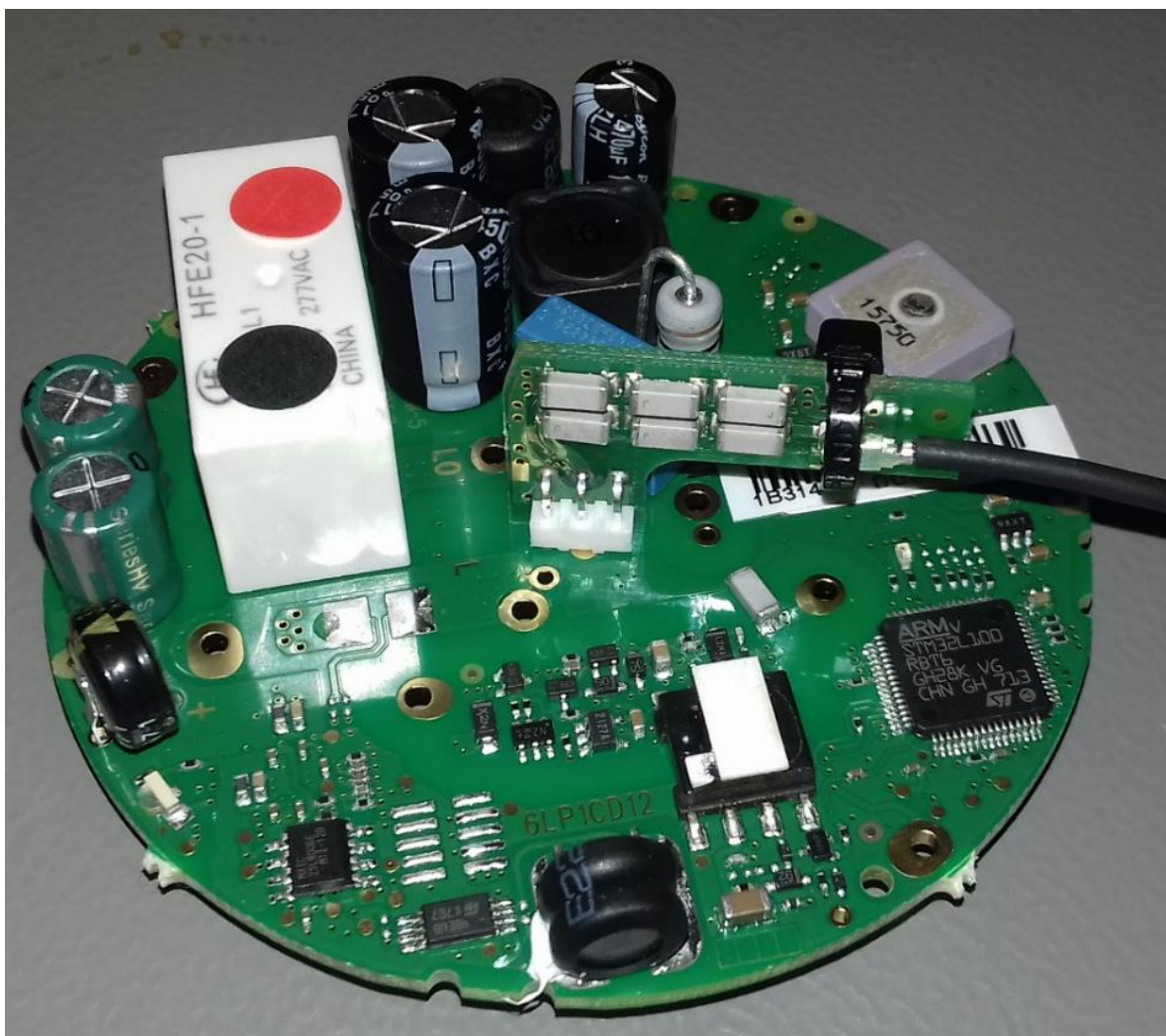
Figure 4 Main PCB top with antenna isolator fitted
