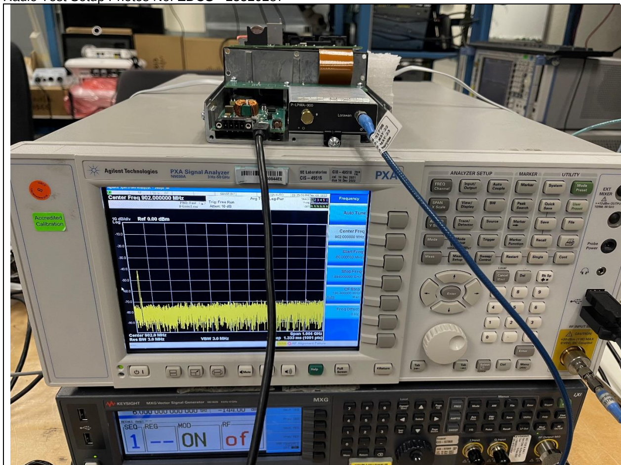
Radio Test Setup Photos No: EDCS - 23320287
