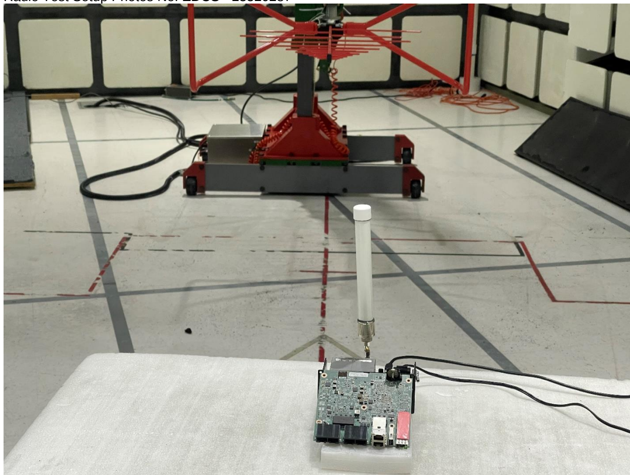
Title: Radiated Spurious Emissions Test Configuration 30M - 1000MHz (1.5dBi antenna gain)
